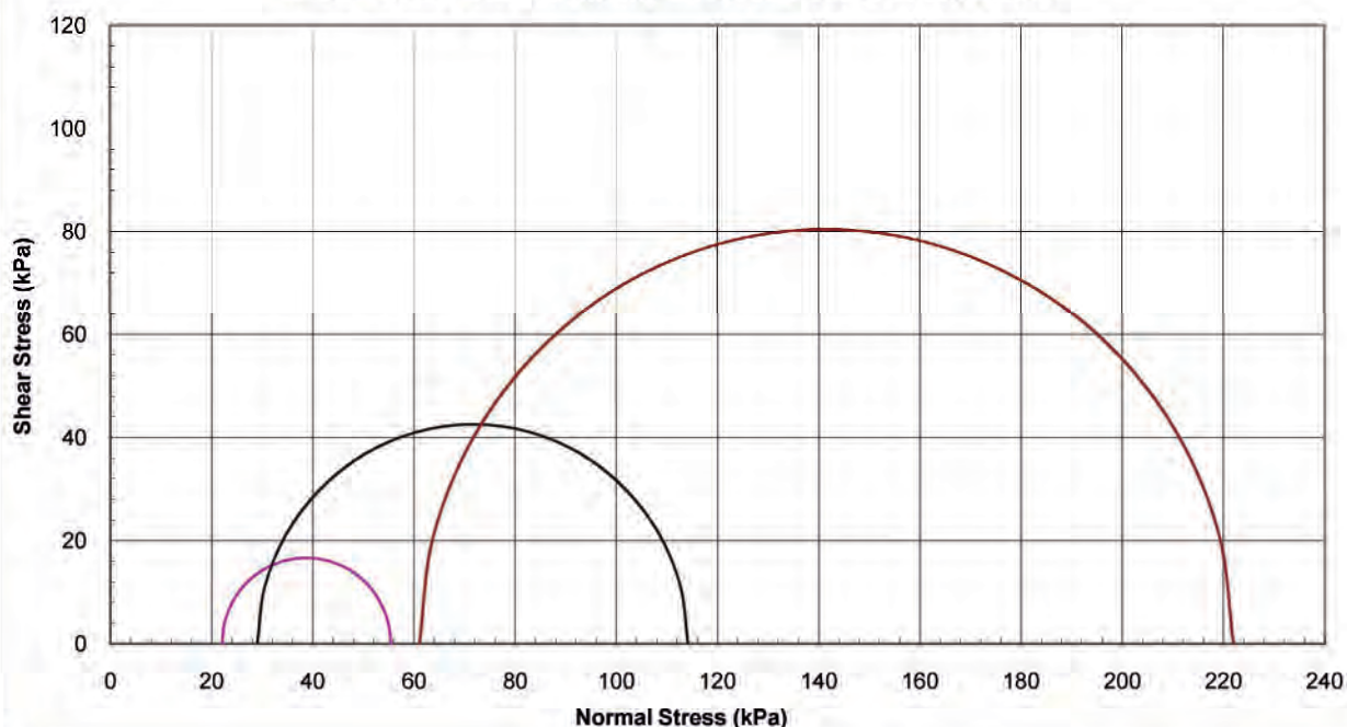
Mohr Circles and the Mohr Envelope Representing Failure
