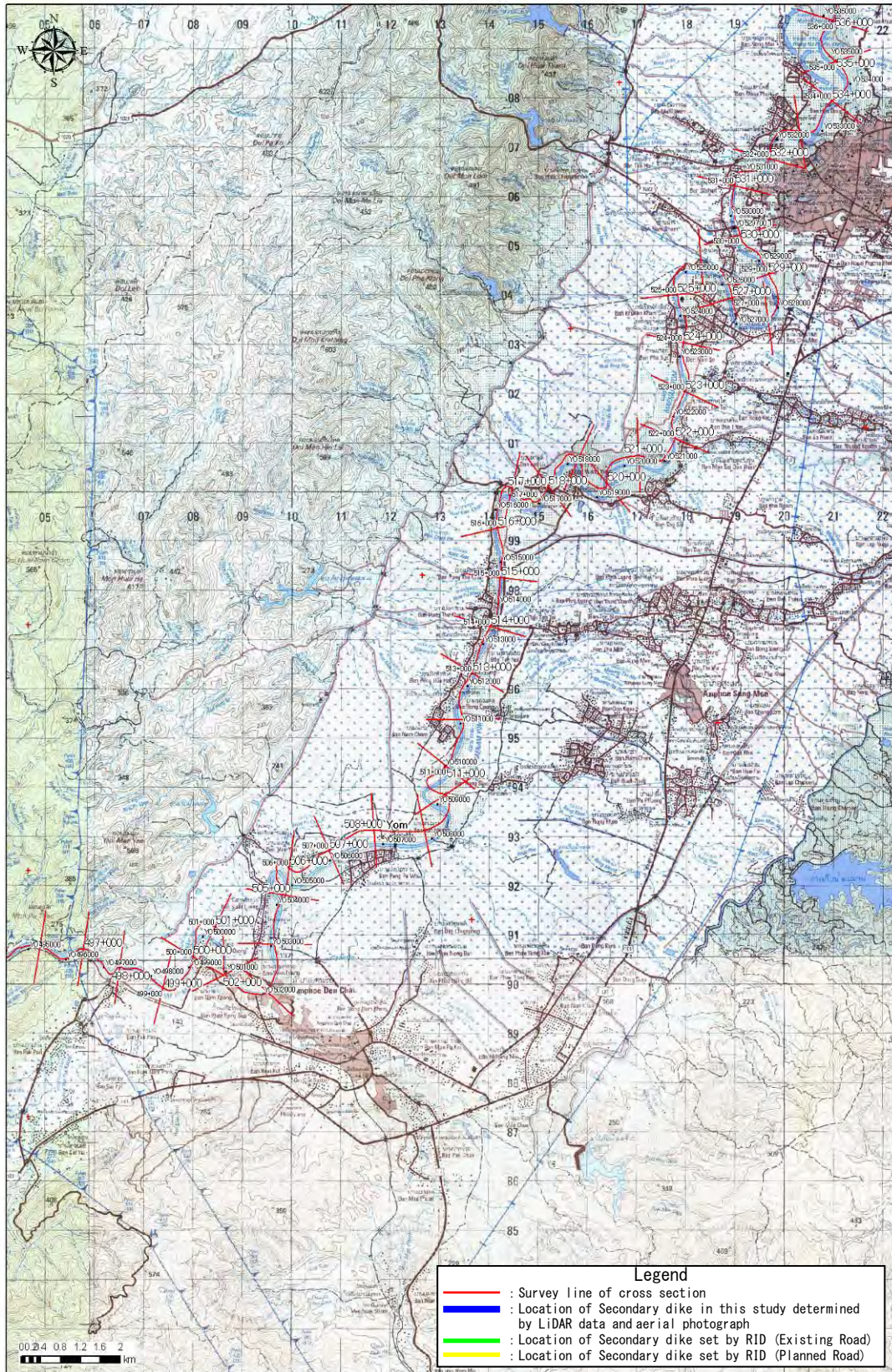
Figure D1.1.65 Location of Cross-section & Secondary dike (63)
