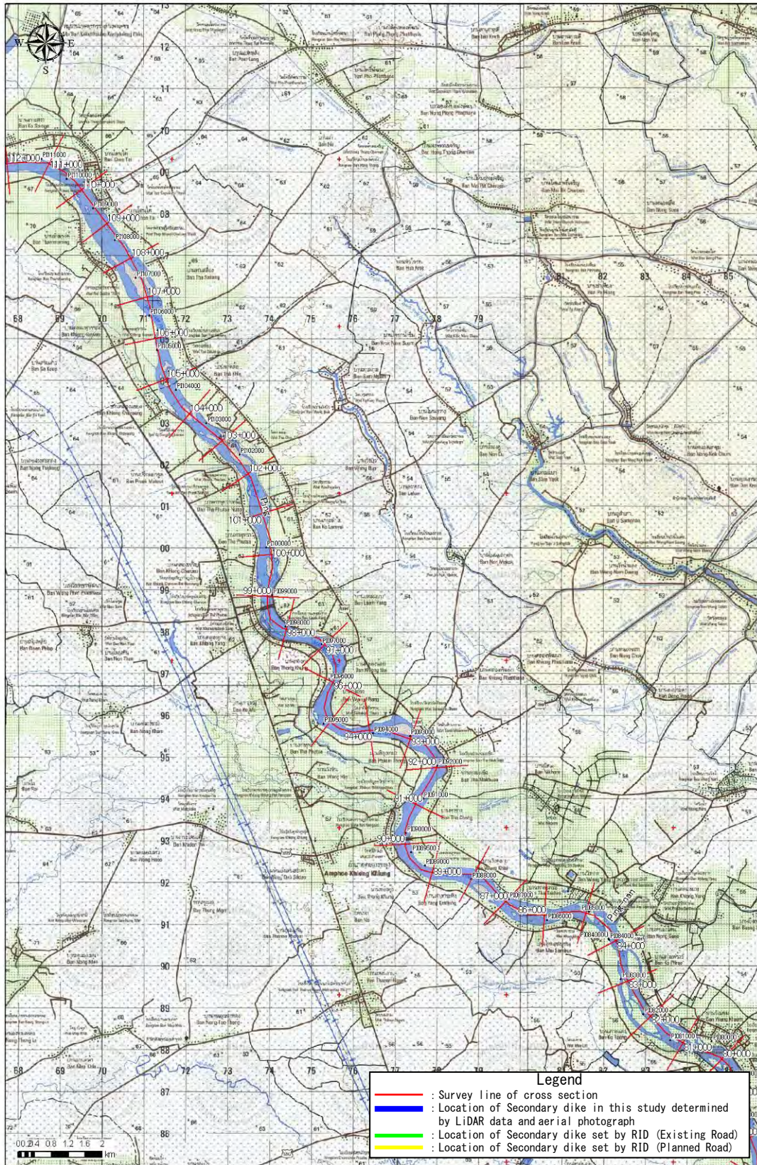
Figure D1.1.71 Location of Cross-section & Secondary dike (69)
