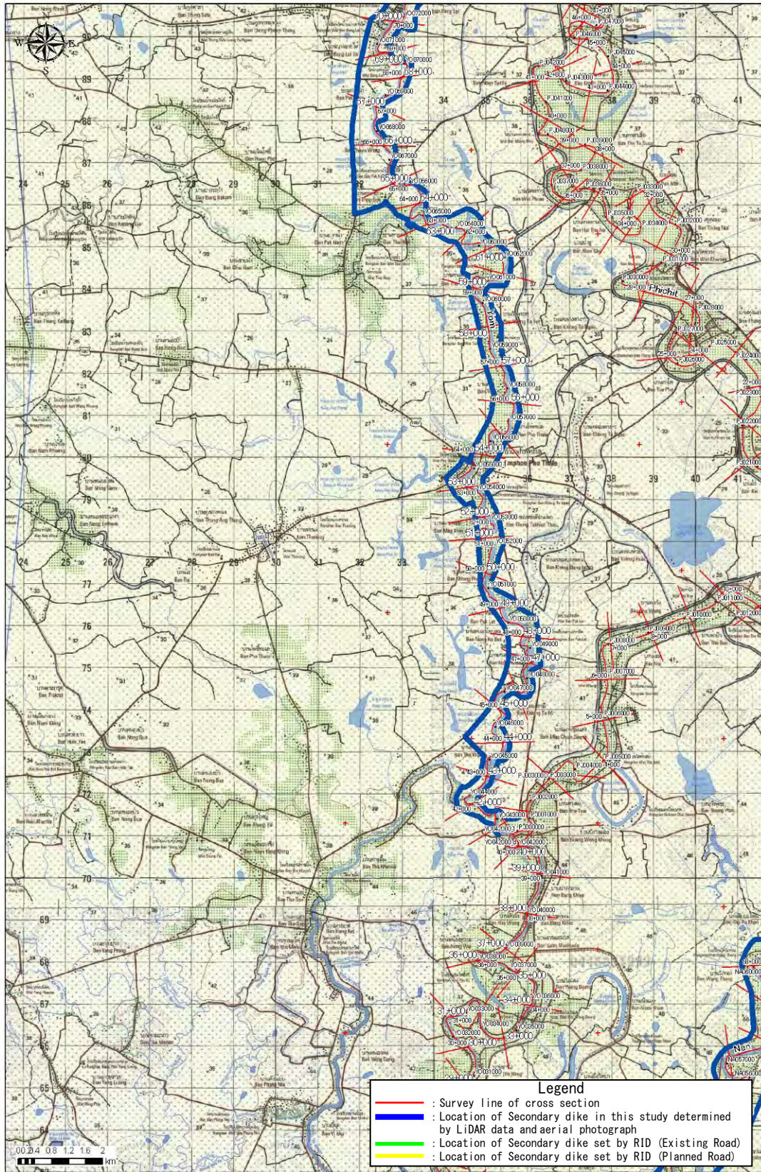
Figure D1.1.53 Location of Cross-section & Secondary dike (51)
