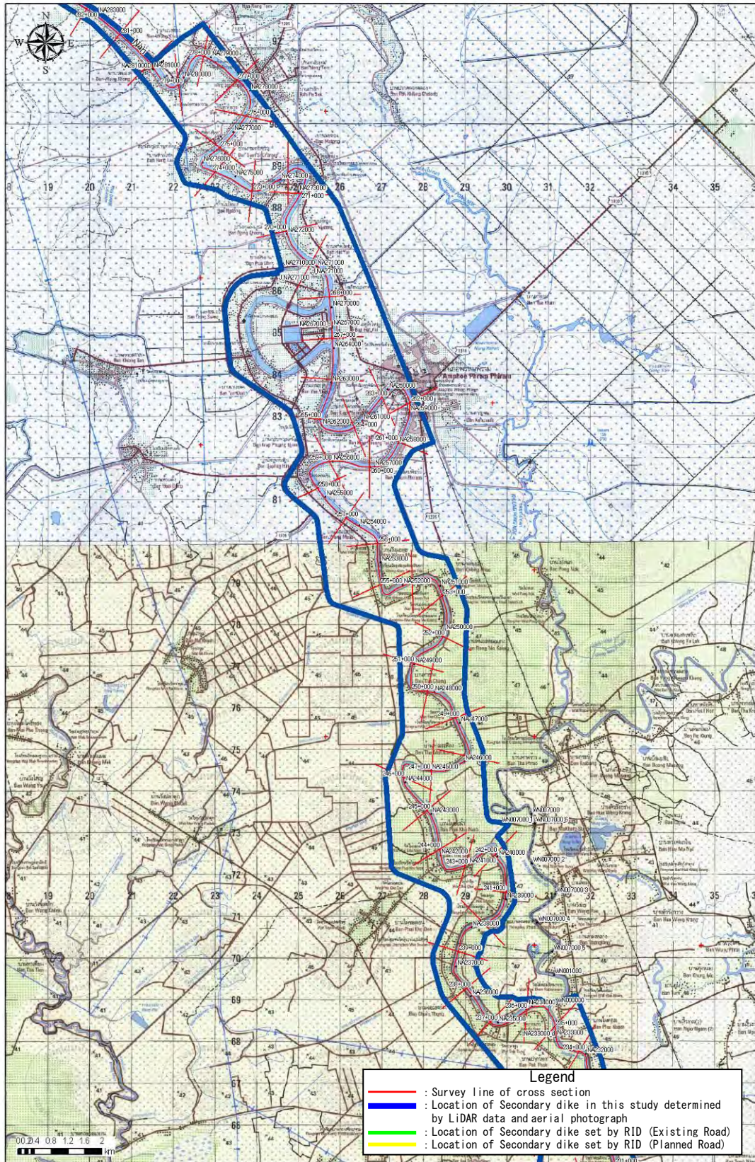
Figure D1.1.45 Location of Cross-section & Secondary dike (43)
