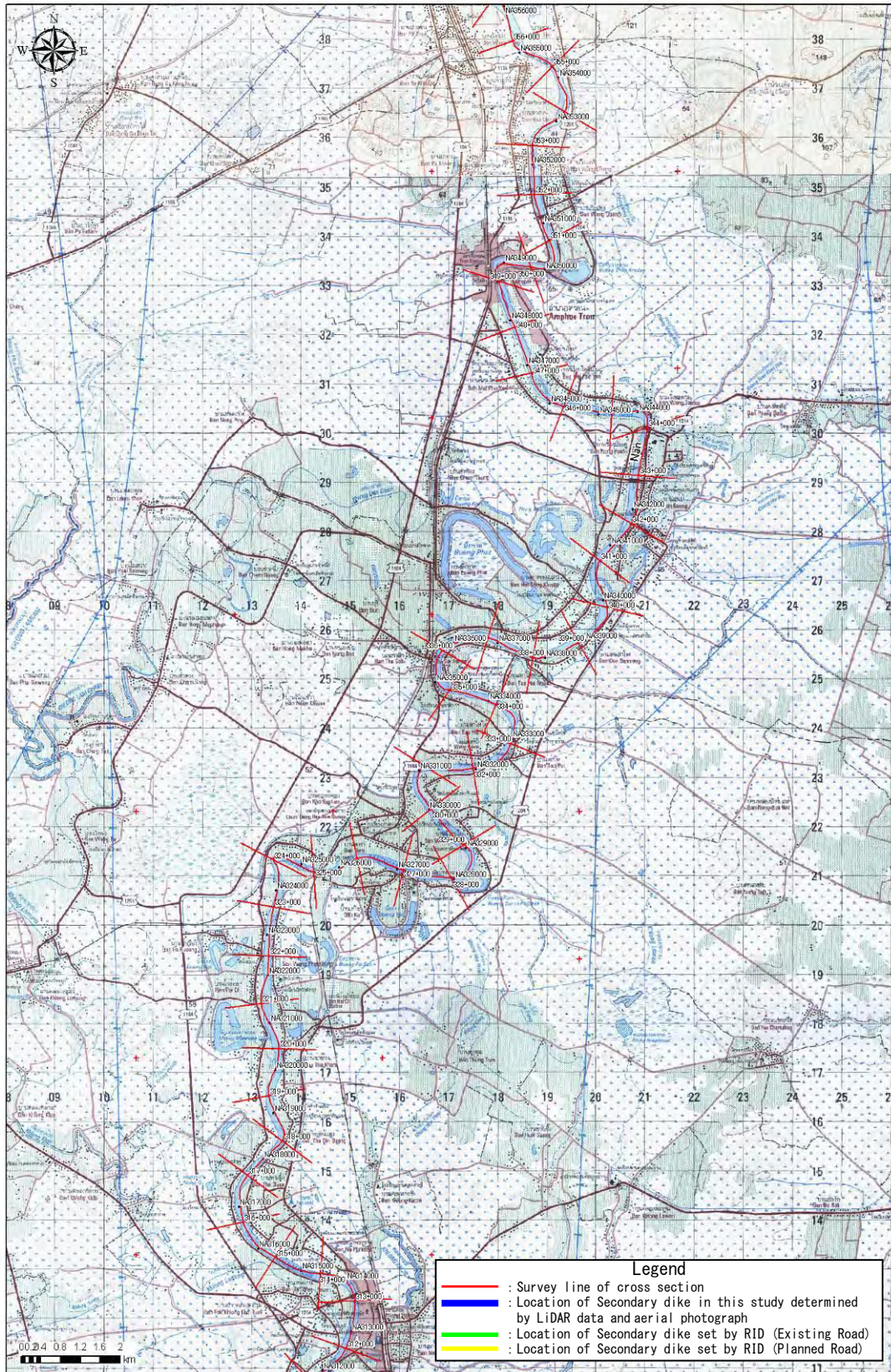
Figure D1.1.47 Location of Cross-section & Secondary dike (45)
