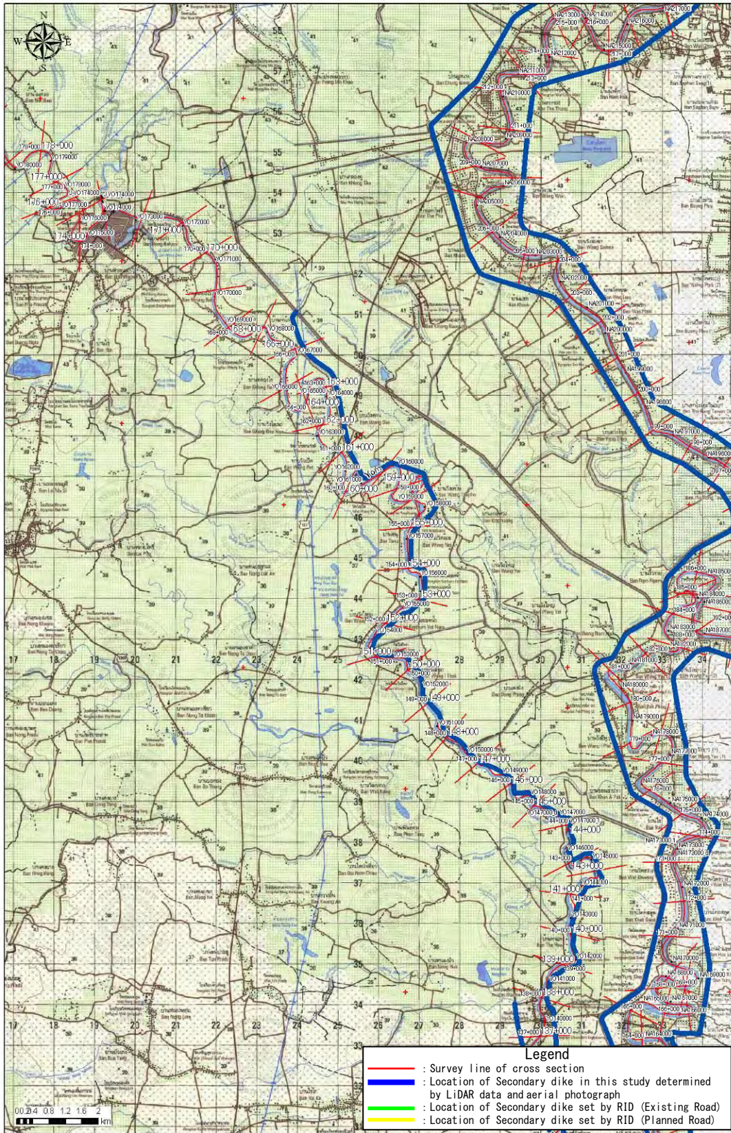
Figure D1.1.56 Location of Cross-section & Secondary dike (54)
