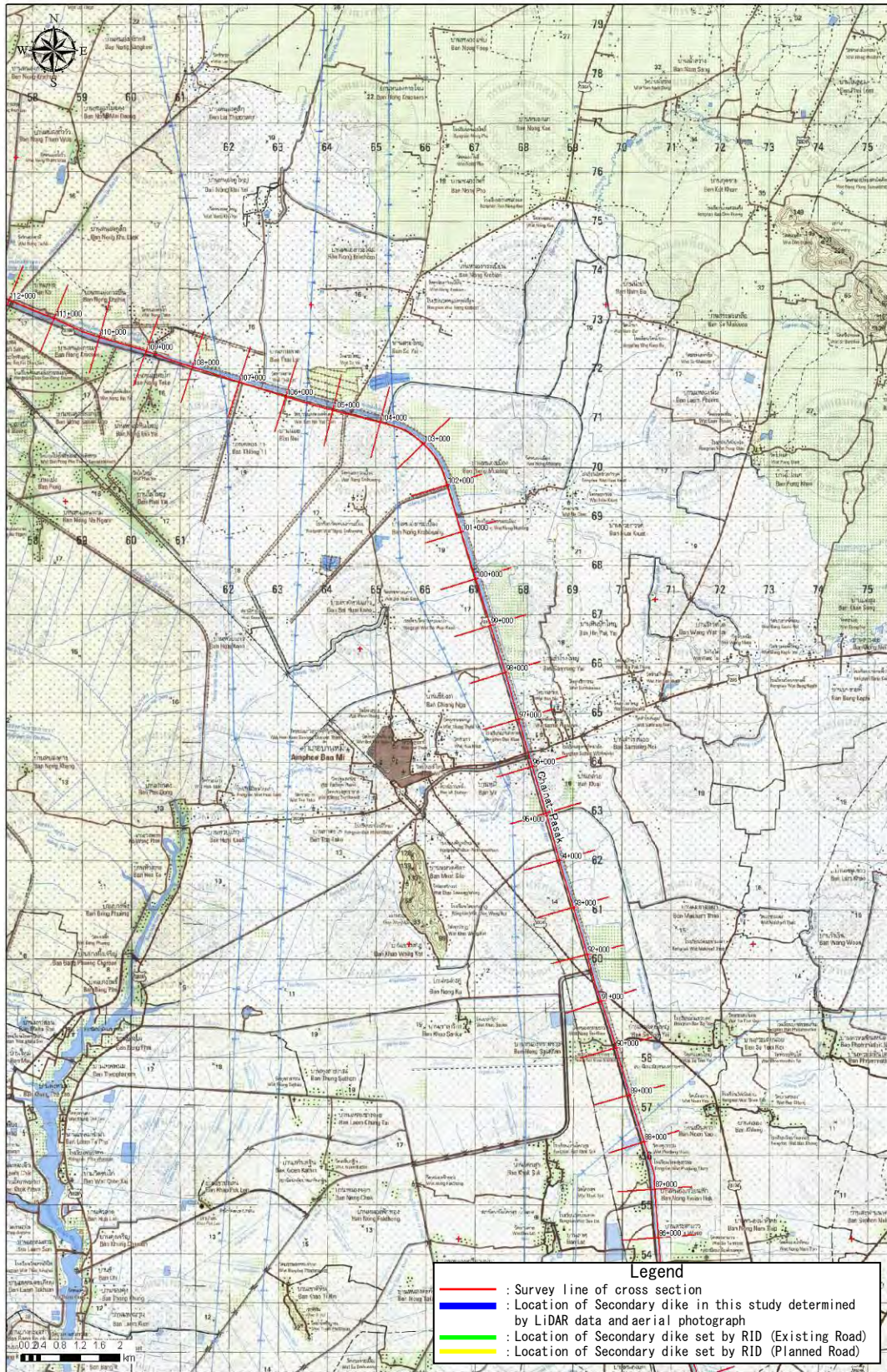
Figure D1.1.30 Location of Cross-section & Secondary dike (28)
