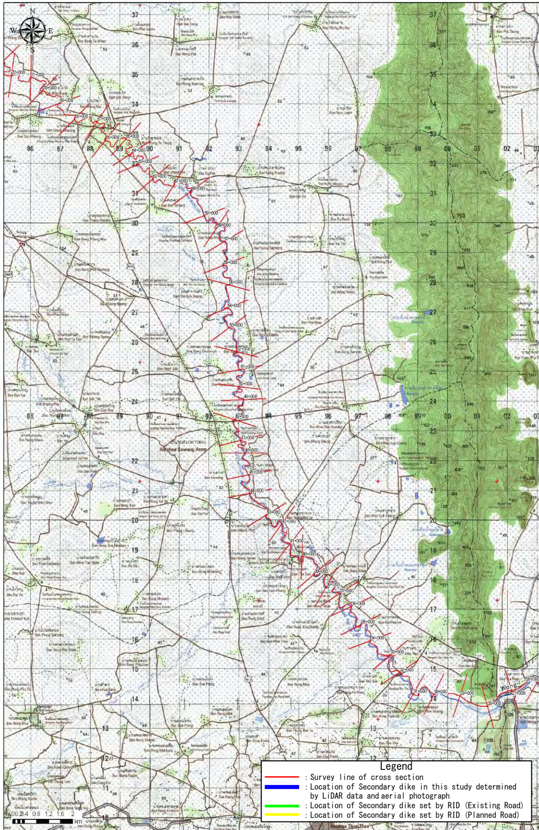
Figure D1.1.35 Location of Cross-section & Secondary dike (33)
