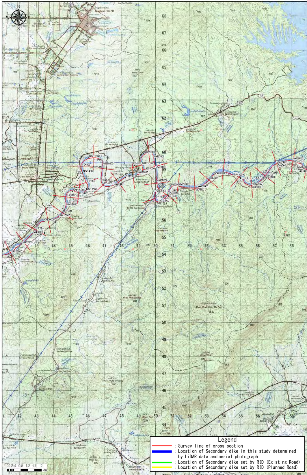
Figure D1.1.50 Location of Cross-section & Secondary dike (48)
