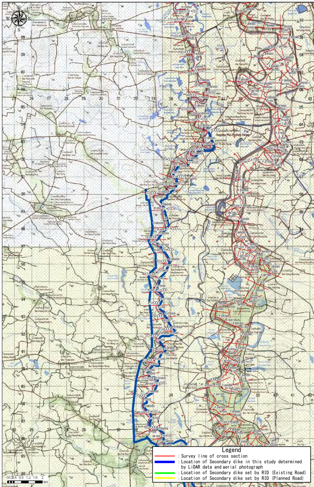
Figure D1.1.54 Location of Cross-section & Secondary dike (52)
