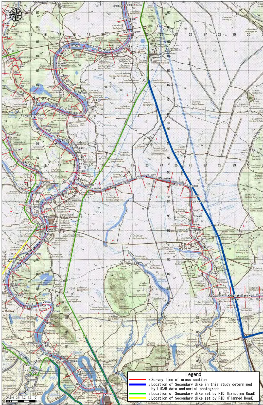
Figure D1.1.33 Location of Cross-section & Secondary dike (31)
