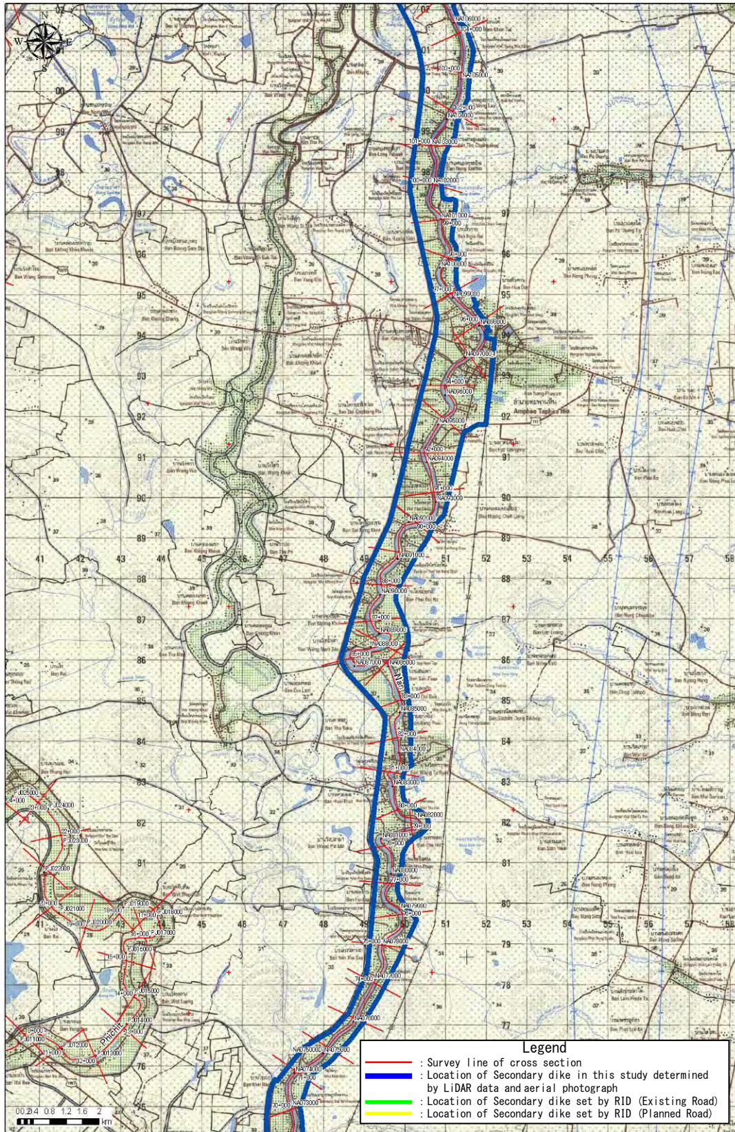
Figure D1.1.41 Location of Cross-section & Secondary dike (39)
