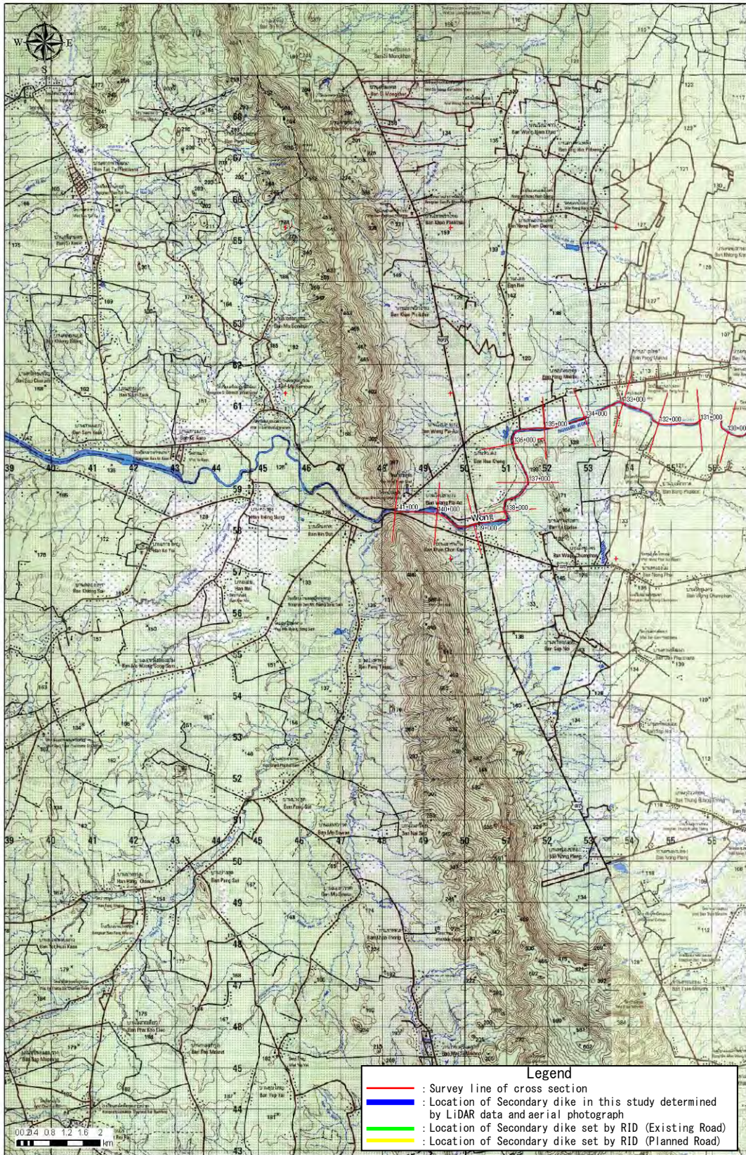
Figure D1.1.38 Location of Cross-section & Secondary dike (36)
