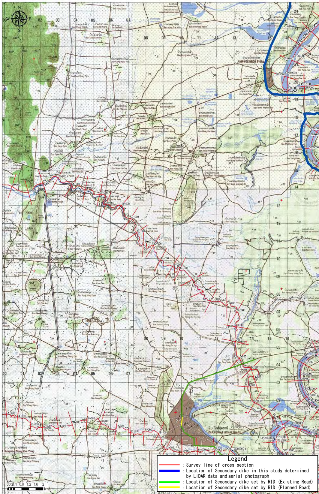
Figure D1.1.34 Location of Cross-section & Secondary dike (32)
