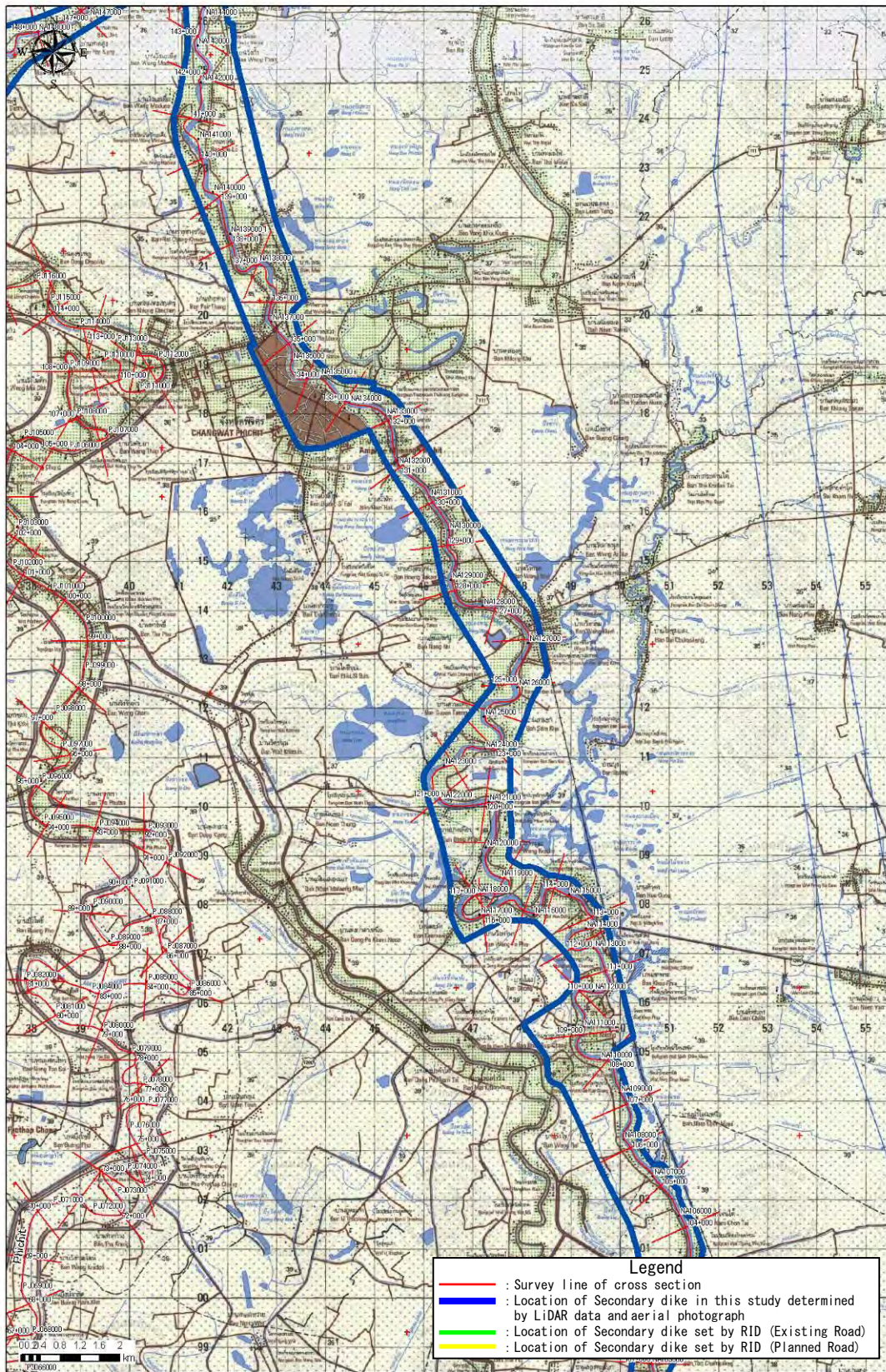
Figure D1.1.42 Location of Cross-section & Secondary dike (40)
