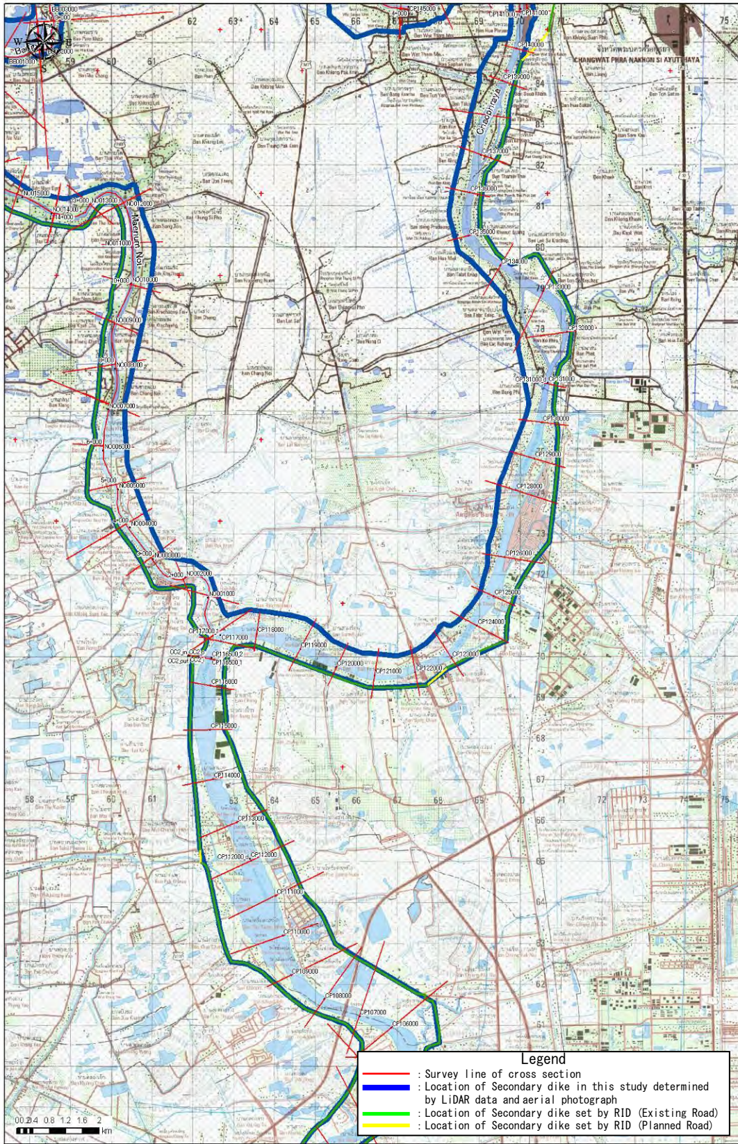
Figure D1.1.6 Location of Cross-section & Secondary dike (4)
