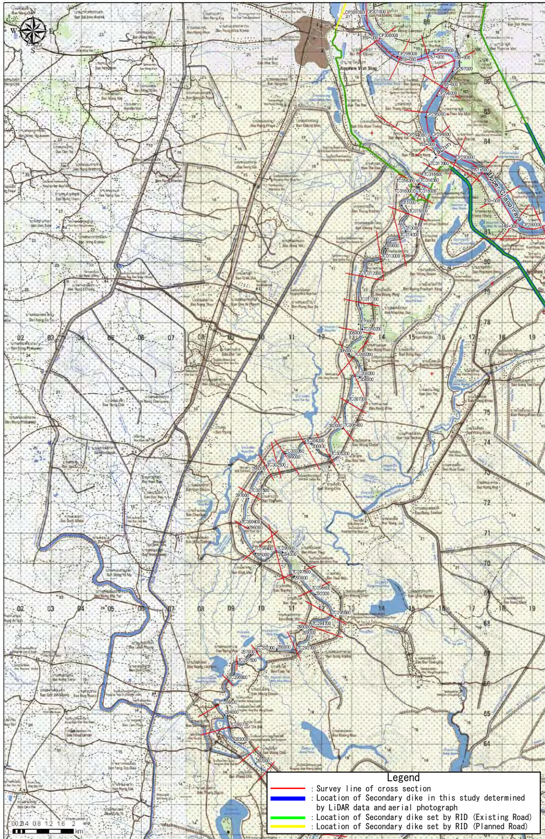
Figure D1.1.21 Location of Cross-section & Secondary dike (19)
