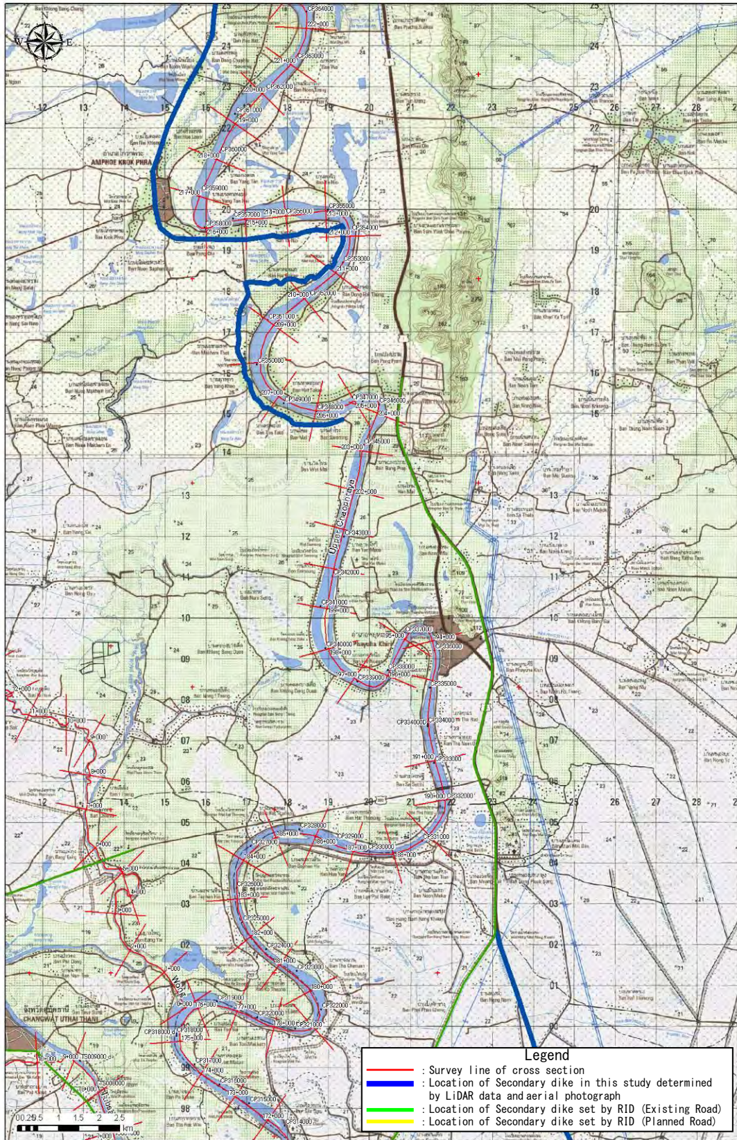
Figure D1.1.12 Location of Cross-section & Secondary dike (10)
