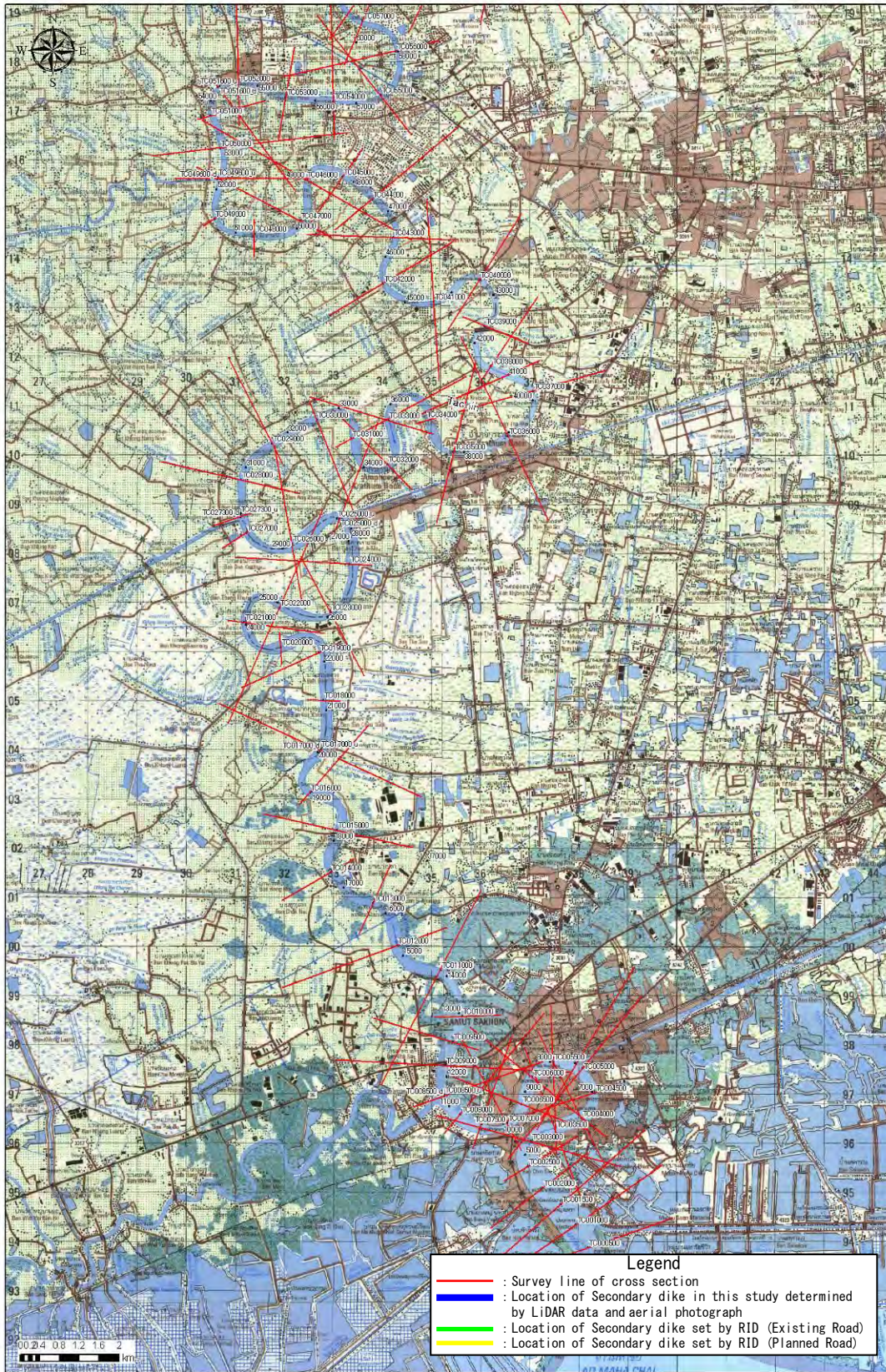
Figure D1.1.14 Location of Cross-section & Secondary dike (12)
