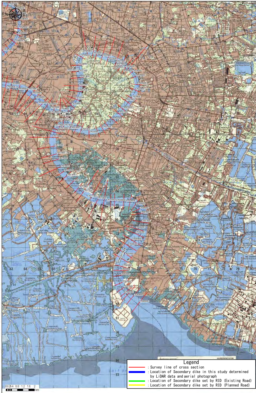
Figure D1.1.3 Location of Cross-section & Secondary dike (1)
