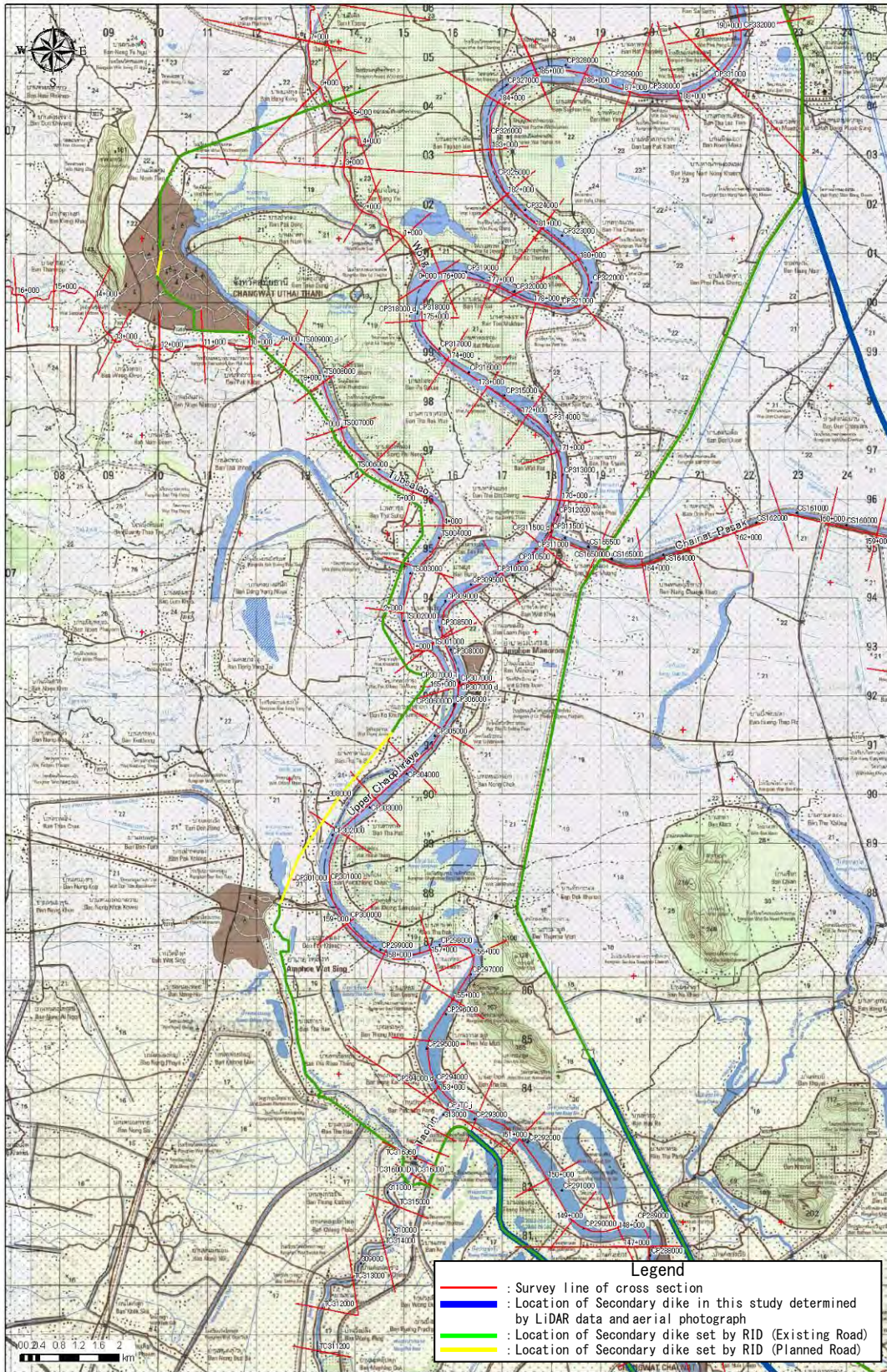
Figure D1.1.22 Location of Cross-section & Secondary dike (20)
