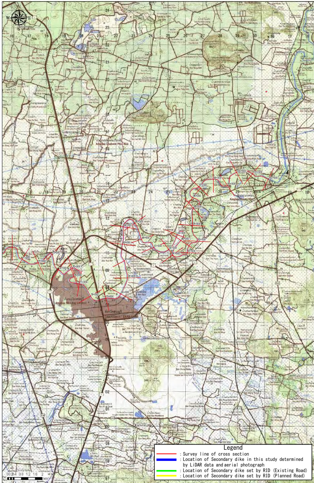
Figure D1.1.25 Location of Cross-section & Secondary dike (23)
