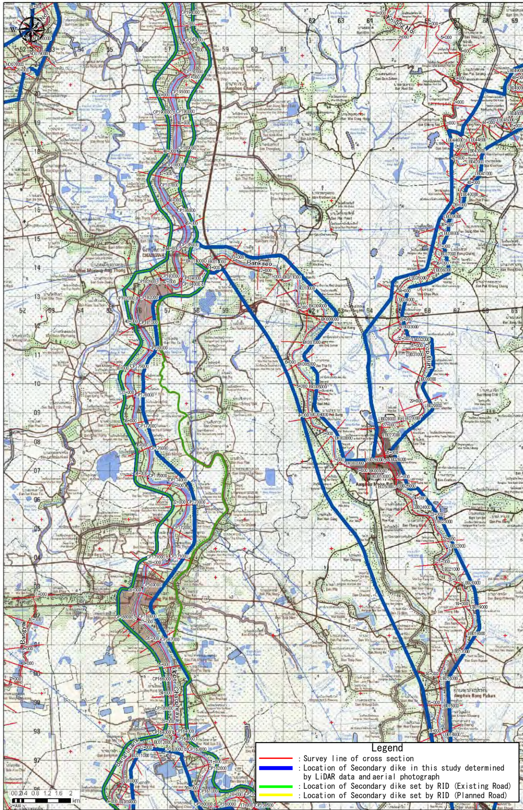
Figure D1.1.26 Location of Cross-section & Secondary dike (24)
