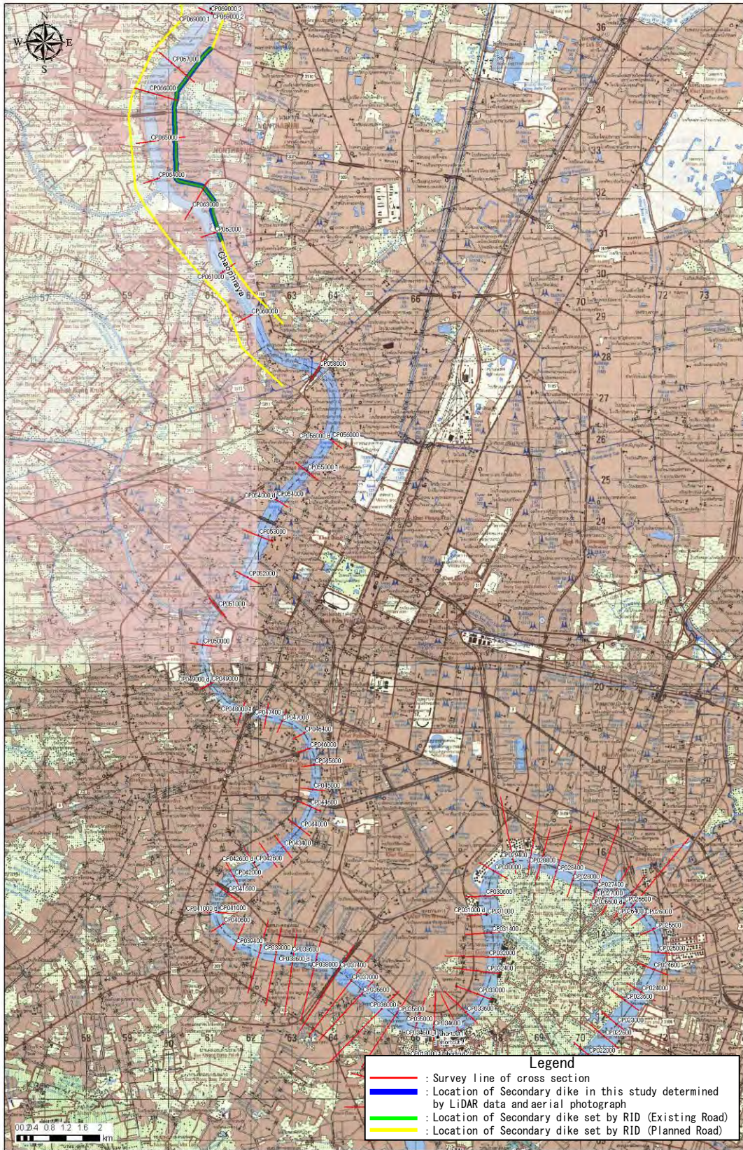
Figure D1.1.4 Location of Cross-section & Secondary dike (2)
