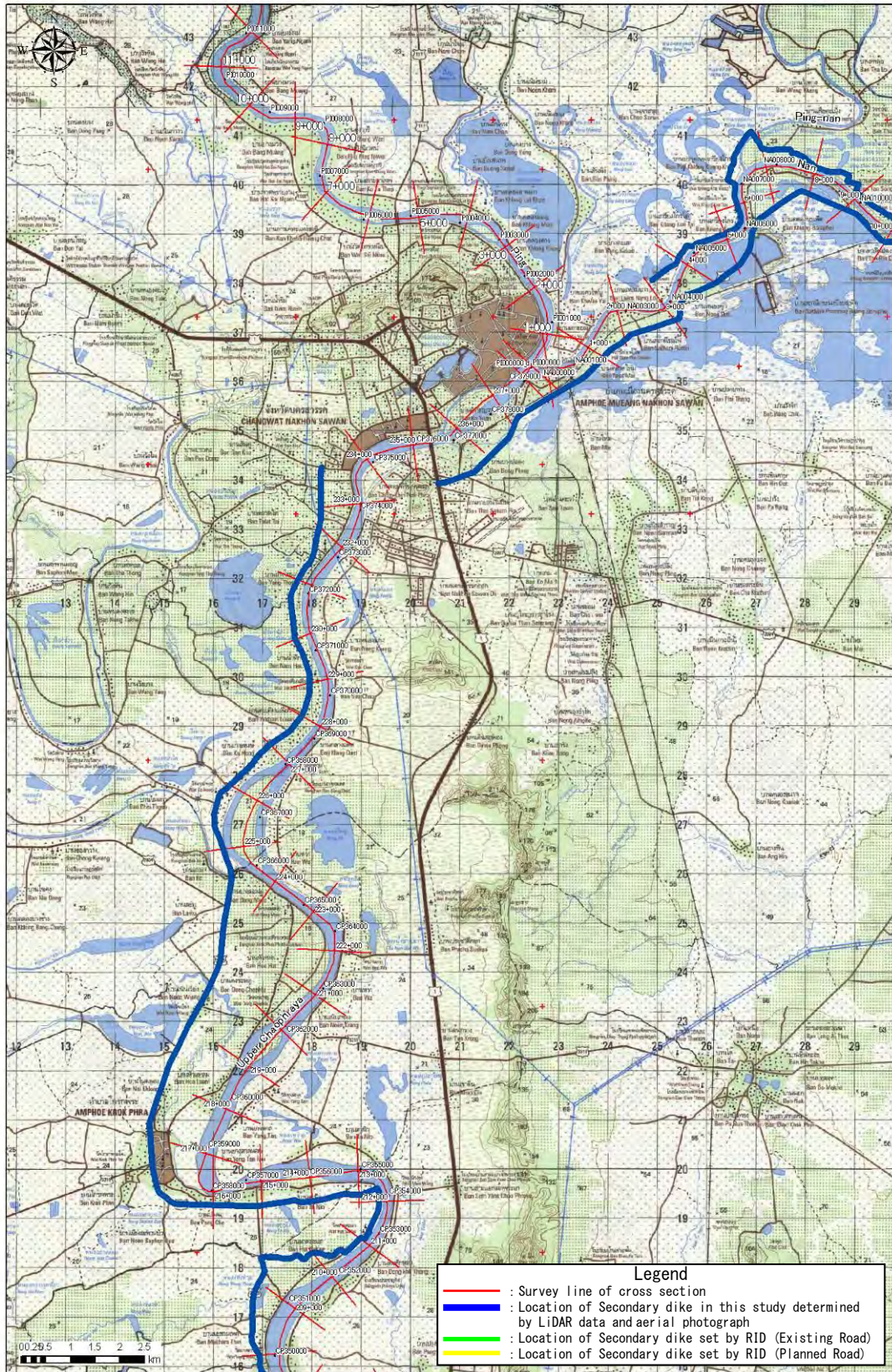
Figure D1.1.13 Location of Cross-section & Secondary dike (11)
