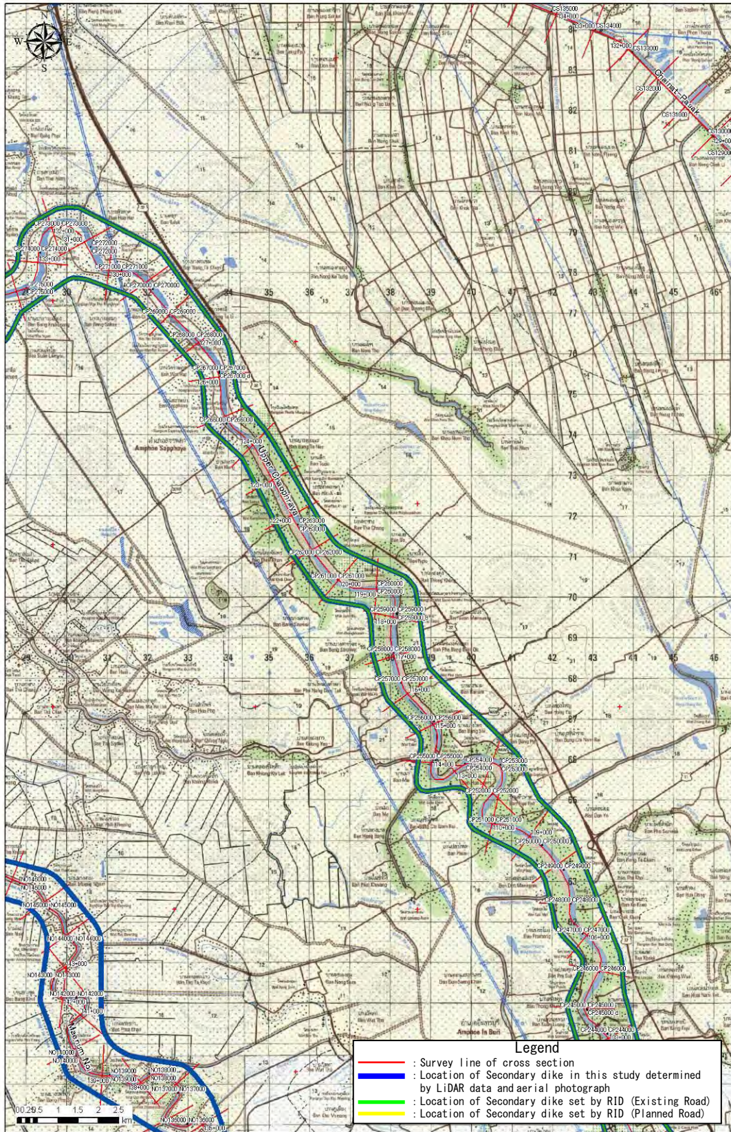
Figure D1.1.10 Location of Cross-section & Secondary dike (8)
