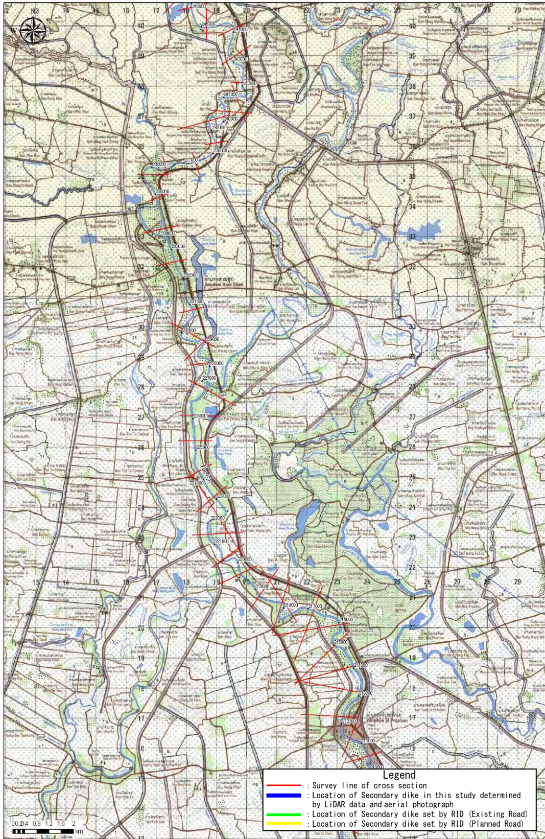
Figure D1.1.19 Location of Cross-section & Secondary dike (17)
