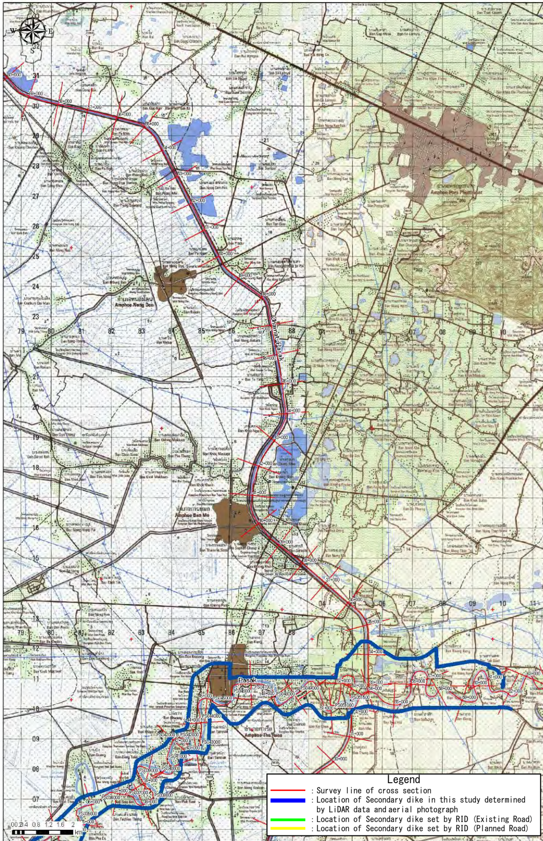
Figure D1.1.28 Location of Cross-section & Secondary dike (26)
