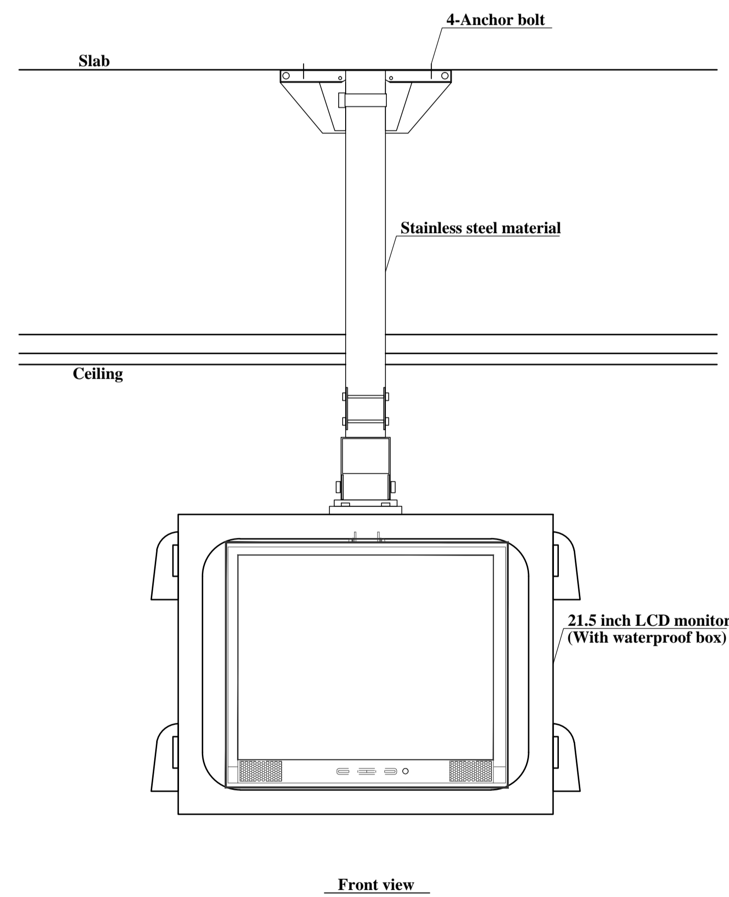
21.5 inch LCD monitor ceiling mounted (Driver's lounge) S=1/10
