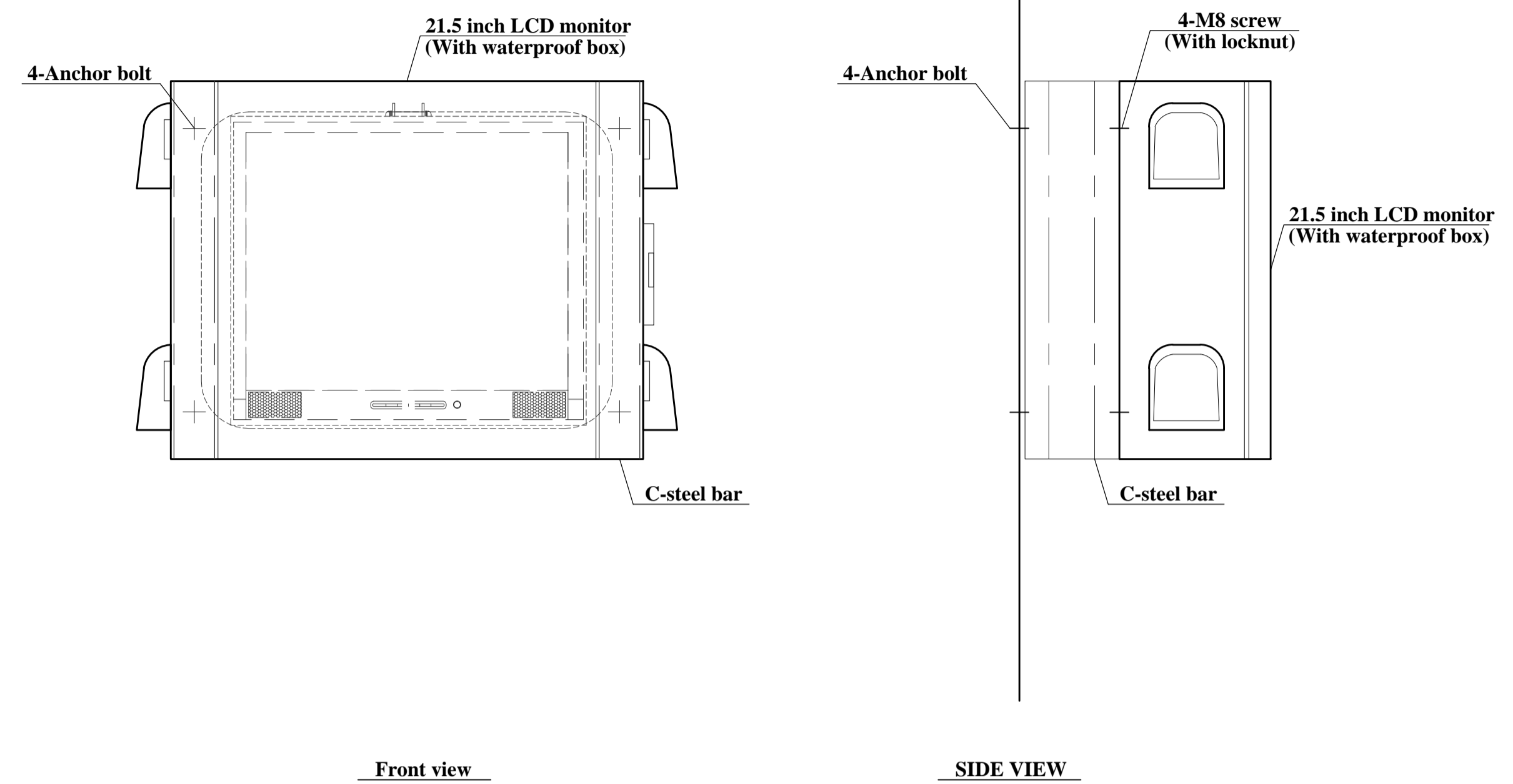
21.5 inch LCD monitor wall mounted (Baggage breakdown & Make-Up area) S=1/10
