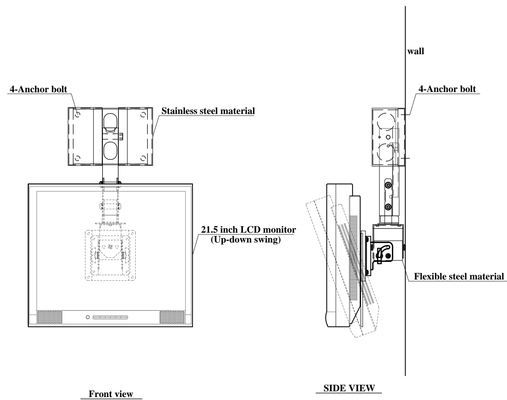
21.5 inch LCD monitor wall mounted (Vertical swing) S=1/10
