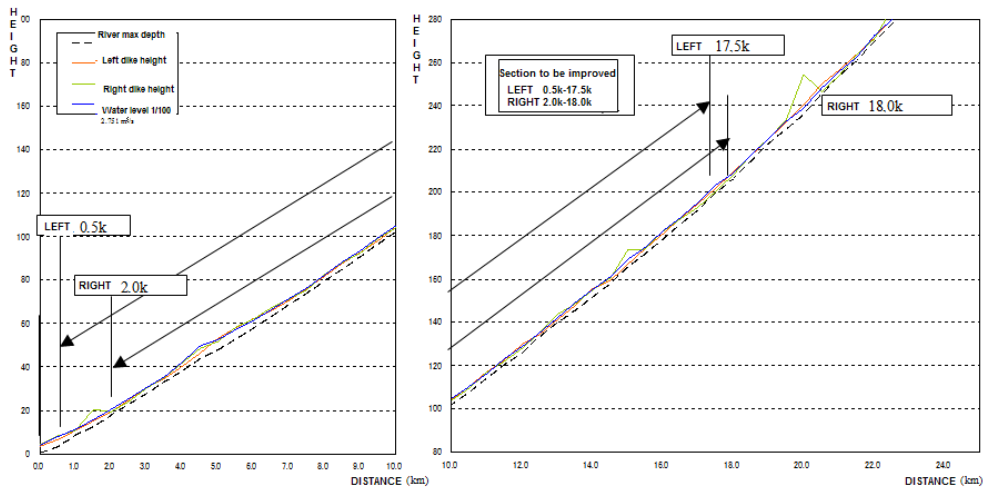
Figure 4.12.1-3 Chincha River Longitudinal Profile (Chico River)
