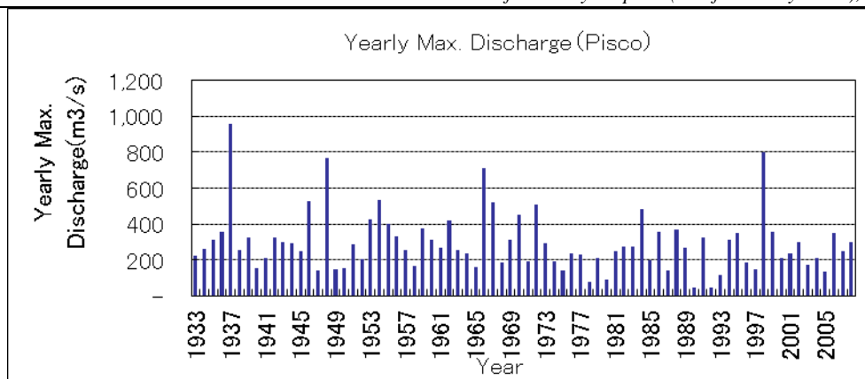
Figure- 4.3.1-1 Yearly Max. Discharge (Pisco)
