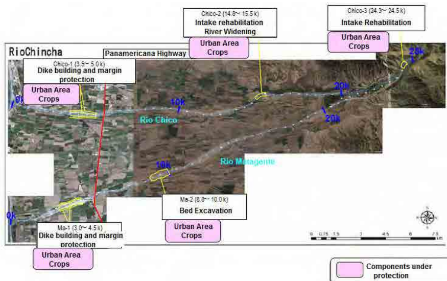
Figure 4.3.1-5 Priority Works on flood control in the Chincha River
