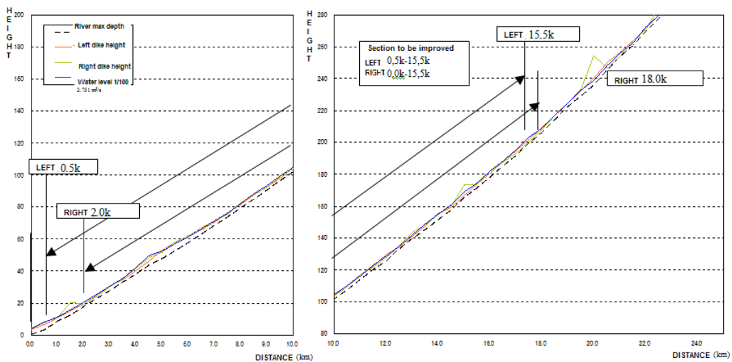
Figure 4.12.1-4 Chincha River Longitudinal Profile (Matagente River)
