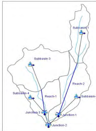
Figure-3.1.9.4-2 Schematic diagrams in HEC-HMS
