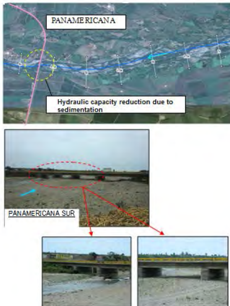
Figure 3.1.6-4 Local conditions related with Challenge 3 (Cañete river)
