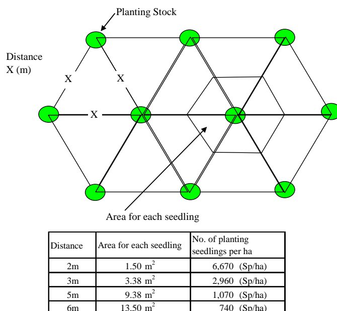
Figure 3.5 Layout of Planting Points (Forestation in Upper Stream)
