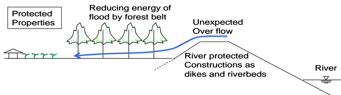
Figure 3.1 Conceptual Diagram of Riparian Forestation Plan (Type A)
