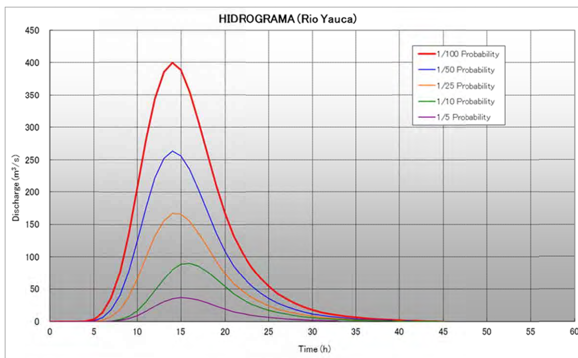
Figure 2.9 Probable Flood Hydrographs (Yauca River)
