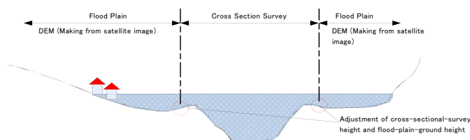
Figure 1.1 Image of One-Dimensional Analysis Model
