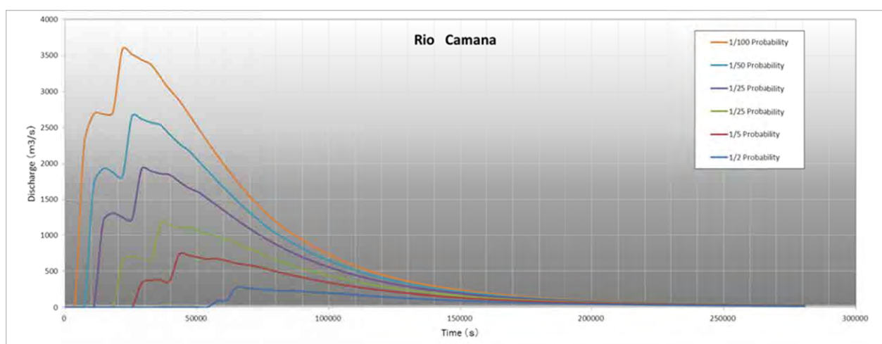
Figure 2.11 Probable Flood Hydrographs (Majes-Camana River)
