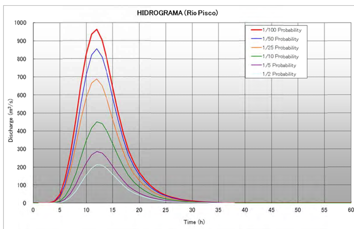
Figure 2.7 Probable Flood Hydrographs (Pisco River)
