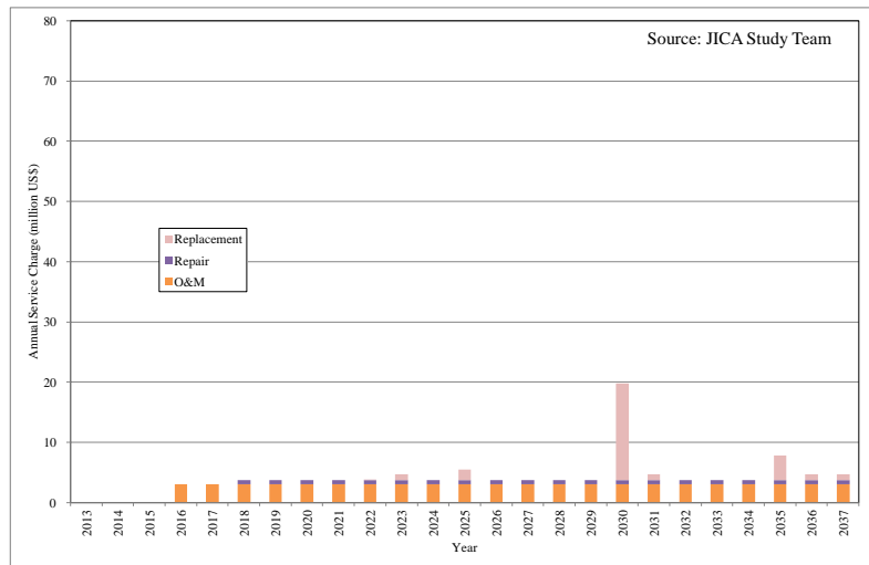
Figure 4.6.4 JC Expenditure for O&M/Repair/Replacement of Phu Do WWTP
