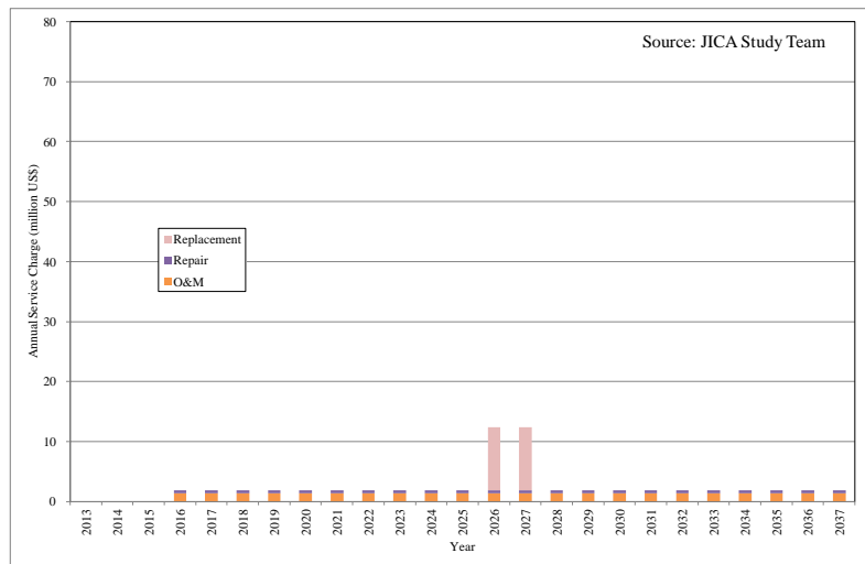
Figure 4.6.6 JC Expenditure for O&M/Repair/Replacement for Yen So BPC
