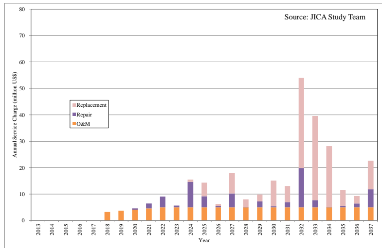
Figure 4.6.5 JC Expenditure for O&M/Repair/Replacement of Yen Xa WWTP
