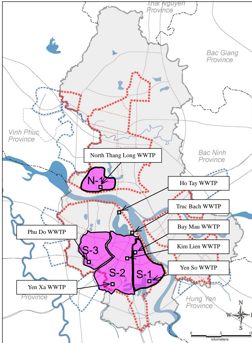
Figure-3.2.1 Location of 8 WWTPs in Hanoi
