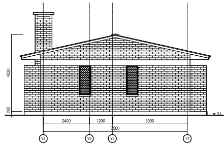
EAST ELEVATION
