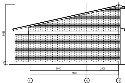
EAST ELEVATION
