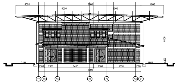
WEST ELEVATION
