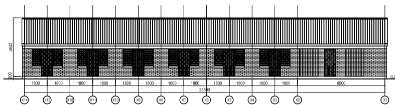
NORTH ELEVATION
