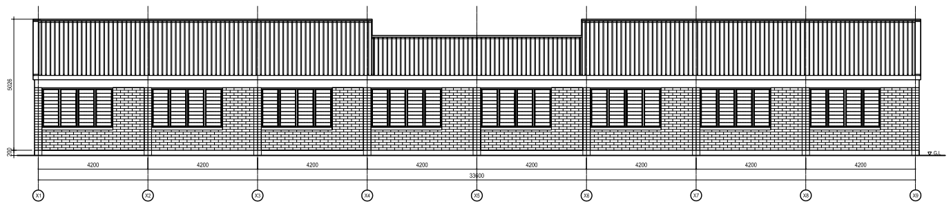
SOUTH ELEVATION
