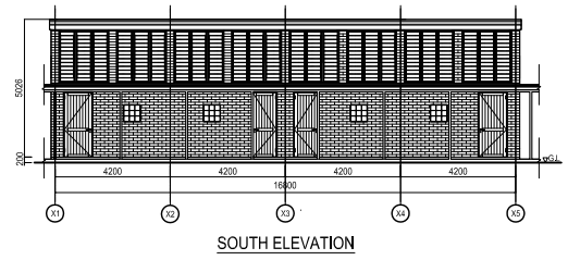
SOUTH ELEVATION
