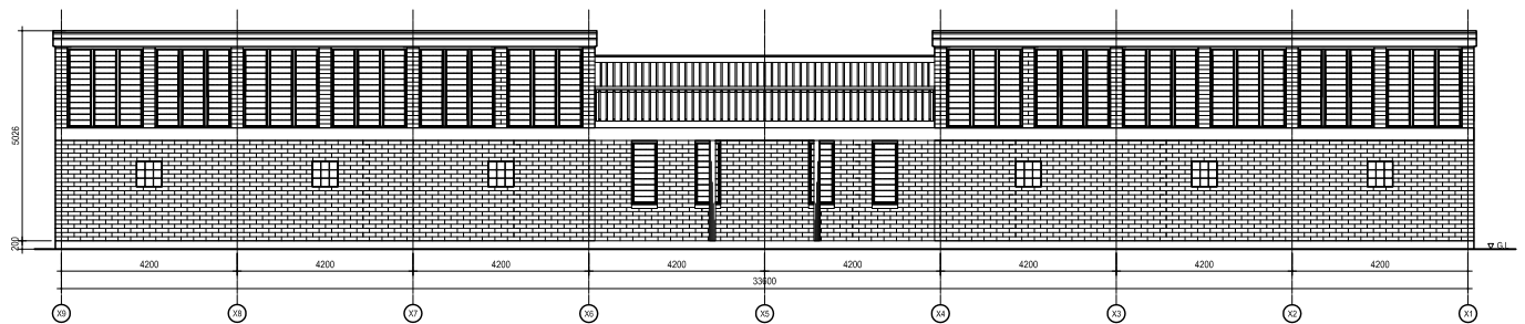
NORTH ELEVATION
