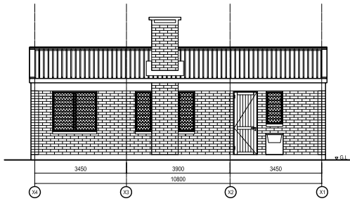
SOUTH ELEVATION
