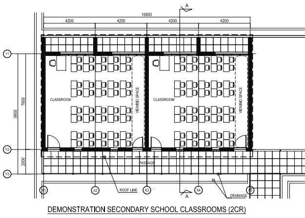
DEMONSTRATION SECONDARY SCHOOL CLASSROOMS (2CR)
