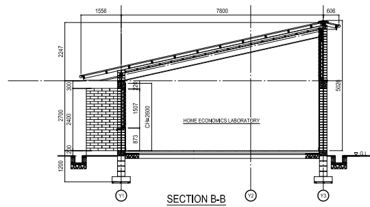
A-07 HOME ECONOMICS LABORATORY (PLAN, ELEVATION, SECTION) S:1/200
