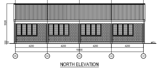
NORTH ELEVATION
