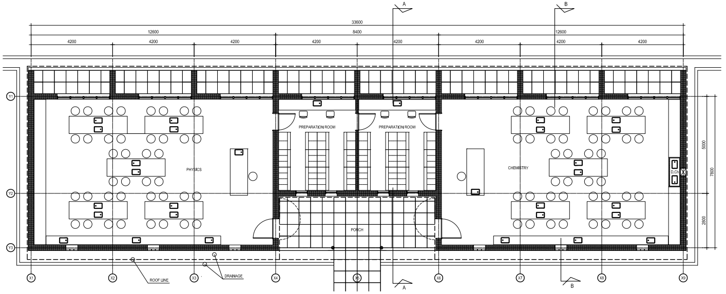
LABORATORY (PHYSICS/CHEMISTRY) PLAN
