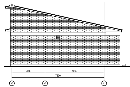
EAST ELEVATION
