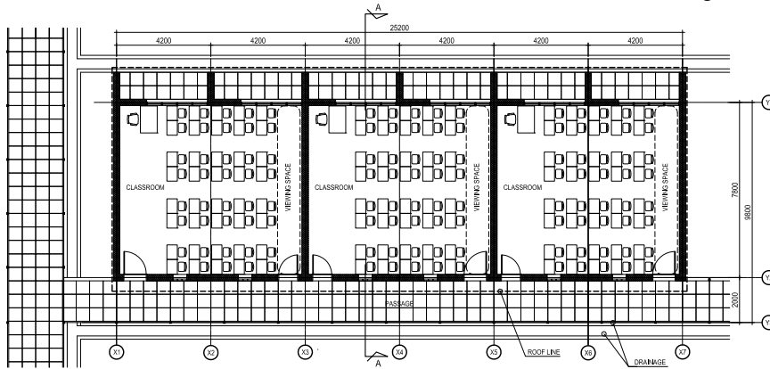
DEMONSTRATION SECONDARY SCHOOL CLASSROOMS (3CR)
