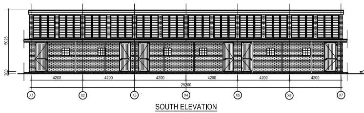
SOUTH ELEVATION
