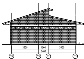
WEST ELEVATION
