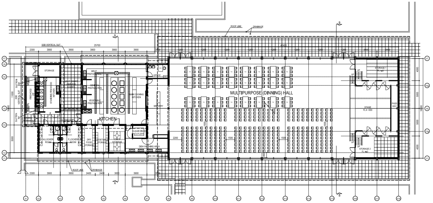
MULTIPURPOSE (DINING) HALL
