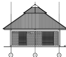
WEST ELEVATION
