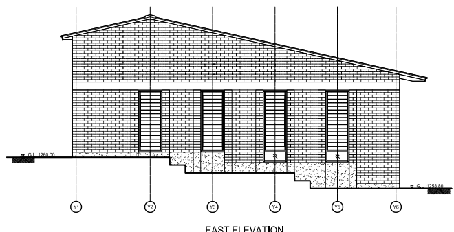
EAST ELEVATION
