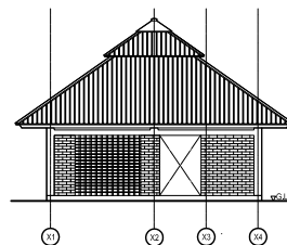
SOUTH ELEVATION
