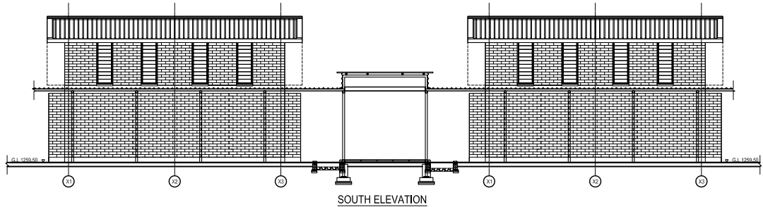
SOUTH ELEVATION
