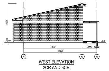
DEMO. SEC. SCHOOL CLASSROOMS(2CR/3CR)
