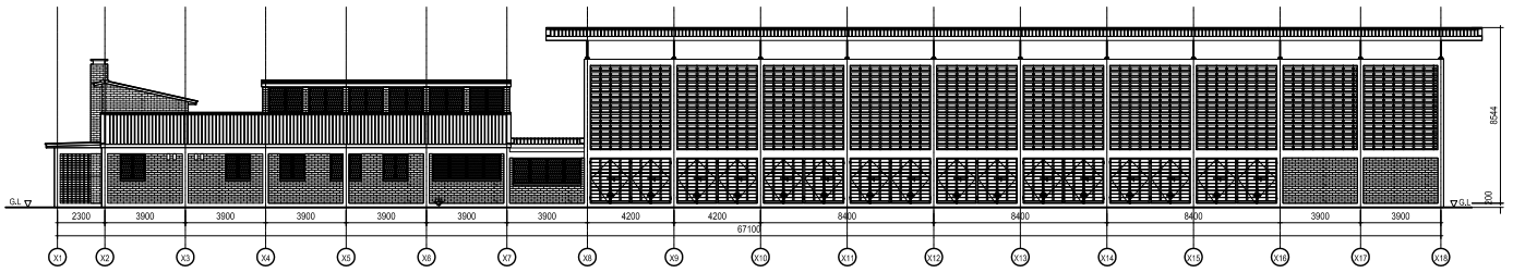
SOUTH ELEVATION
