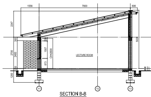
A-03 LECTURE ROOM UNIT (PLAN, ELEVATION, SECTION) S:1/200
