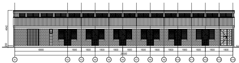
SOUTH ELEVATION
