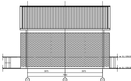
NORTH ELEVATION
