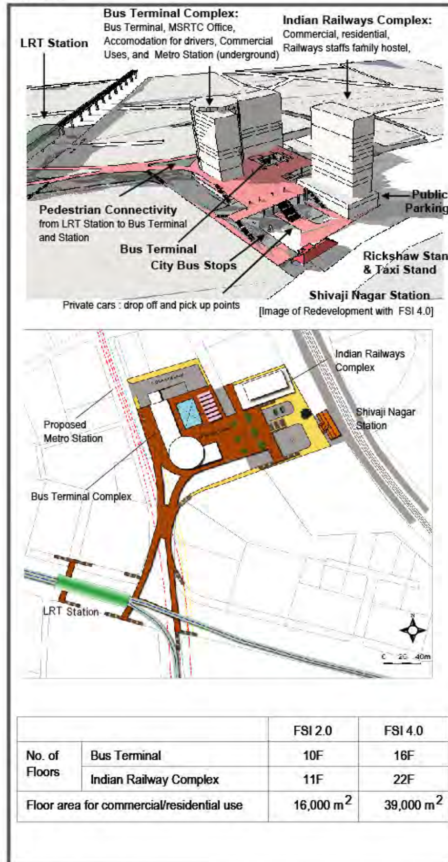
Figure 5.6.3 Optional Scenarios for Redevelopment of Shivaji Nagar Station Area
