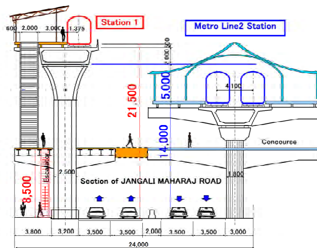
Figure 5.4.6 Plan and Section of Option-2
