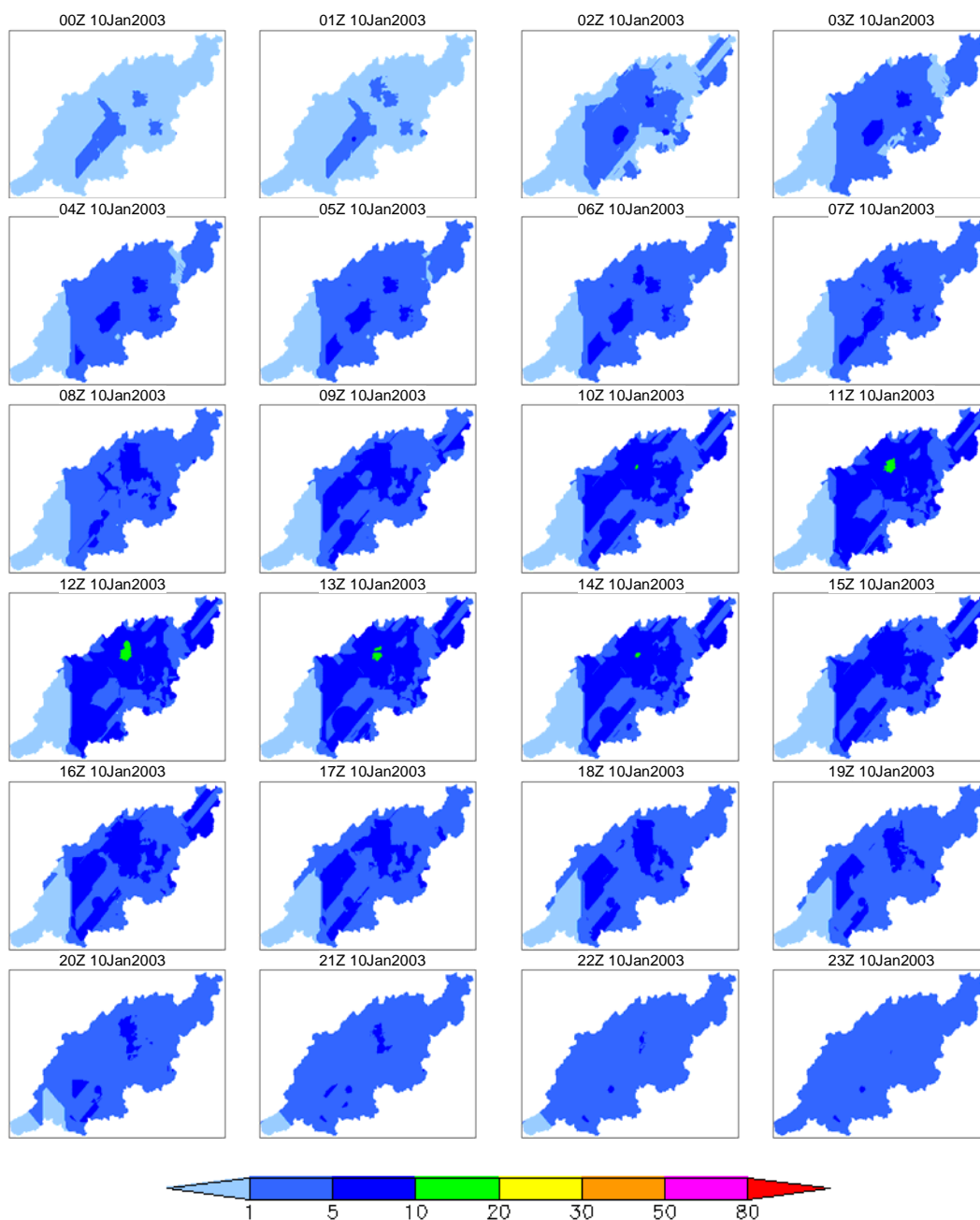
Figure 2b 4-day rainfall 100-year prob. spatio-temporal distribution (January 2003 case, day 2)
