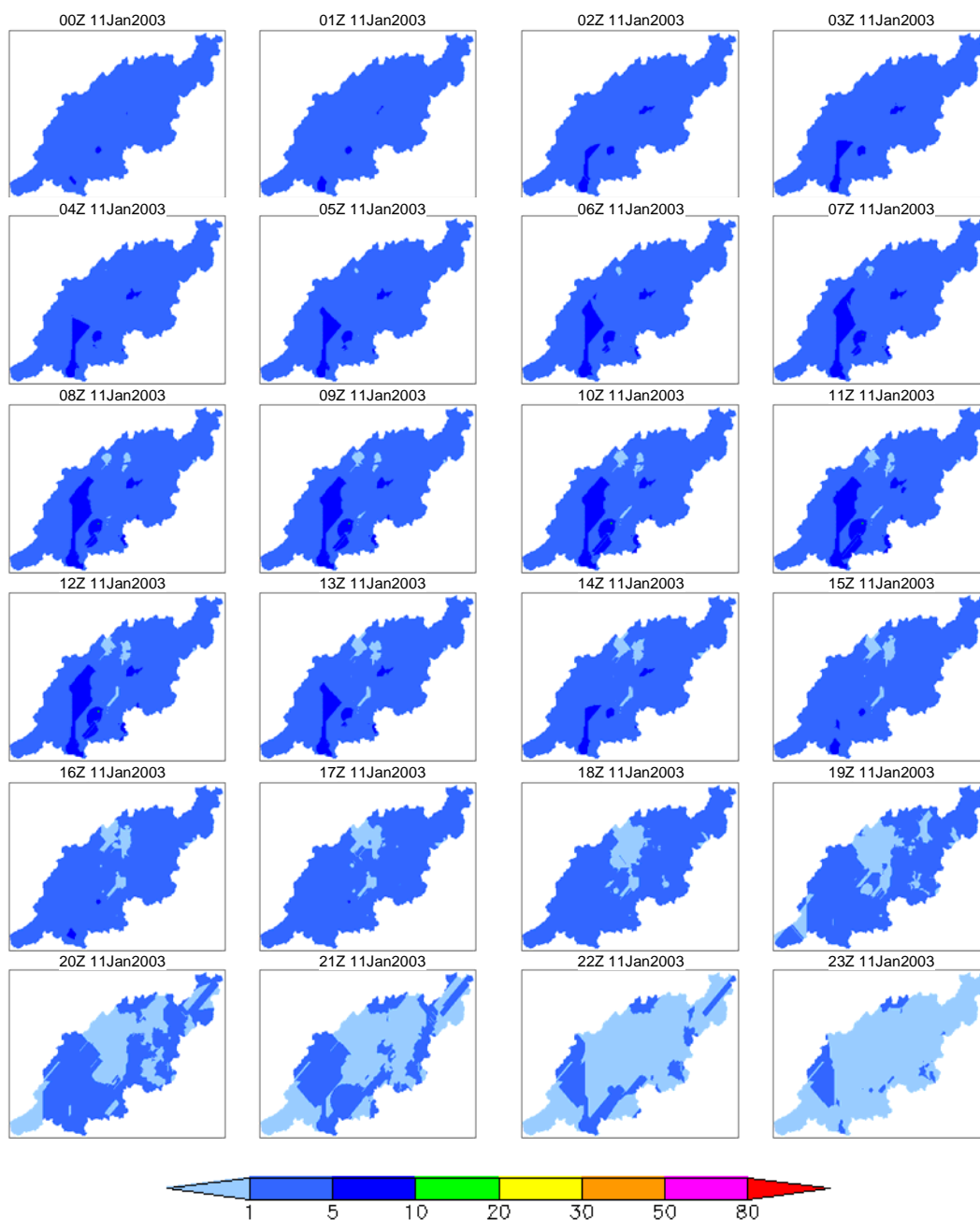
Figure 2c 4-day rainfall 100-year prob. spatio-temporal distribution (January 2003 case, day 3)
