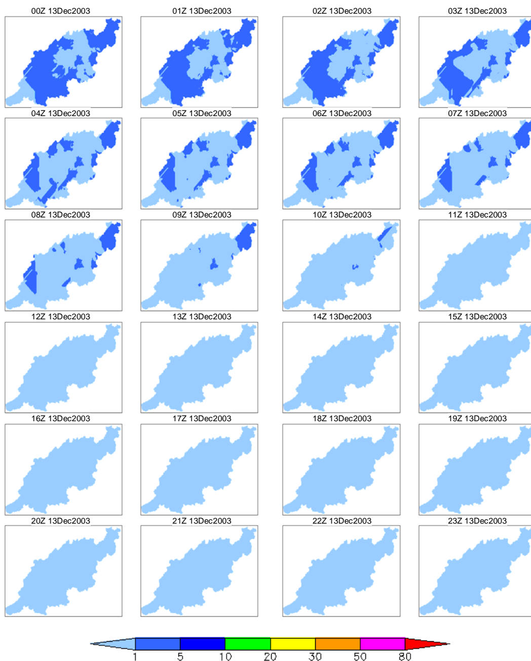
Figure 3d 4-day rainfall 100-year prob. spatio-temporal distribution (December 2003 case, day 4)
