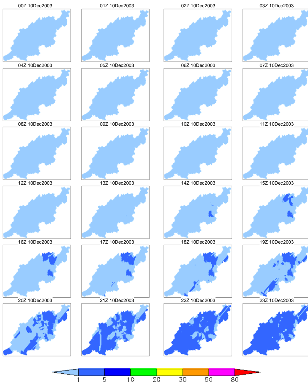
Figure 3a 4-day rainfall 100-year prob. spatio-temporal distribution (December 2003 case, day 1)
