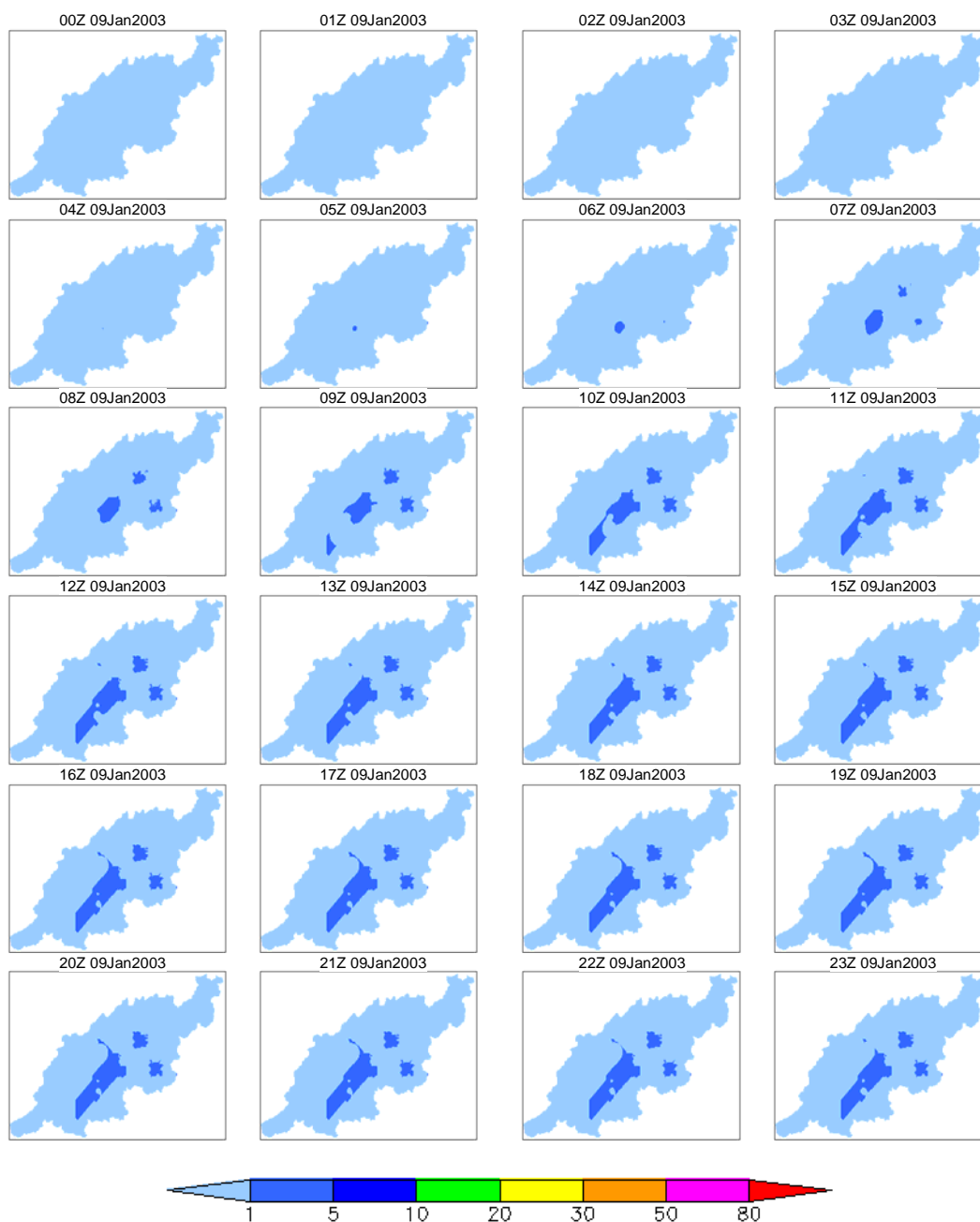
Figure 2a 4-day rainfall 100-year prob. spatio-temporal distribution (January 2003 case, day 1)
