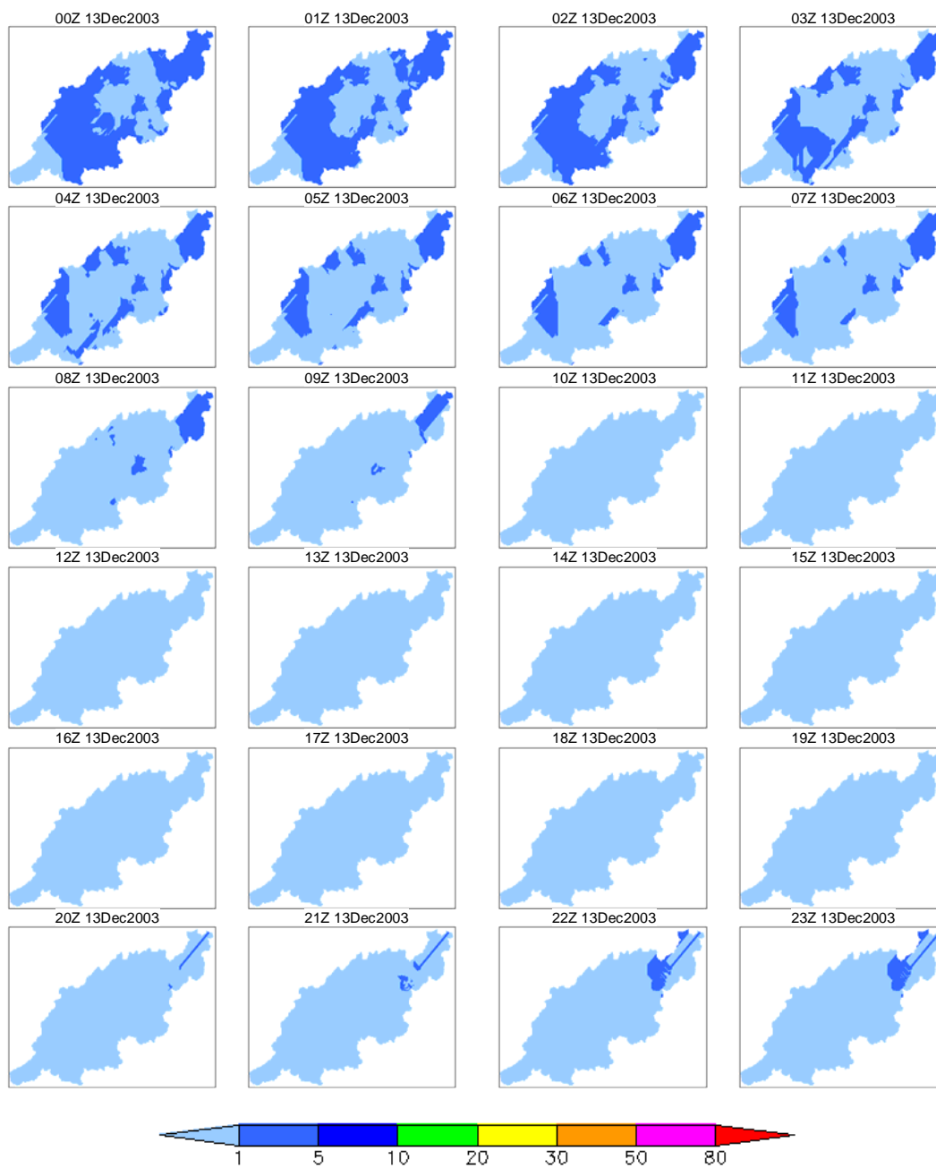
Figure 7d 5-day rainfall 100-year prob. spatio-temporal distribution (December 2003 case, day 4)
