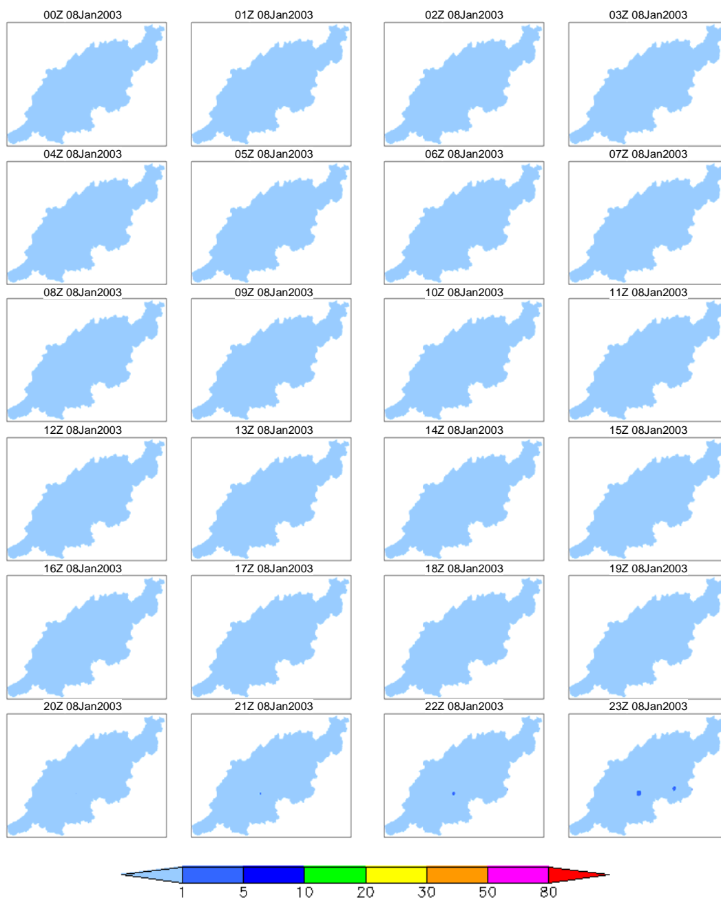
Figure 6a 5-day rainfall 100-year prob. spatio-temporal distribution (January 2003 case, day 1)
