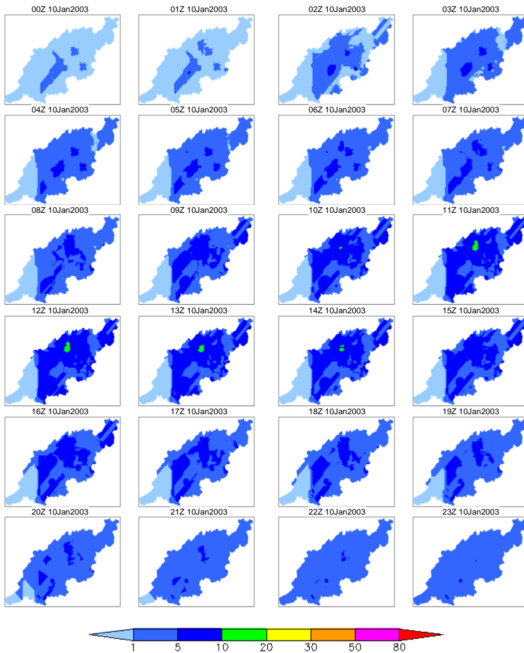
Figure 6c 5-day rainfall 100-year prob. spatio-temporal distribution (January 2003 case, day 3)
