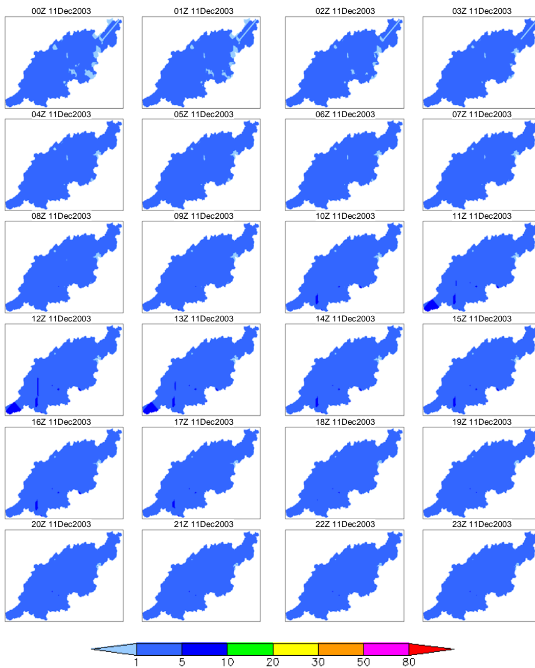
Figure 3b 4-day rainfall 100-year prob. spatio-temporal distribution (December 2003 case, day 2)
