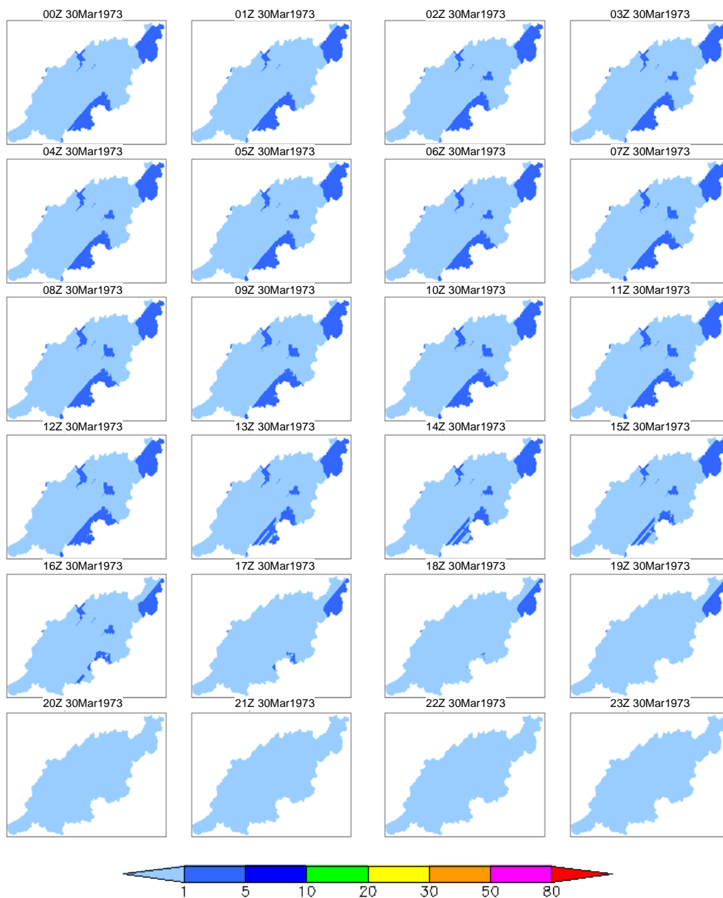
Figure 4e 5-day rainfall 100-year prob. spatio-temporal distribution (March 1973 case, day5)
