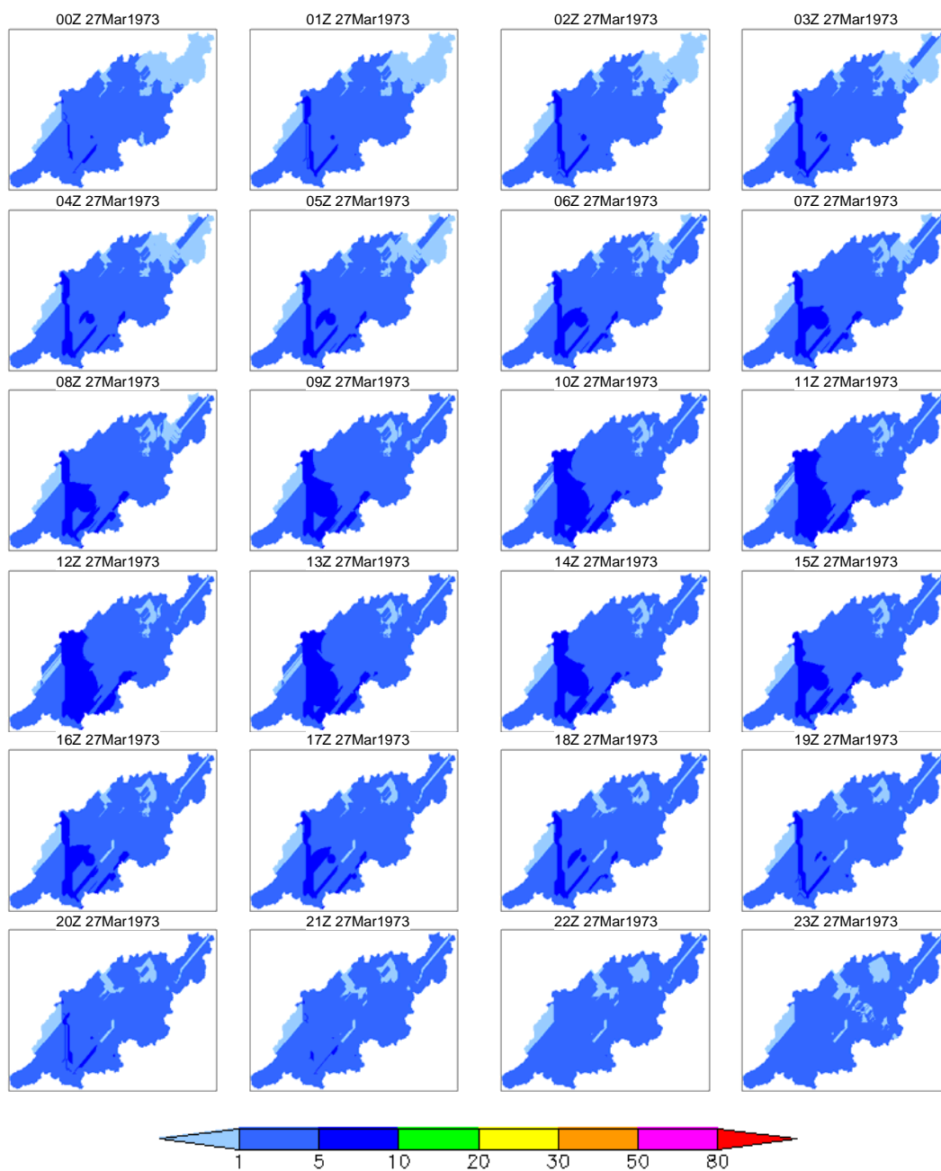
Figure 1b 4-day rainfall 100-year prob. spatio-temporal distribution (March 1973 case, day 2)
