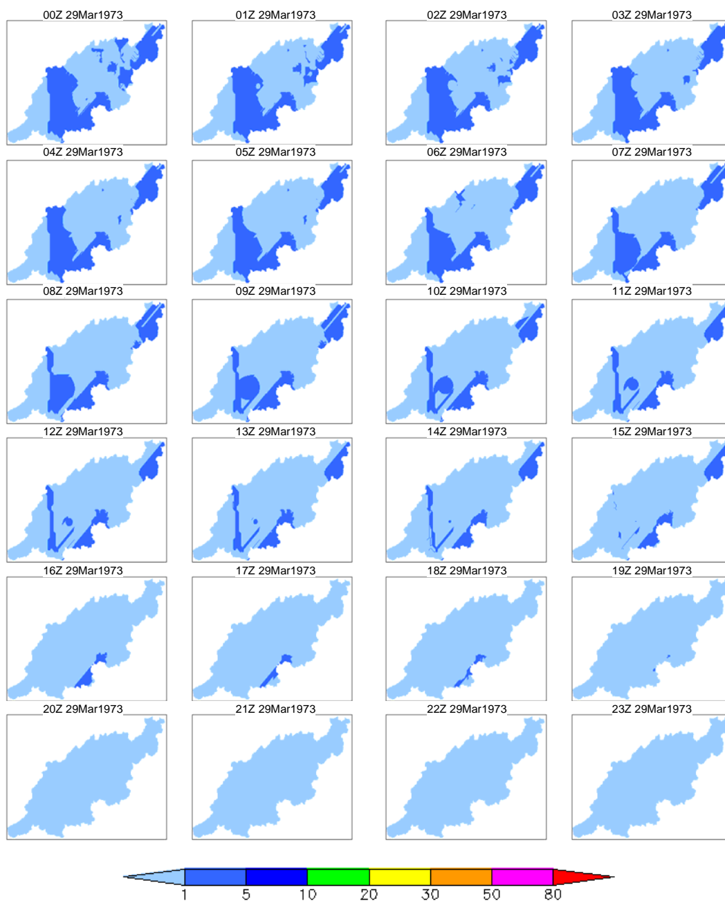
Figure 1d 4-day rainfall 100-year prob. spatio-temporal distribution (March 1973 case, day 4)
