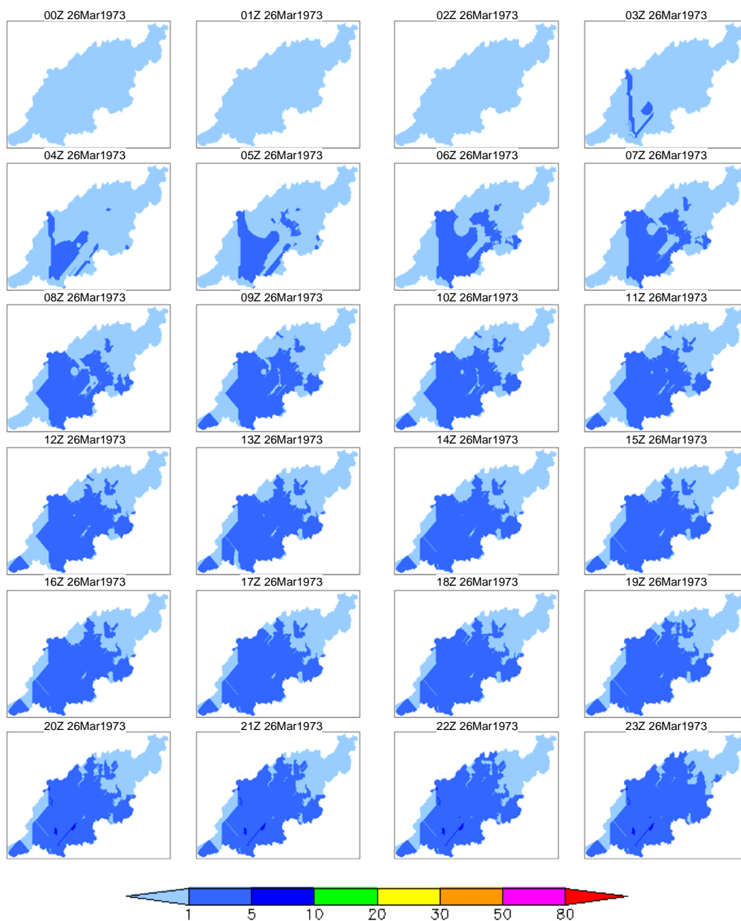
Figure 4a 5-day rainfall 100-year prob. spatio-temporal distribution (March 1973 case, day 1)
