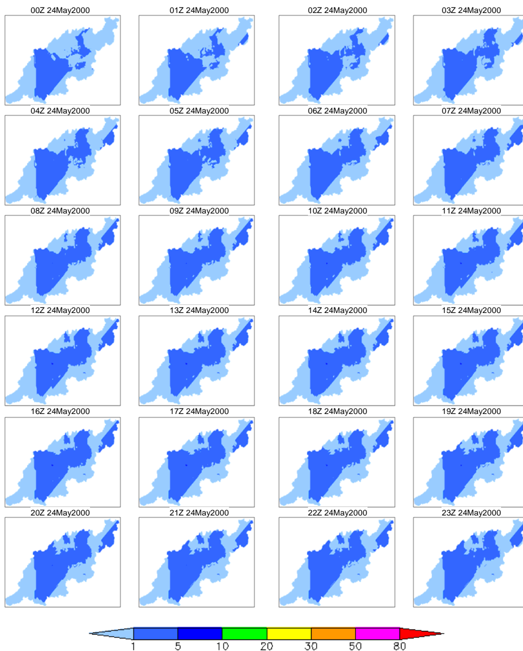
Figure 5b 5-day rainfall 100-year prob. spatio-temporal distribution (May 2000 case, day 2)
