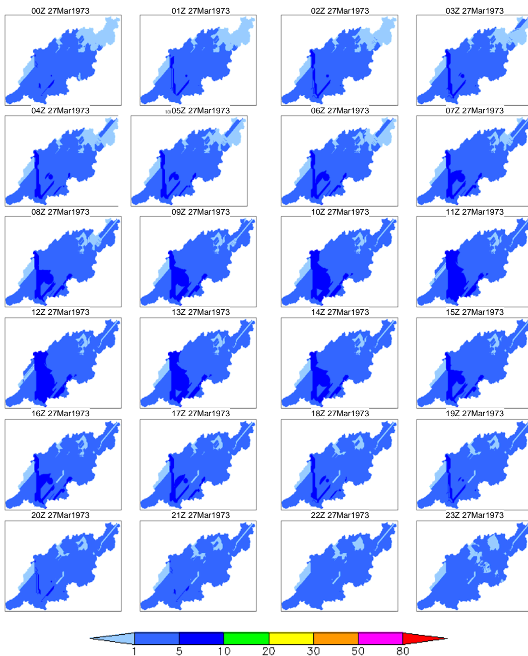
Figure 4b 5-day rainfall 100-year prob. spatio-temporal distribution (March 1973 case, day 2)
