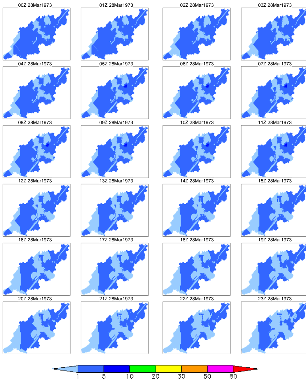
Figure 4c 5-day rainfall 100-year prob. spatio-temporal distribution (March 1973 case, day 3)
