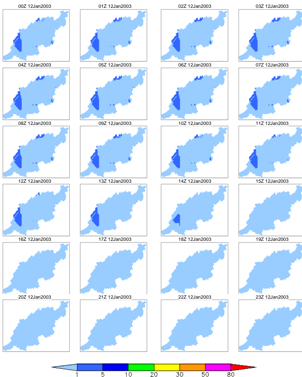
Figure 2d 4-day rainfall 100-year prob. spatio-temporal distribution (January 2003 case, day 4)
