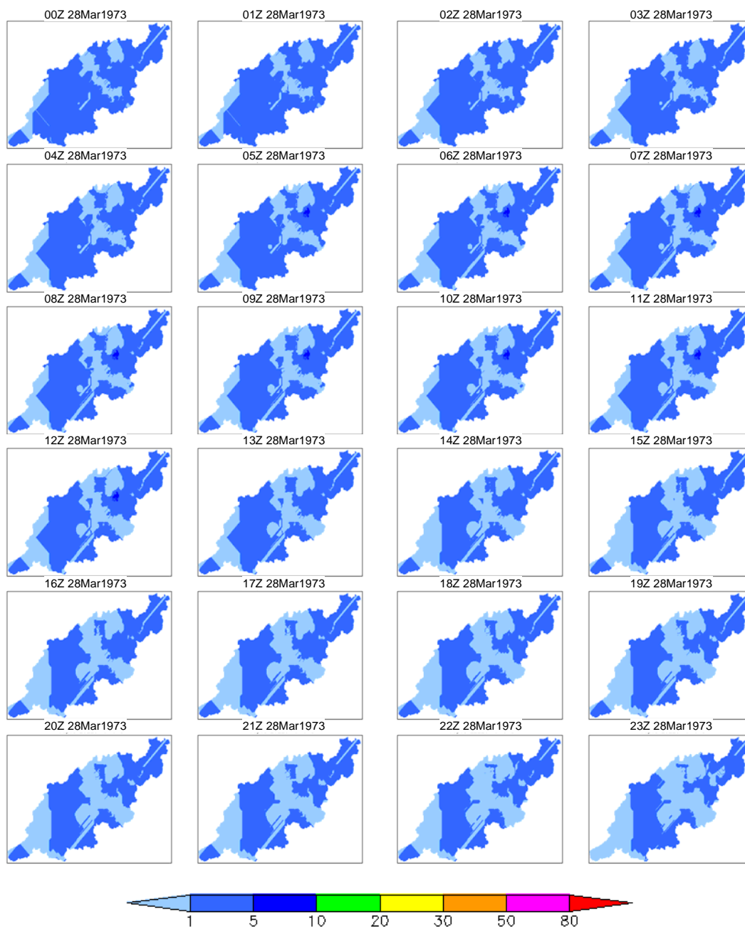
Figure 1c 4-day rainfall 100-year prob. spatio-temporal distribution (March 1973 case, day 3)
