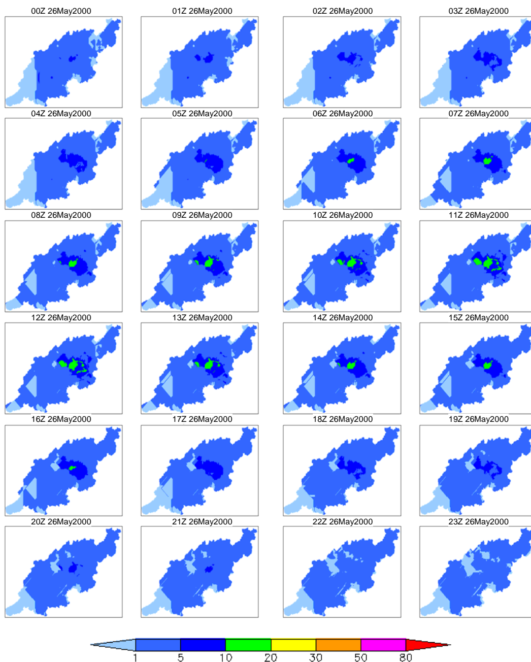
Figure 5d 5-day rainfall 100-year prob. spatio-temporal distribution (May 2000 case, day 4)
