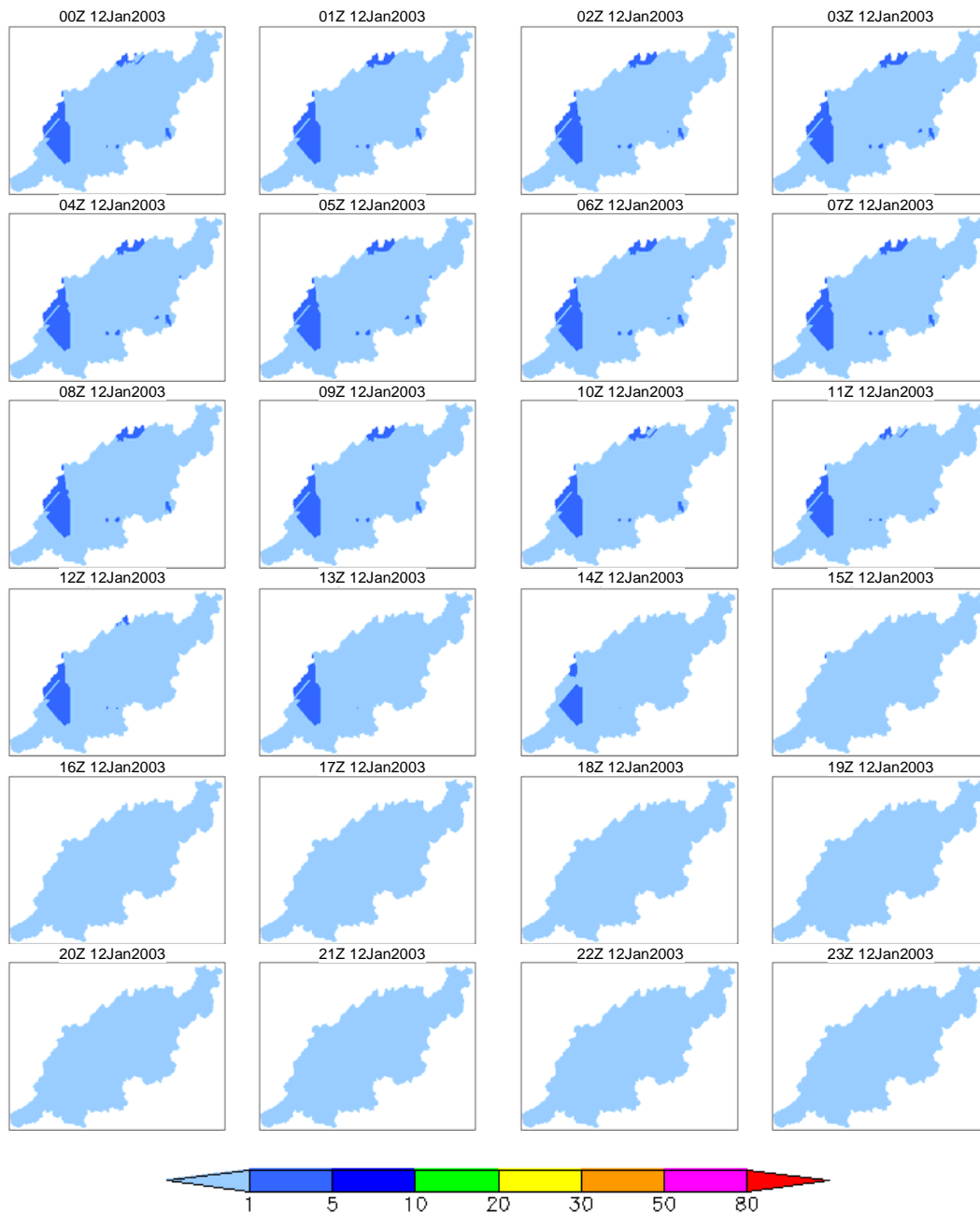
Figure 6e 5-day rainfall 100-year prob. spatio-temporal distribution (January 2003 case, day 5)
