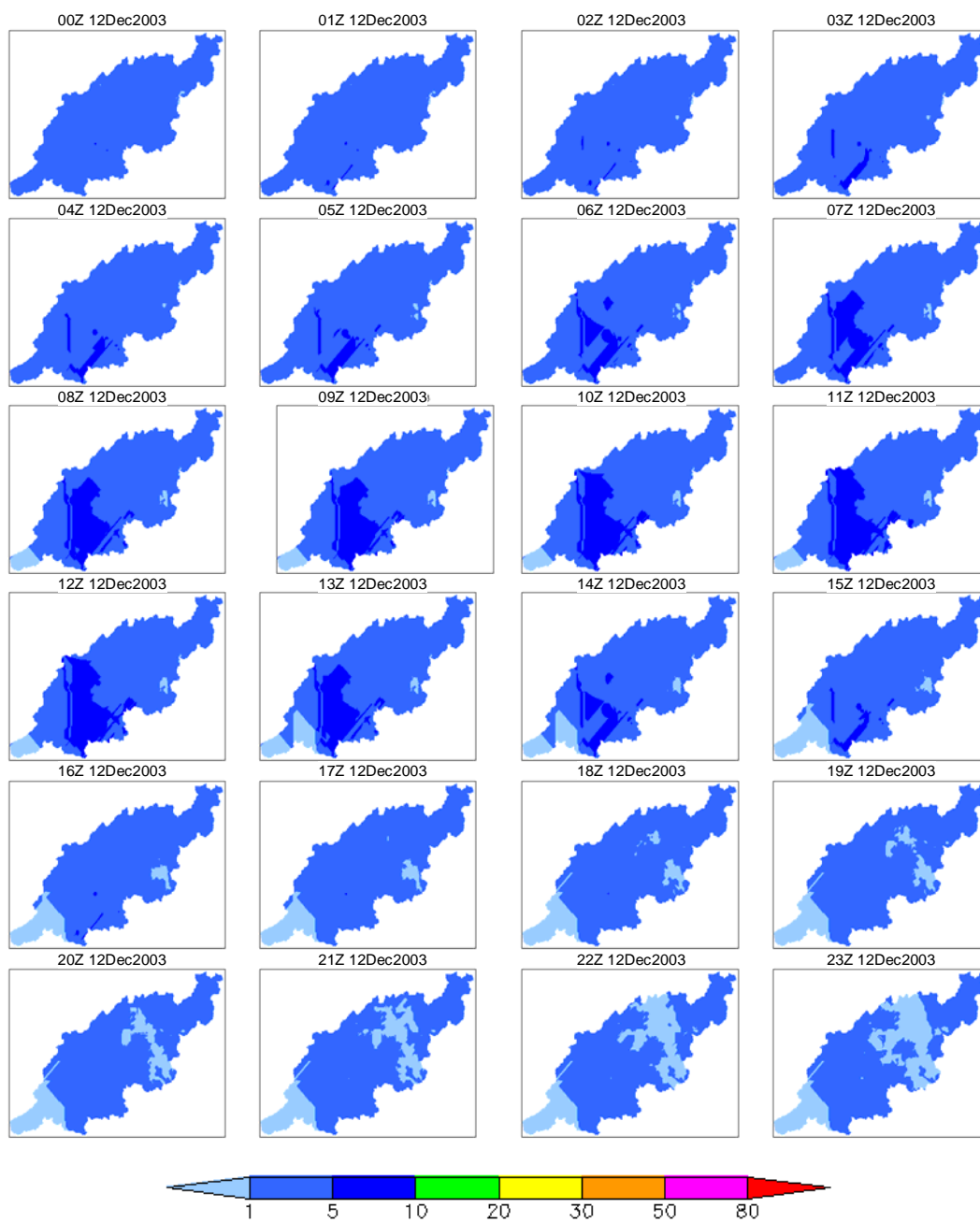
Figure 7c 5-day rainfall 100-year prob. spatio-temporal distribution (December 2003 case, day 3)
