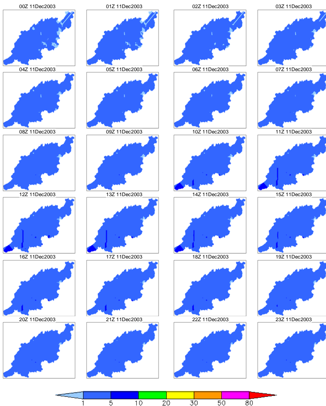
Figure 7b 5-day rainfall 100-year prob. spatio-temporal distribution (December 2003 case, day 2)
