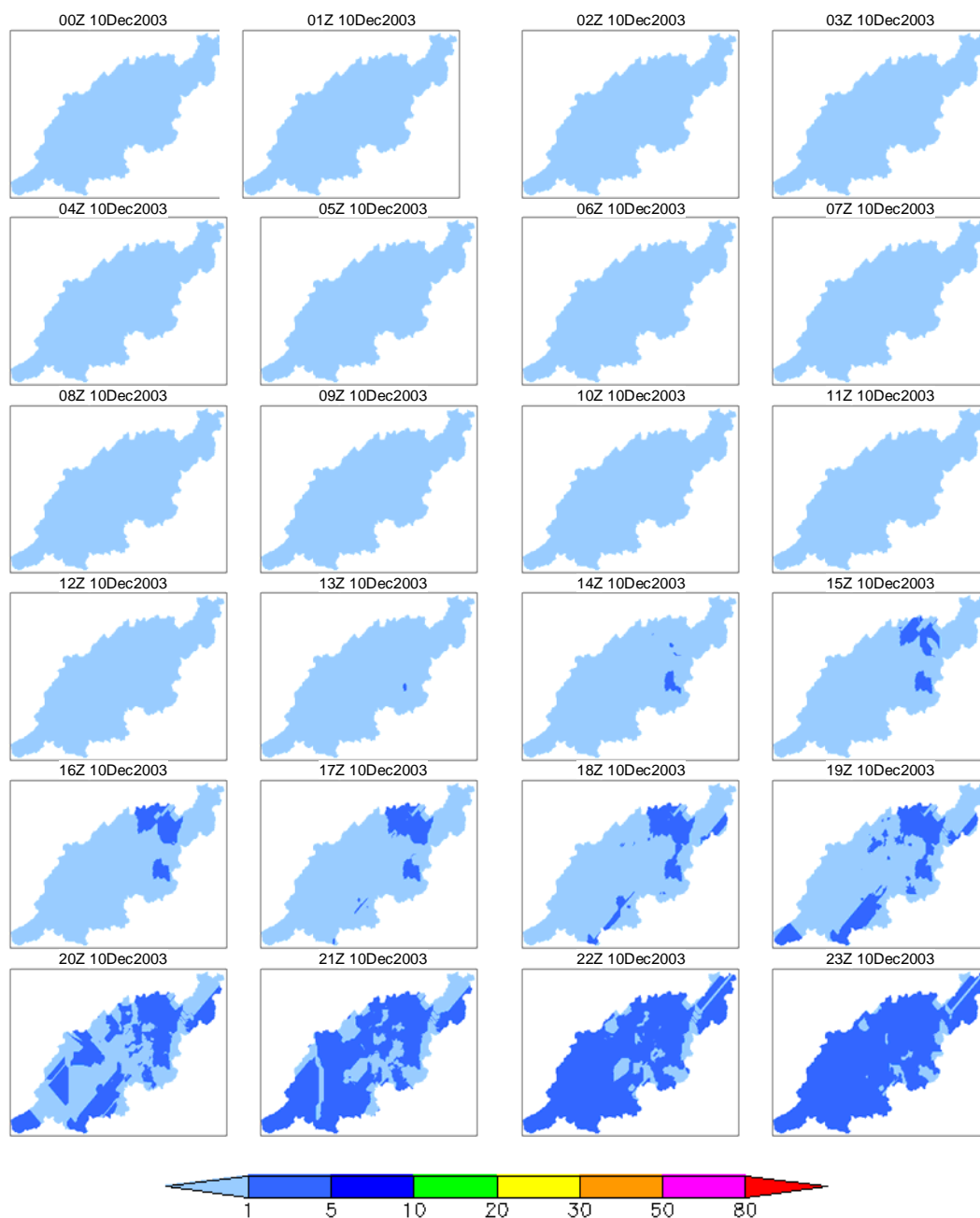
Figure 7a 5-day rainfall 100-year prob. spatio-temporal distribution (December 2003 case, day 1)
