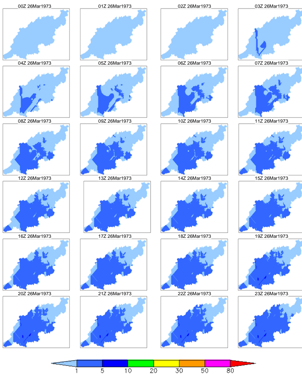
Figure 1a 4-day rainfall 100-year prob. spatio-temporal distribution (March 1973 case, day 1)
