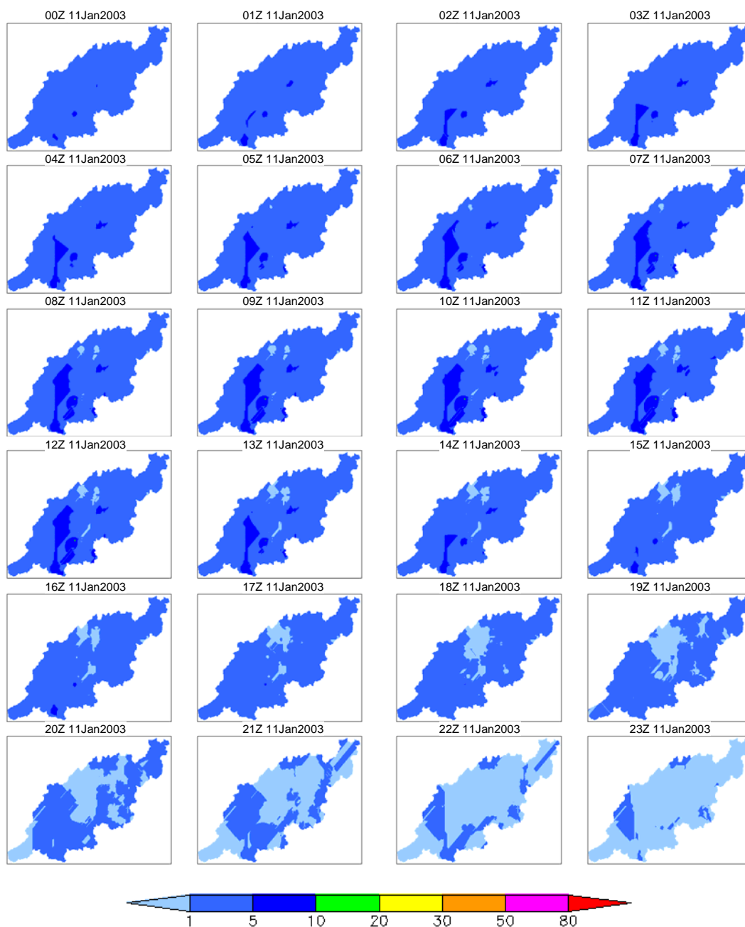
Figure 6d 5-day rainfall 100-year prob. spatio-temporal distribution (January 2003 case, day 4)
