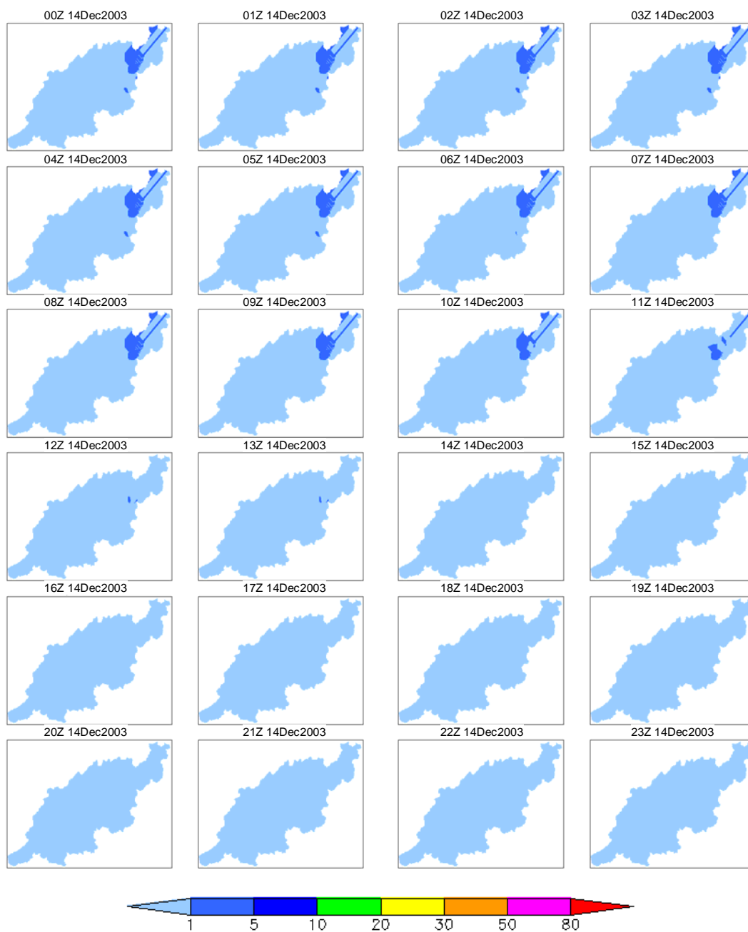
Figure 7e 5-day rainfall 100-year prob. spatio-temporal distribution (December 2003 case, day 5)
