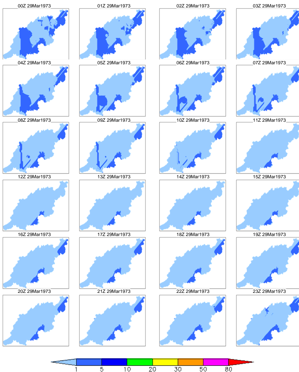
Figure 4d 5-day rainfall 100-year prob. spatio-temporal distribution (March 1973 case, day 4)
