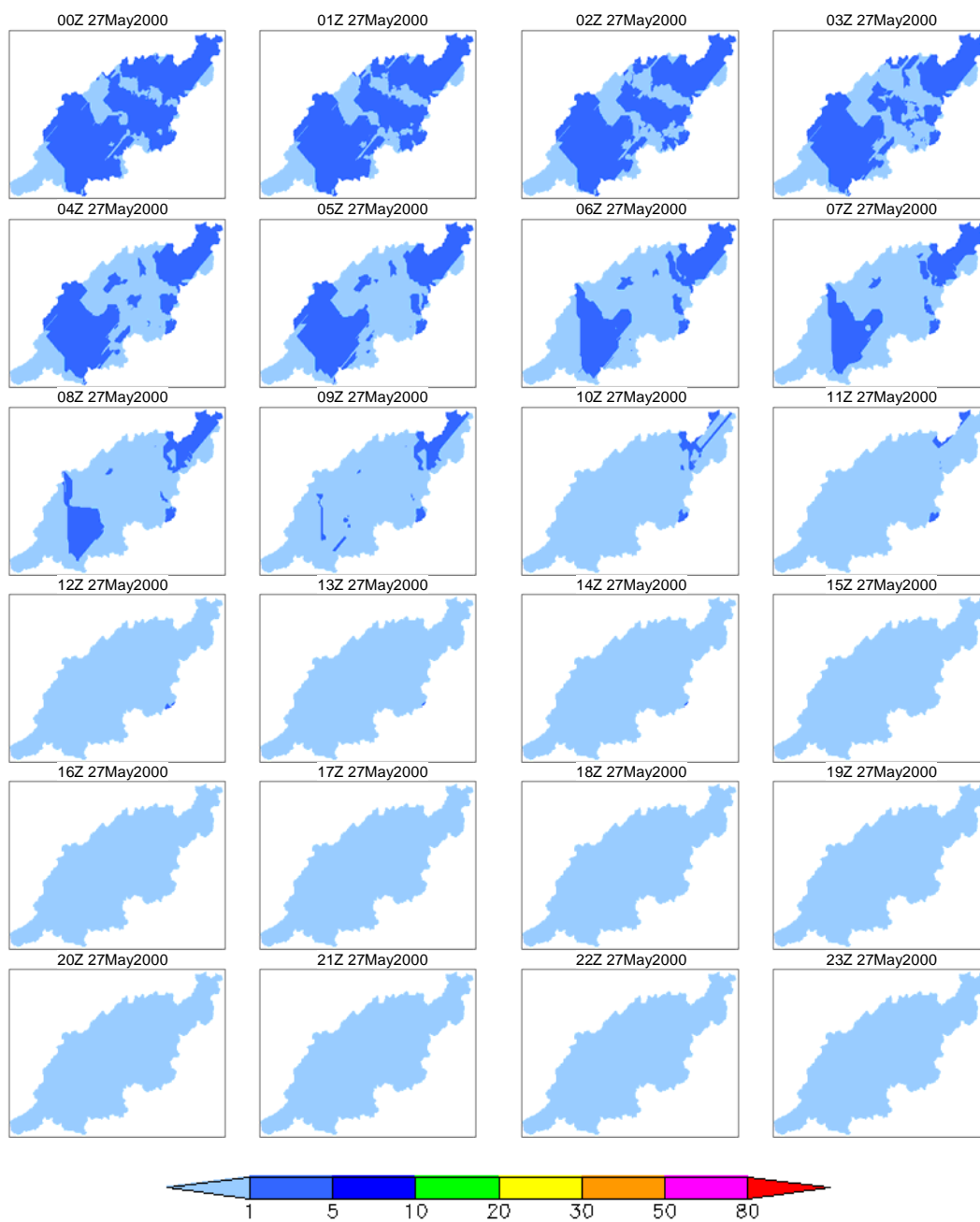
Figure 5e 5-day rainfall 100-year prob. spatio-temporal distribution (May 2000 case, day 5)
