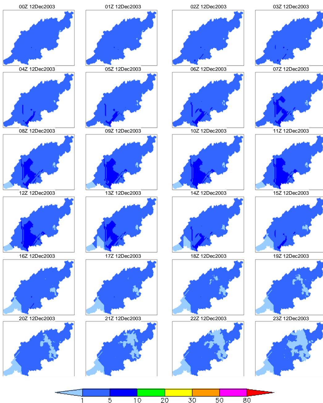
Figure 3c 4-day rainfall 100-year prob. spatio-temporal distribution (December 2003 case, day 3)
