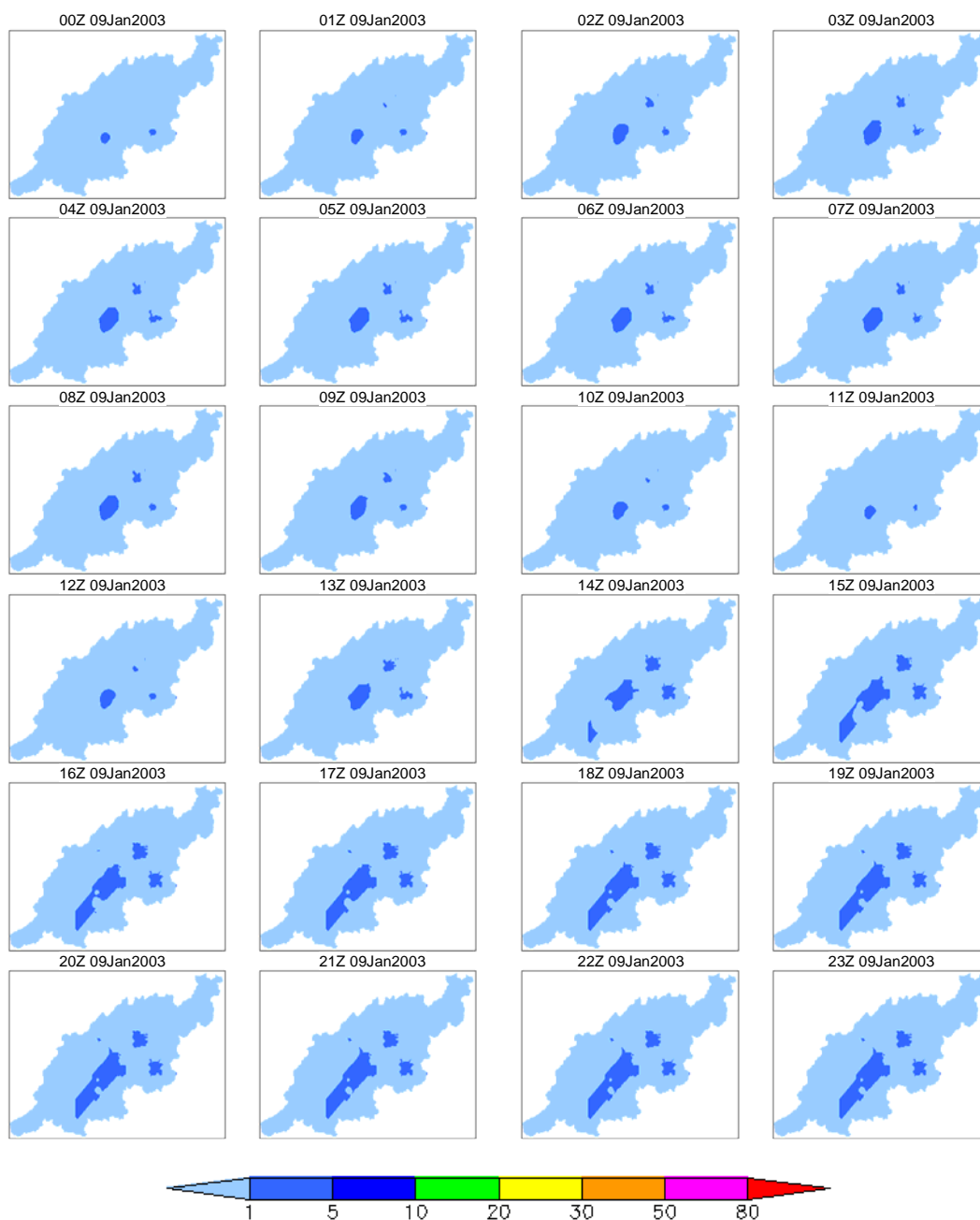
Figure 6b 5-day rainfall 100-year prob. spatio-temporal distribution (January 2003 case, day 2)
