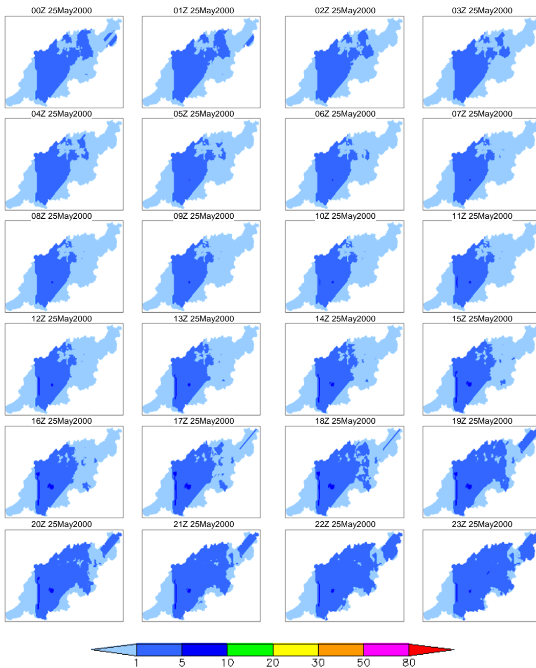
Figure 5c 5-day rainfall 100-year prob. spatio-temporal distribution (May 2000 case, day 3)
