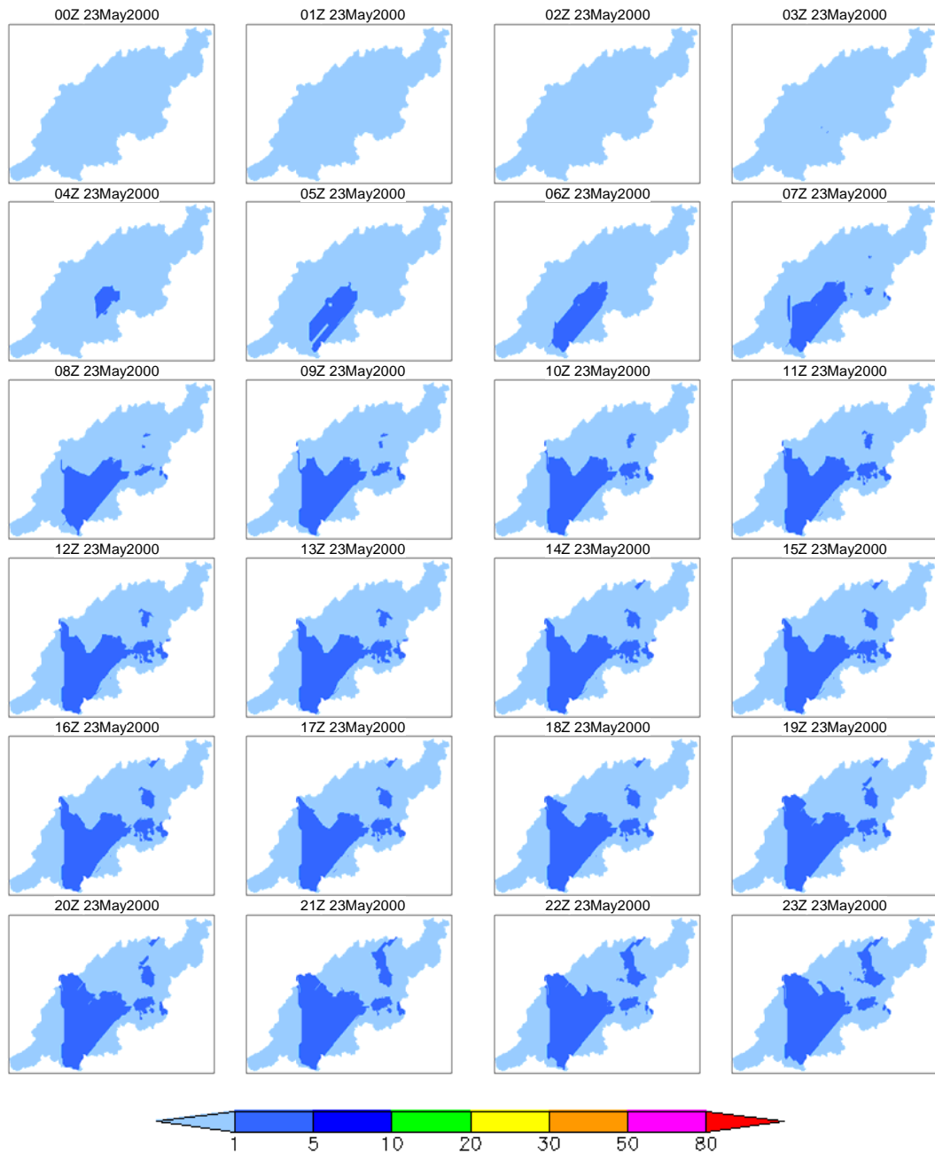
Figure 5a 5-day rainfall 100-year prob. spatio-temporal distribution (May 2000 case, day 1)
