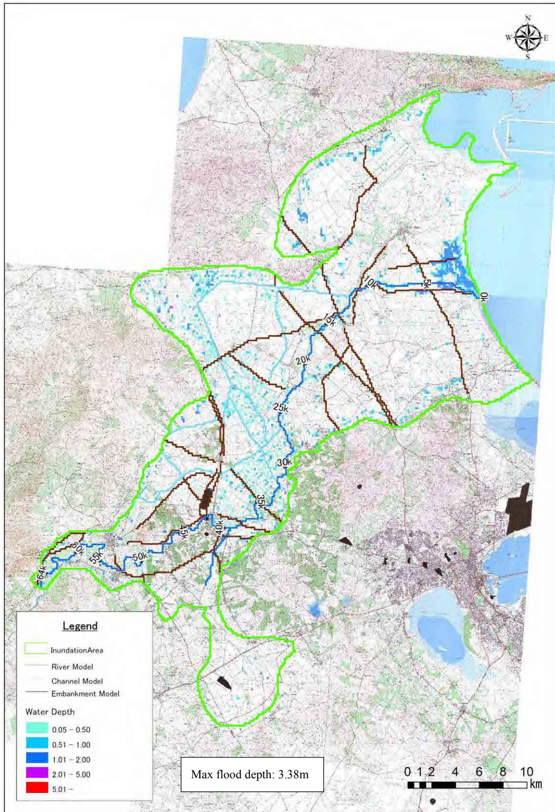
Figure 4-38: Inundation Analysis (current channel, 5th-year discharge)
