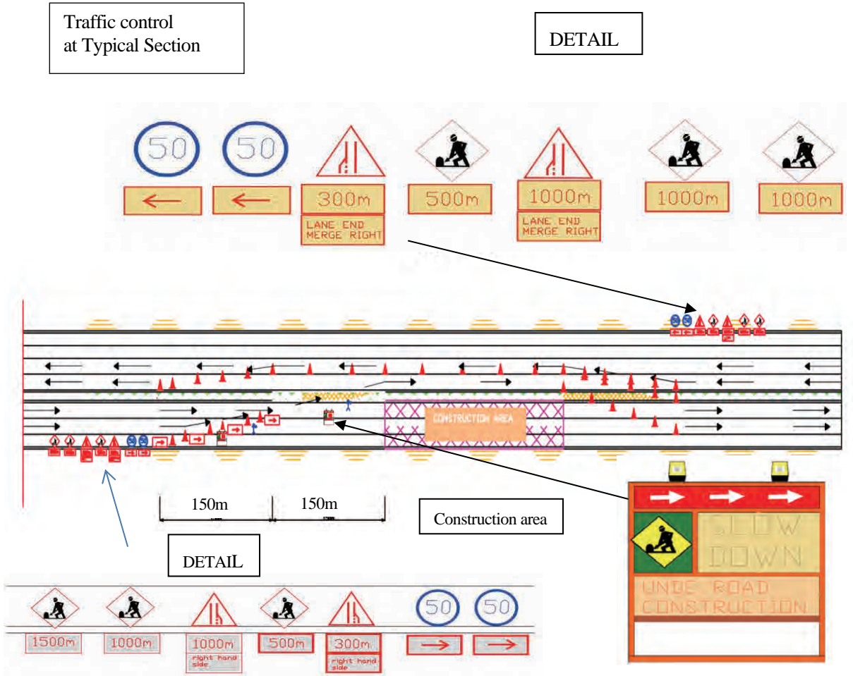
Figure 3.2-16 Traffic Control at Typical Sections
