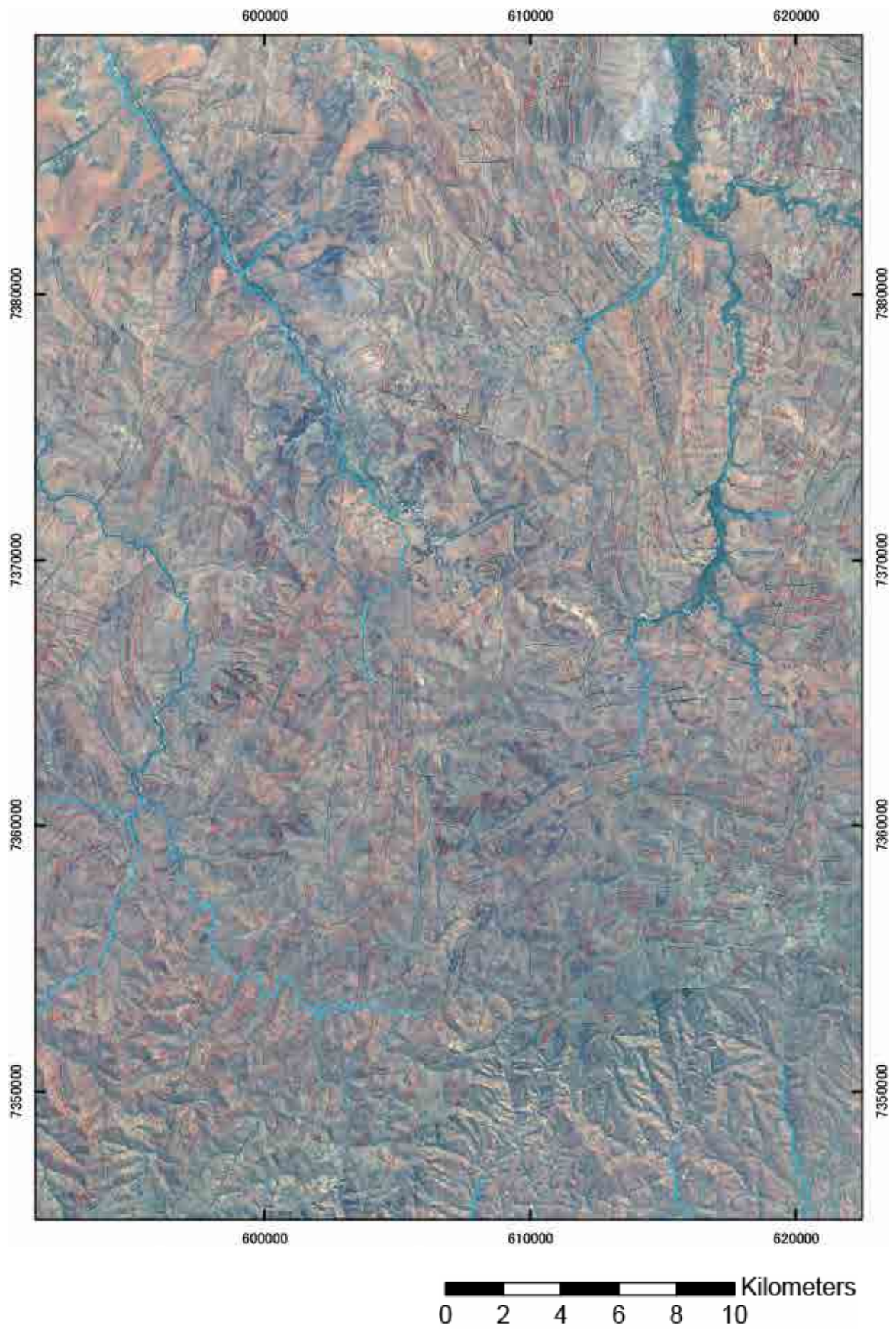
Figure 2. Landsat image of the K59 area
