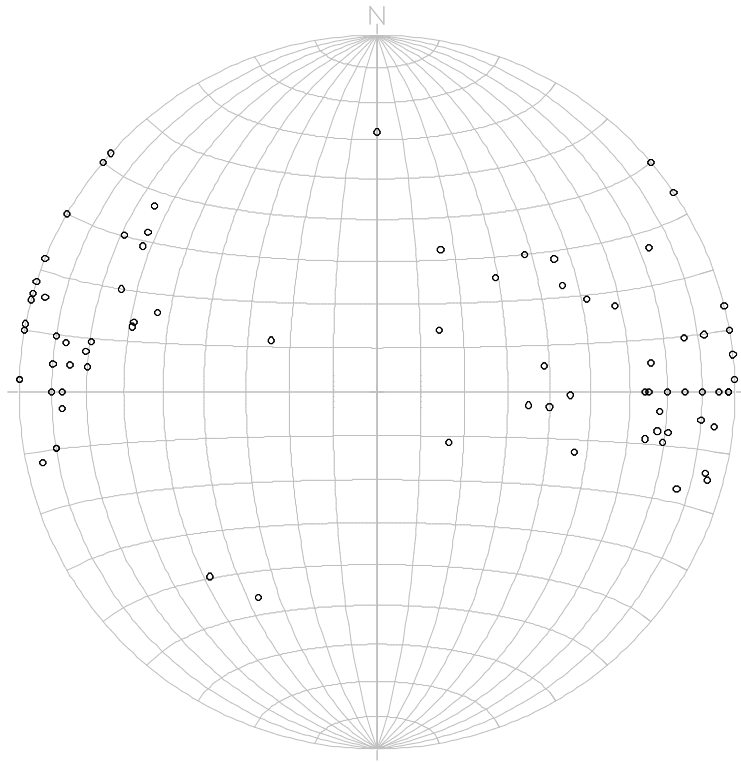
Figure 11. Schmidt's net projection of the strike direction and dip angle observed on the outcrops in the subdomain I. Lower hemisphere projection.
