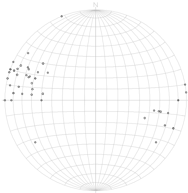
Figure 12. Schmidt's net projection of the strike direction and dip angle observed on the outcrops in the subdomain III. Lower hemisphere projection.
