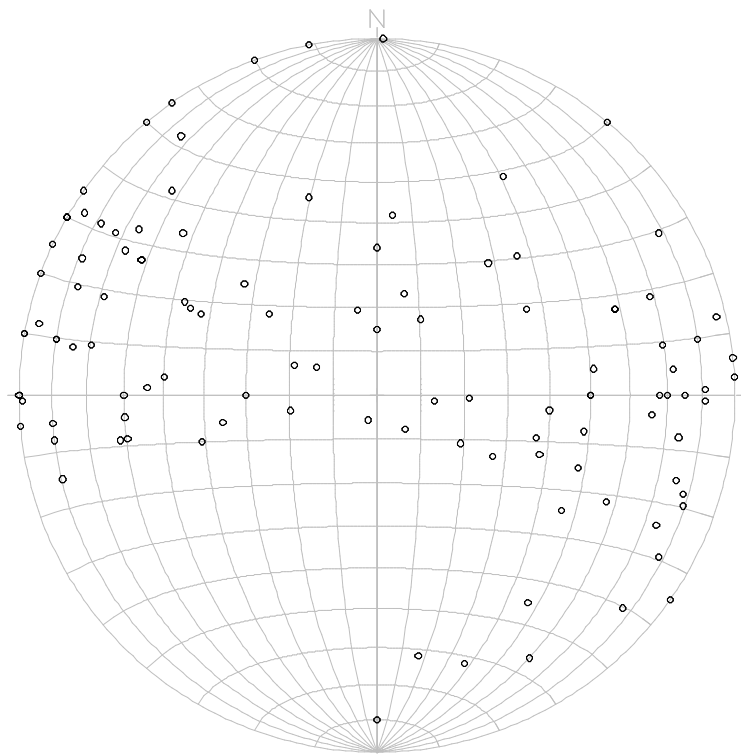
Figure 12. Schmidt's net projection of the strike direction and dip angle observed on the outcrops in the subdomain II. Lower hemisphere projection.
