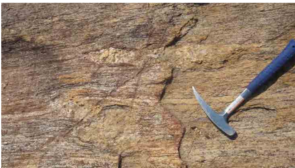
Photo 7. Pelitic gneiss deformed and including coarse-grained quartz and feldspar
