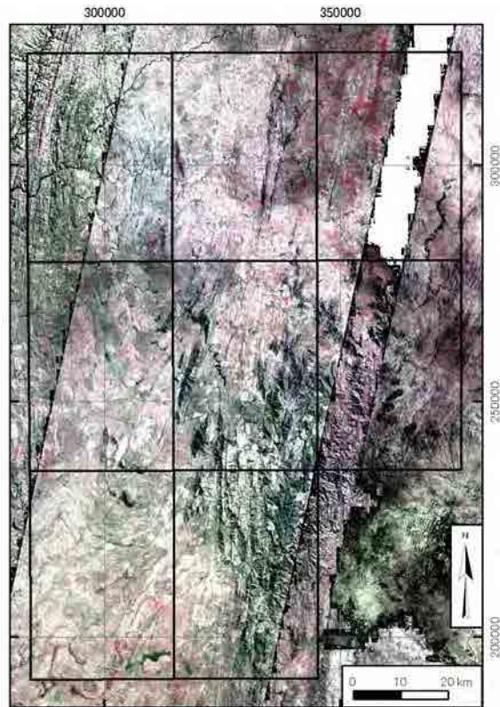
Figure 7.7 Band composite image of ASTER (RGB=B13, B12, B10)
