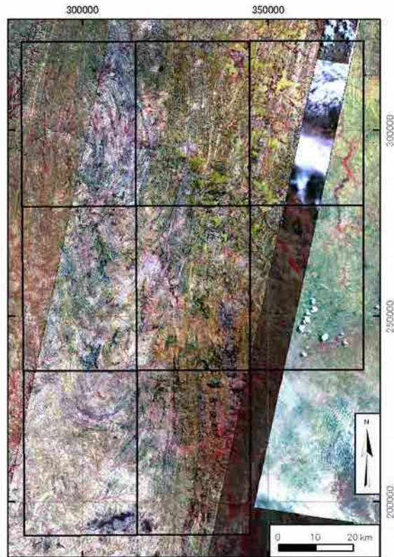
Figure 7.3 Band composite image of ASTER L3 (RGB=B3, B2, B1)
