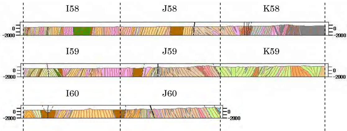
Figure 5.4 Geological cross section
