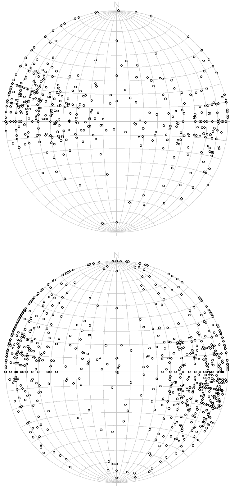
Figure 5.6 Map projection of the lower hemisphere of Schmidt network Anosyen (top) and Androyen (bottom)
