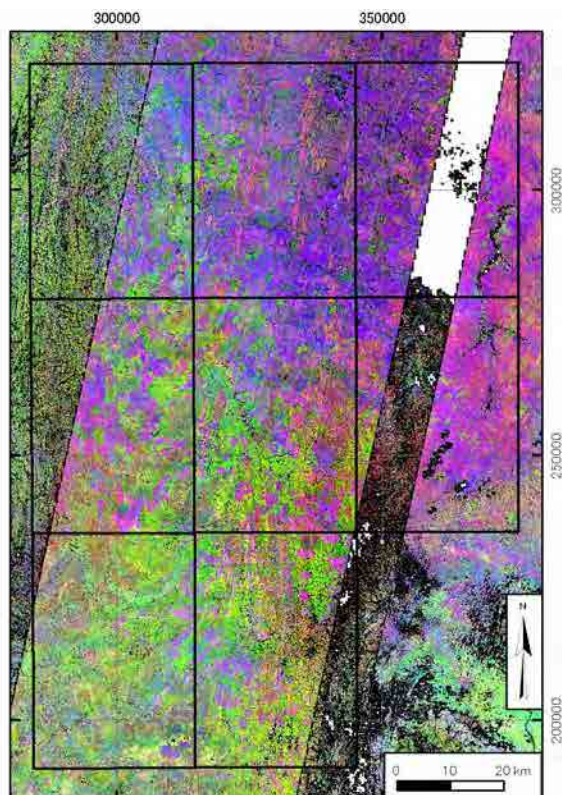
Figure 7.6 Band ratio image of ASTER L3A data (RGB=B5/B6, B6/B8, B5/B4)
