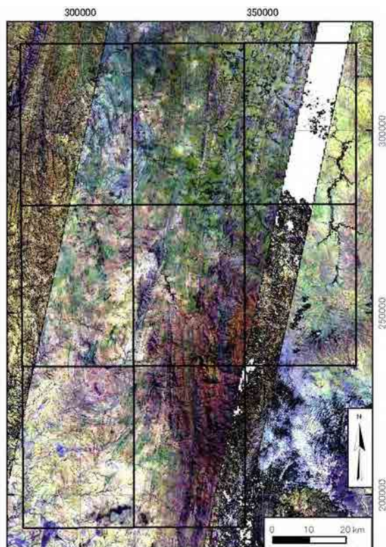
Figure 7.4 Band composite image of ASTER L3 (RGB=B4, B6, B1)
