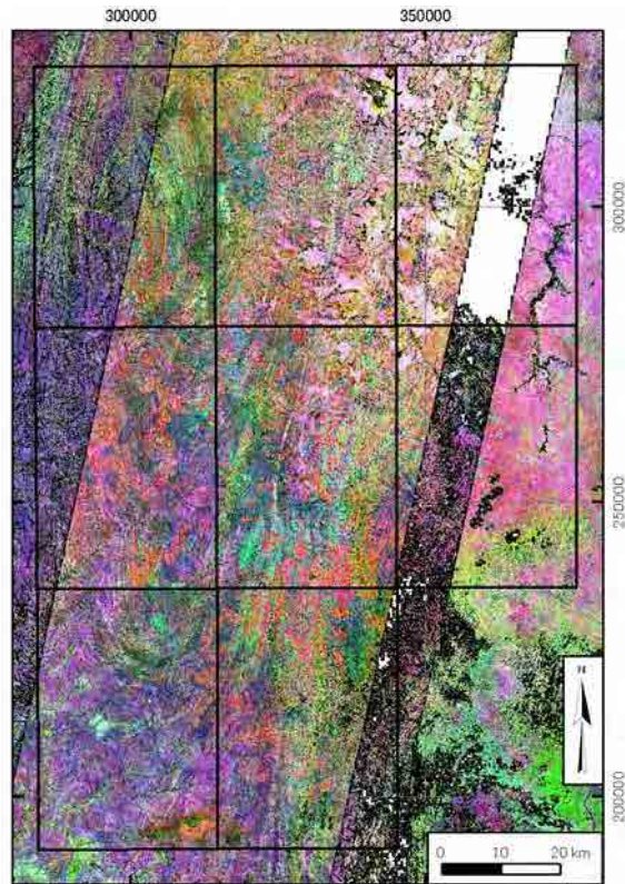
Figure 7.5 Band ratio image of ASTER L3A data (RGB=B7/B6, B3/B4, B2/B1)
