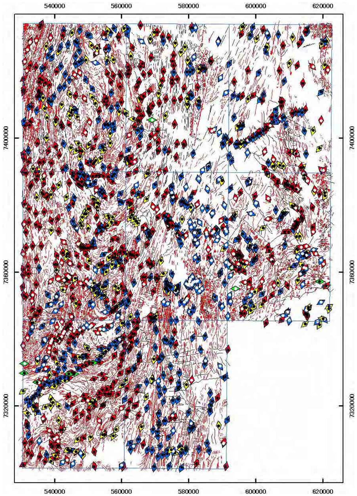
Figure 5.7 Map of geological structure
