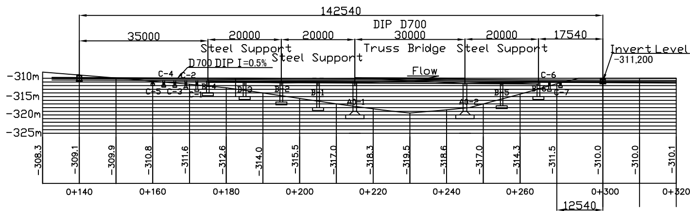
PIPE CROSSING PROFILE
