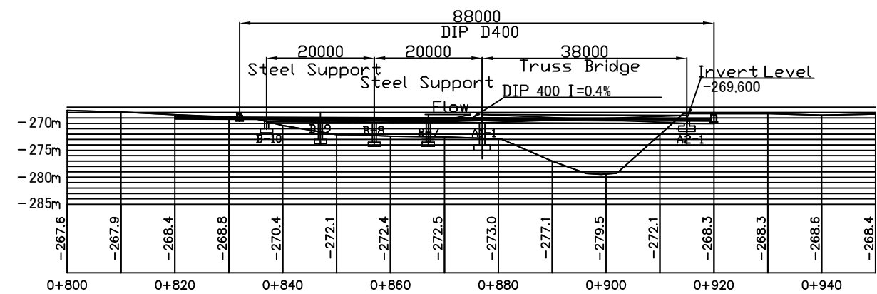
PIPE CROSSING PROFILE
