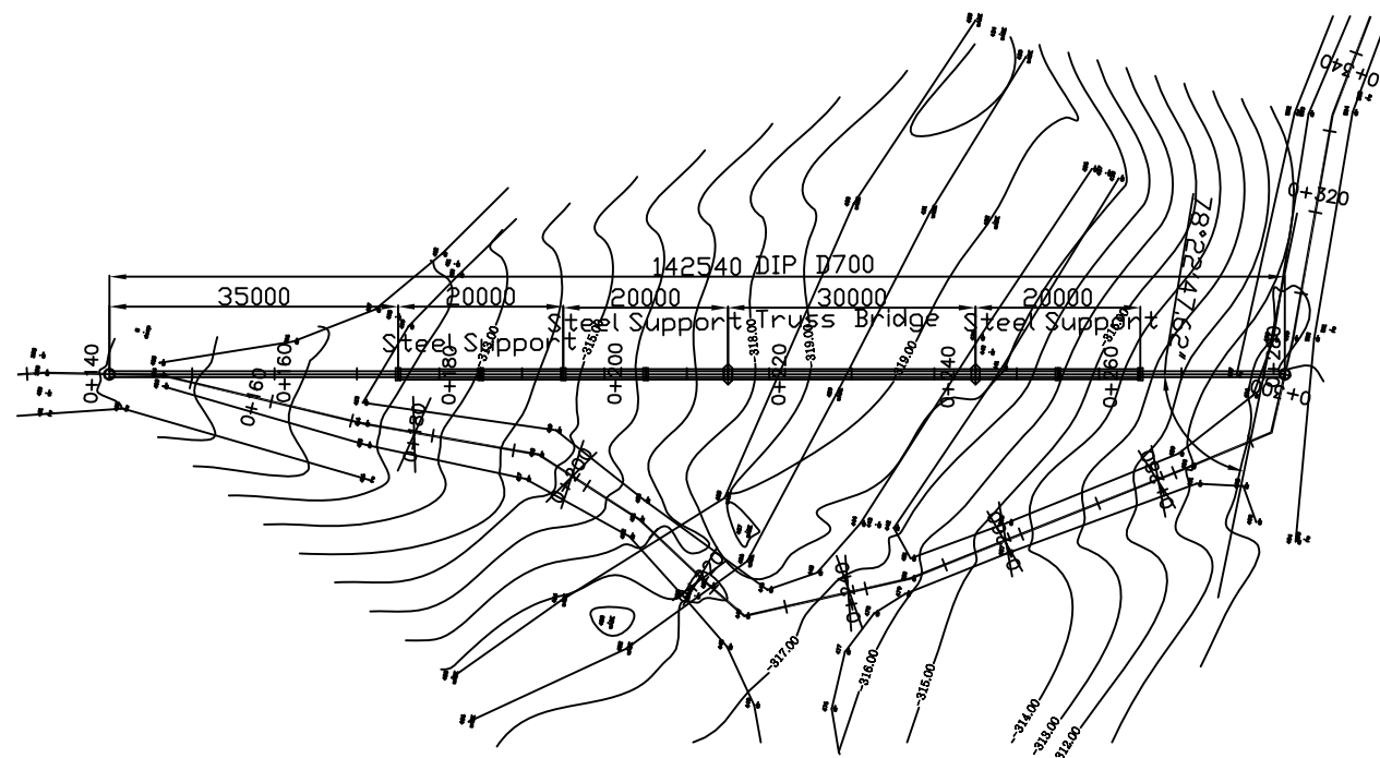
PIPE CROSSING PLAN
