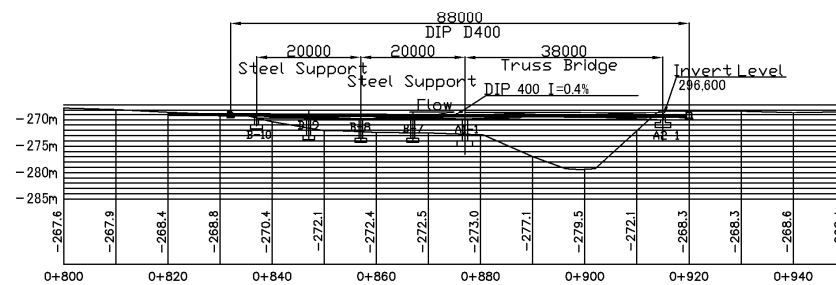
PIPE CROSSING PROFILE
