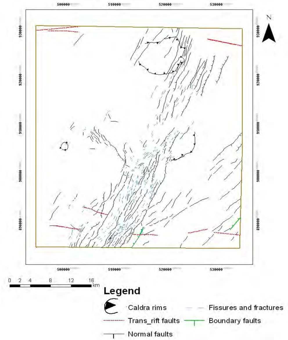
Tectonic Map of the Tulumoye and Gedemsa Geothermal Areas
