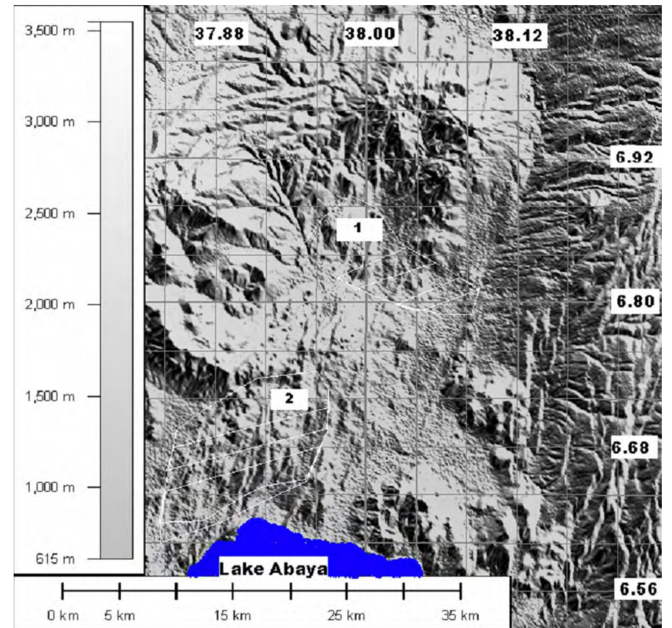
Shaded Relief Elevation Map of Abaya
