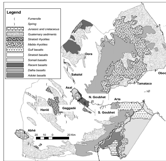
Geologic Map of the Republic of Djibouti
