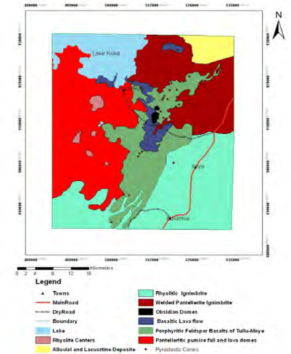
Geologic Map of the Tulumoye and Gedemsa Geothermal Areas
