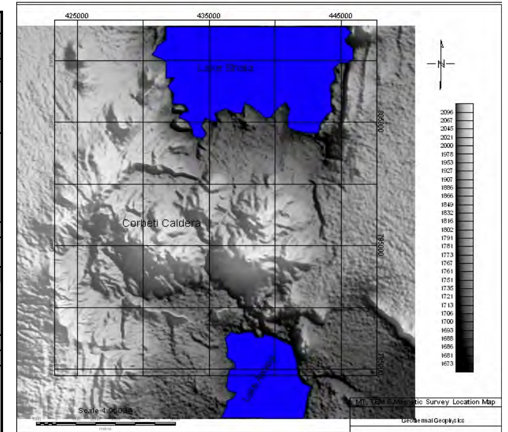
Shaded Relief Elevation Map of Corbetti
