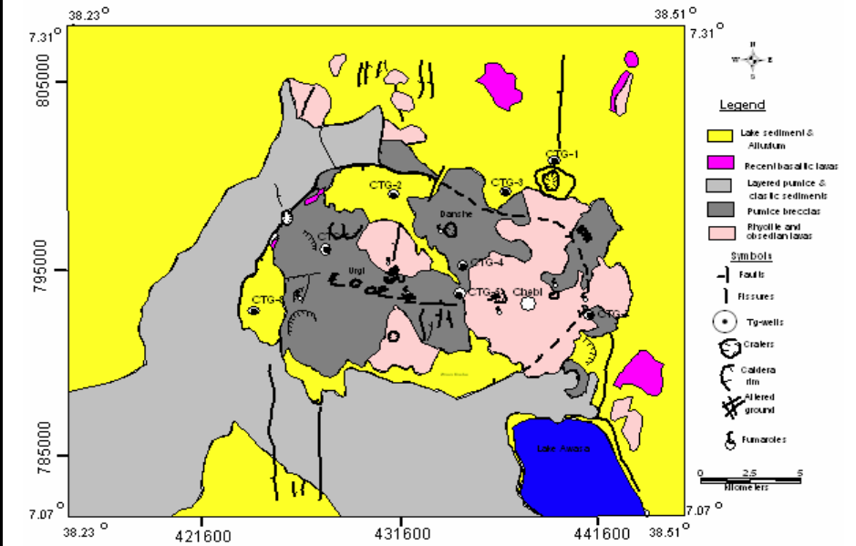
Figure 11, Geological map of Corbetti geothermal prospect (GSE, 1987)
