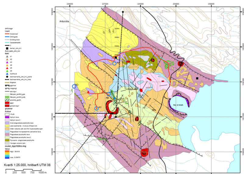
Detailed Geologic Map of the Assal Geothermal Field
