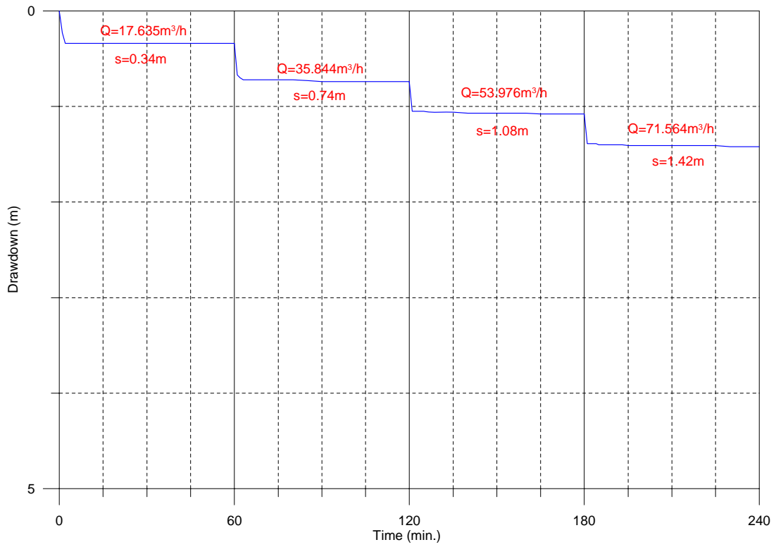
TM3_Gande essai palier-1
