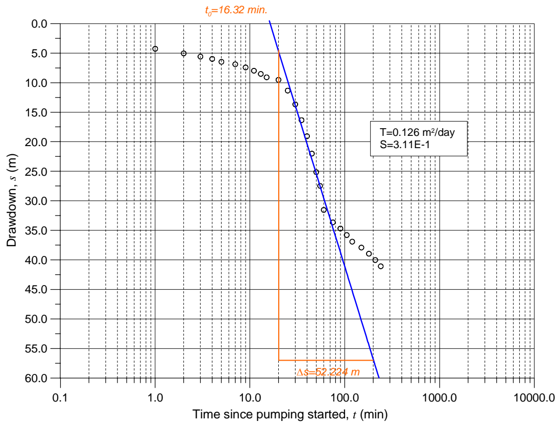
TM6_Yerimale Cooper-Jacobmethode
