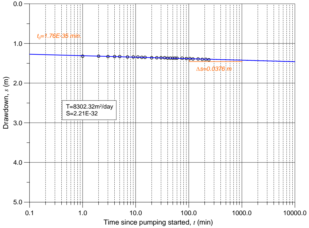
TM3_Gande Cooper-Jacobmethode
