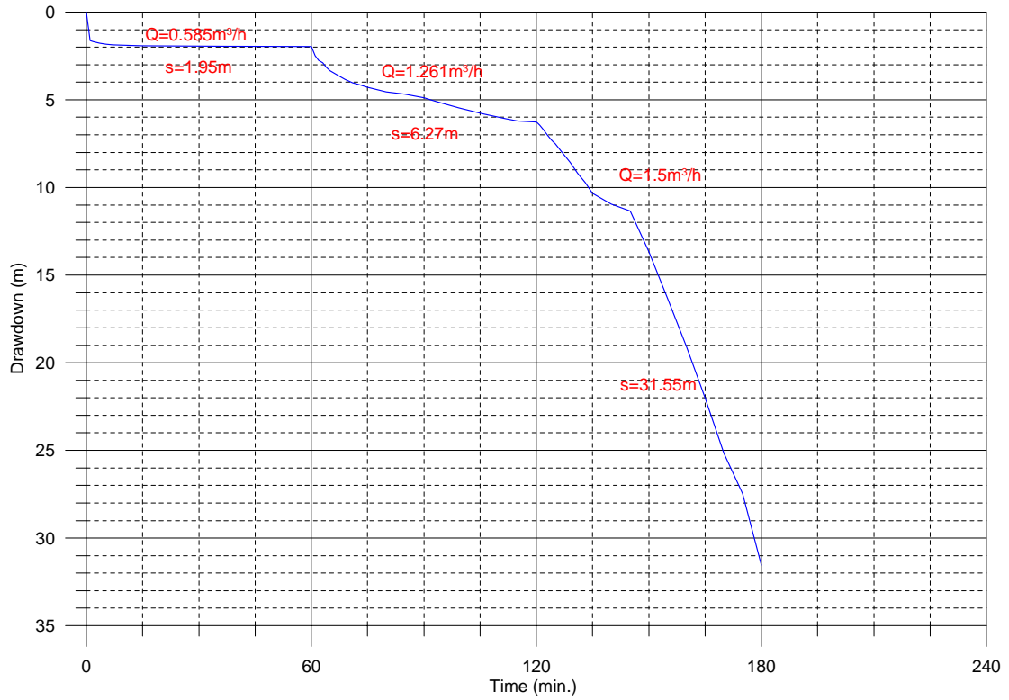
TM6_Yerimale essai palier-1
