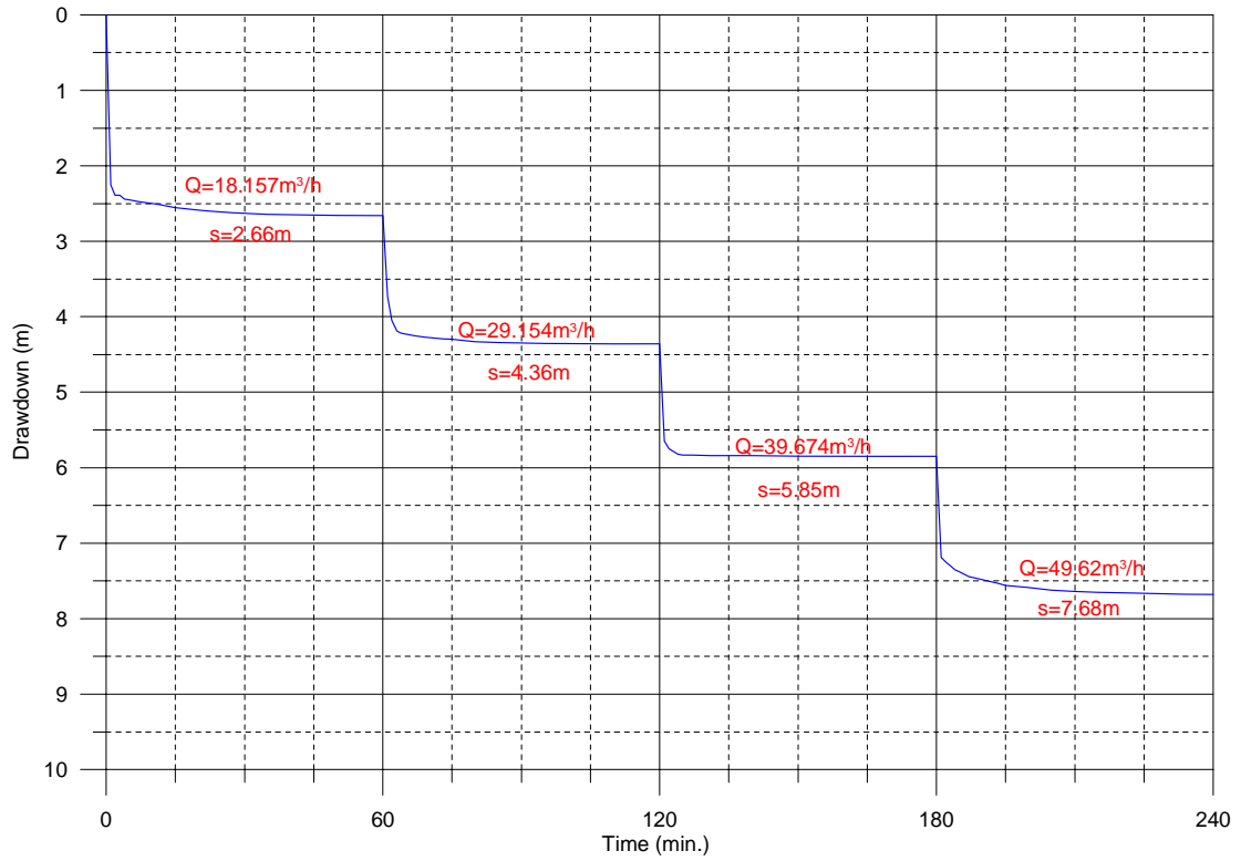
TM12_Soutouta essai palier-1
