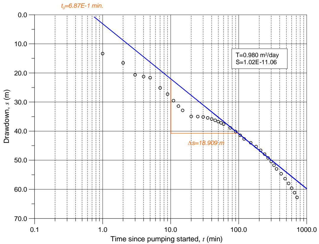
TM7_Khossanto Cooper-Jacobmethode
