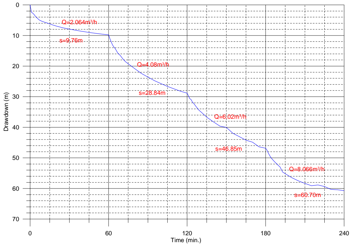
TM7_Khossanto essai palier-1
