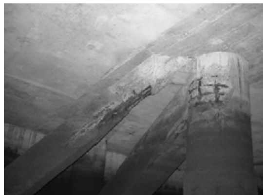
Block 2 Pile 35F-1
