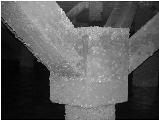
Block 2 Pile 113b
