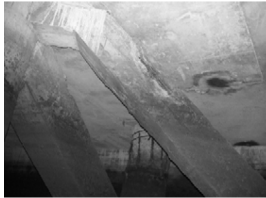
Block 2 Beam bet. Pile 20F & 109c
