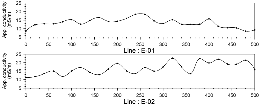
Figure.2.4.26 Geophysical survey results at Iyogelo sub-village in Ufuluma village
