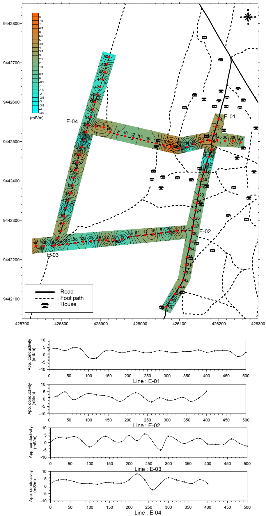
Figure.2.4.48 Geophysical survey results at Kiloleni-B sub-village in Kiloleni village
