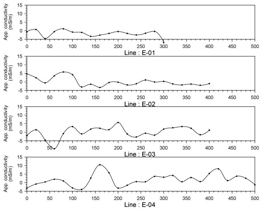
Figure.2.4.30 Geophysical survey results at Misha Kati sub-village in Misha village
