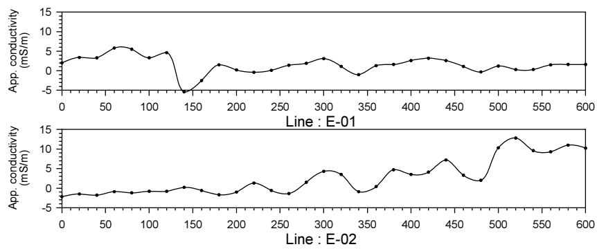
Figure.2.4.21 Geophysical survey results at Kasandalala sub-village in Kasandalala village
