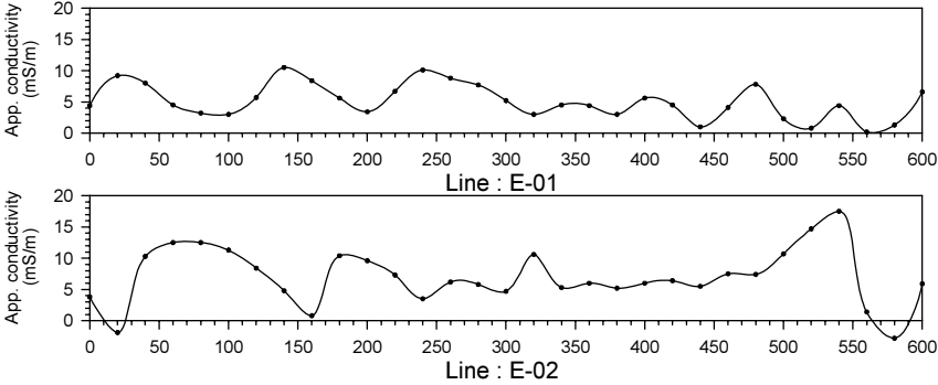
Figure.2.4.18 Geophysical survey results at Mashariki sub-village in Wela village
