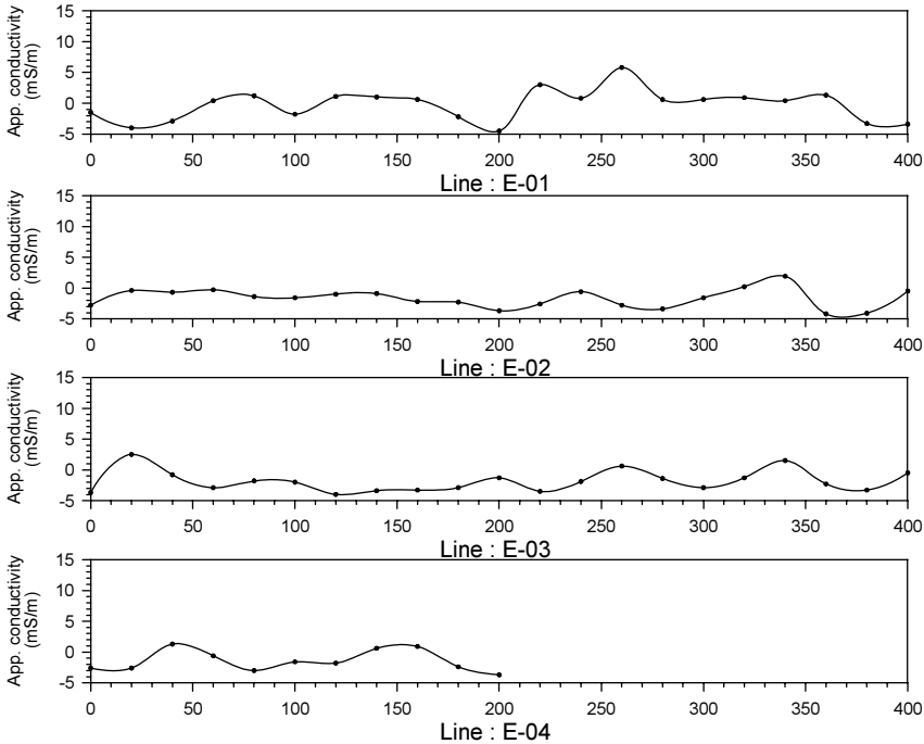
Figure.2.4.35 Geophysical survey results at Mtukula sub-village in Uyui village
