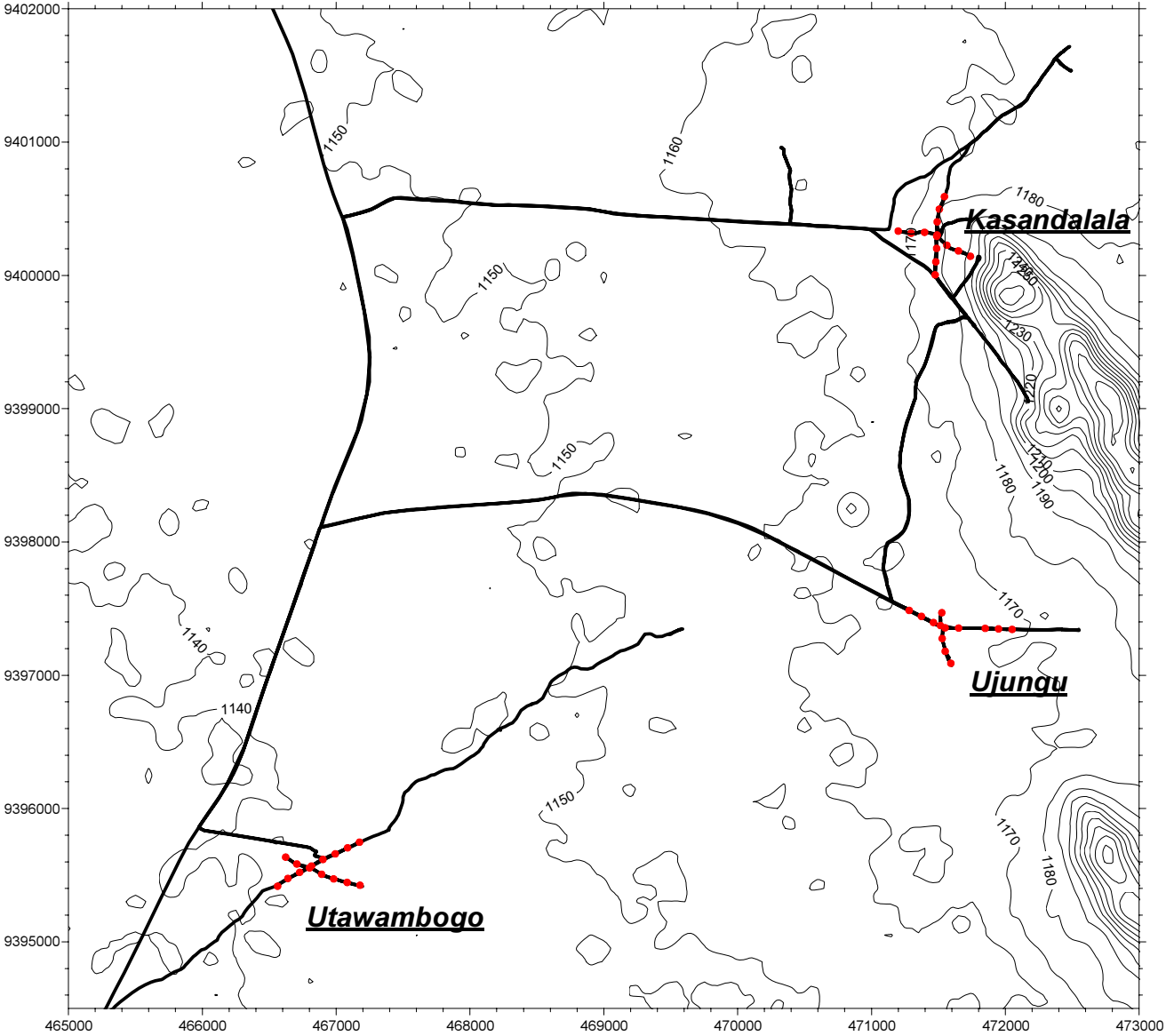
Figure.2.4.20 Geophysical survey location at Kasandalala village in Sikonge district
