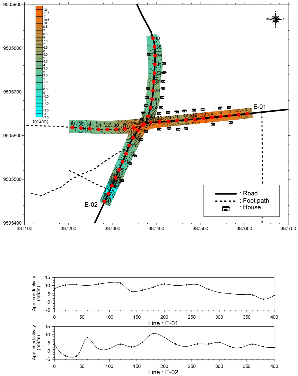
Figure.2.4.50 Geophysical survey results at Nyota sub-village in Nsungwa village
