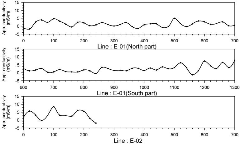
Figure.2.4.45 Geophysical survey results at Kilambo sub-village in Kapilula village
