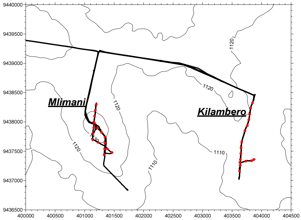
Figure.2.4.38 Geophysical survey location at Kapilula village in Urambo district
