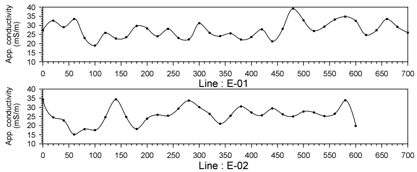
Figure.2.4.23 Geophysical survey results at Utawambogo sub-village in Kasandalala village
