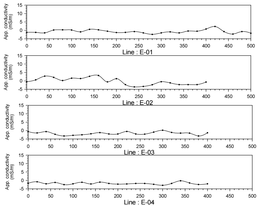
Figure.2.4.43 Geophysical survey results at Kawawa sub-village in Kalembela village
