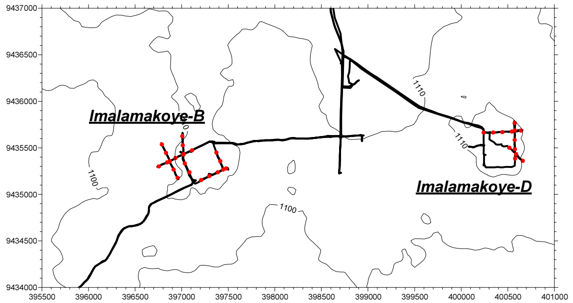
Figure.2.4.36 Geophysical survey location at Imalamakoye village in Urambo district
