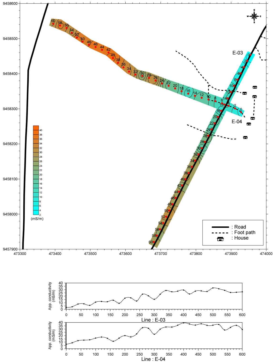
Figure.2.4.32 Geophysical survey results at Utusini sub-village southern part in Misha village
