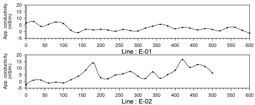
Figure.2.4.25 Geophysical survey results at Imalamapaka sub-village in Ufuluma village
