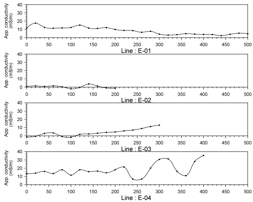
Figure.2.4.34 Geophysical survey results at Milambela sub-village in Uyui village
