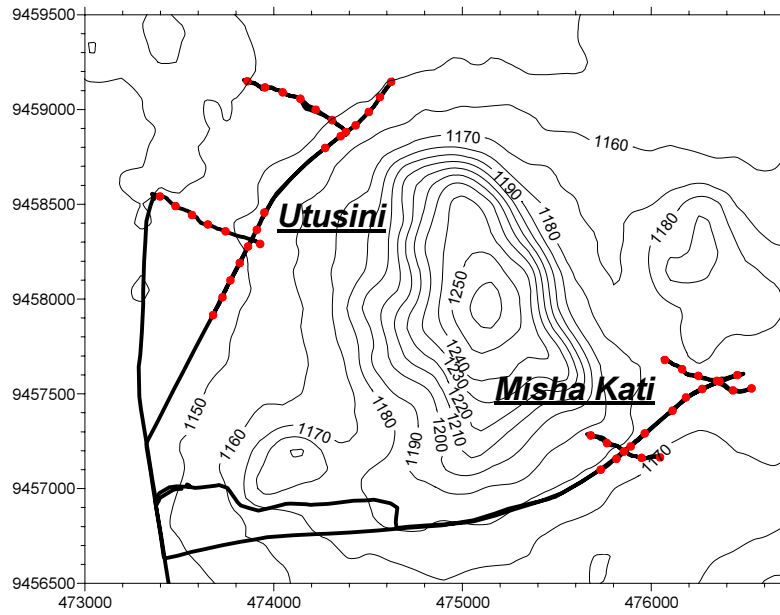
Figure.2.4.28 Geophysical survey location at Misha village in Tabora Municipality
