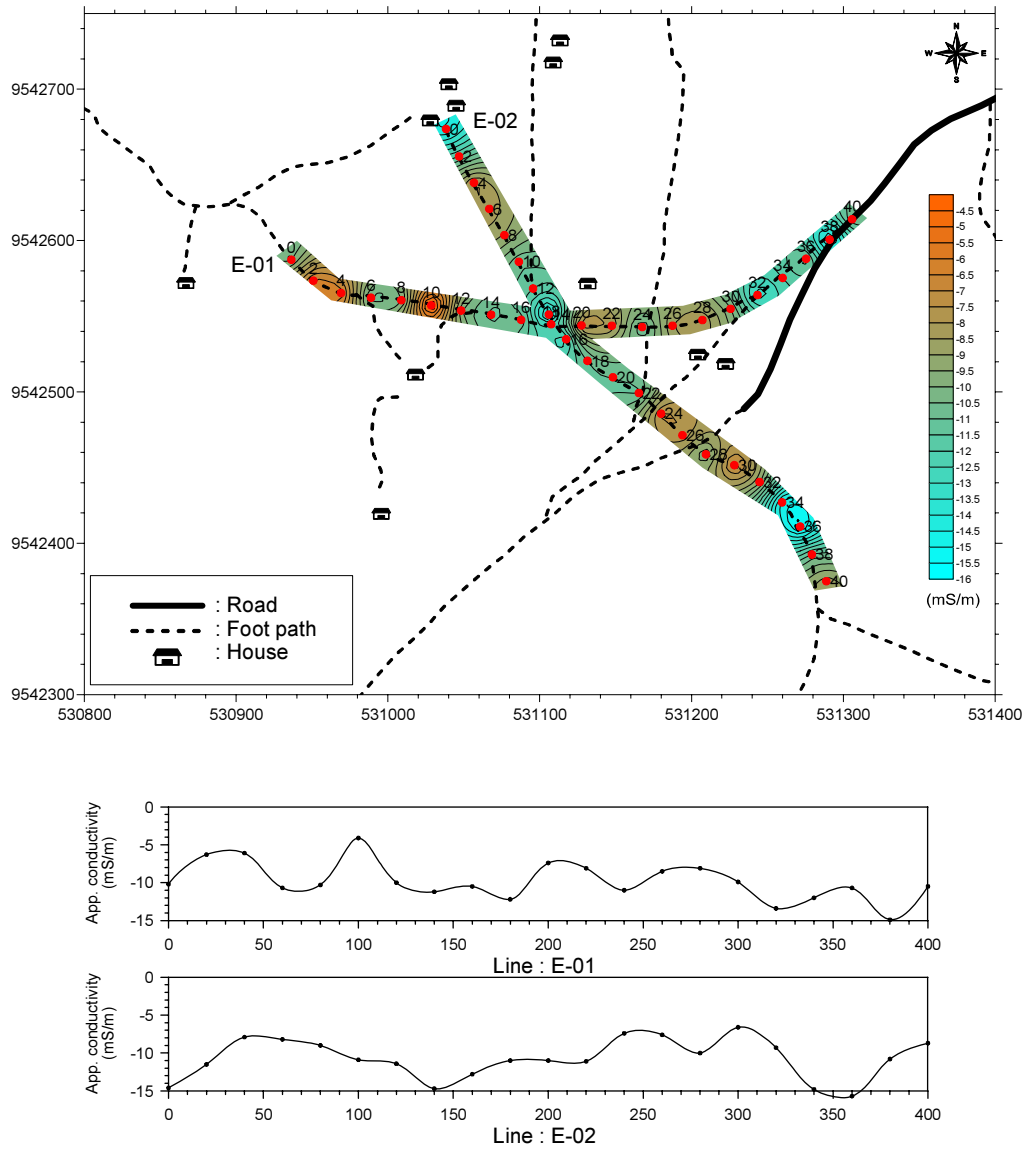
Figure.2.4.19 Geophysical survey results at Usalama sub-village in Wela village
