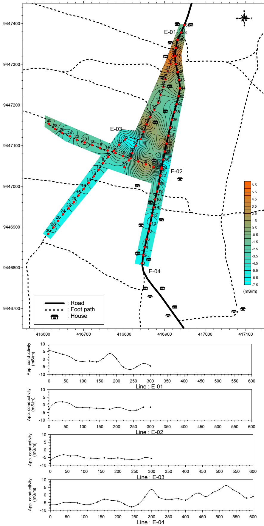
Figure.2.4.44 Geophysical survey results at Mwinye sub-village in Kalembela village
