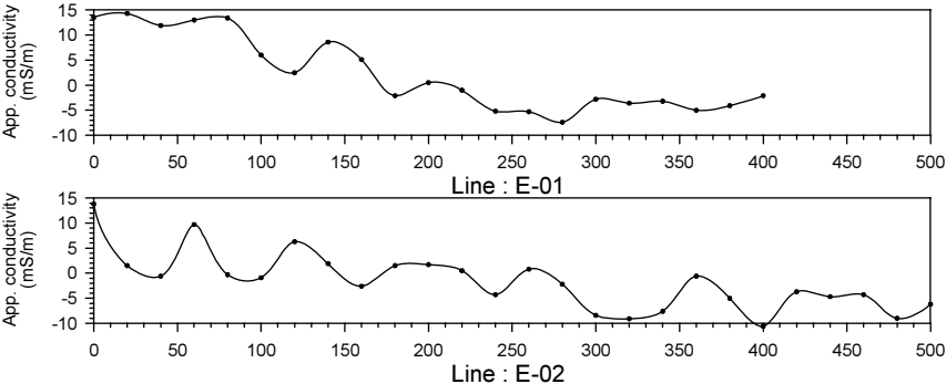
Figure.2.4.16 Geophysical survey results at Makomelo sub-village in Makomelo village
