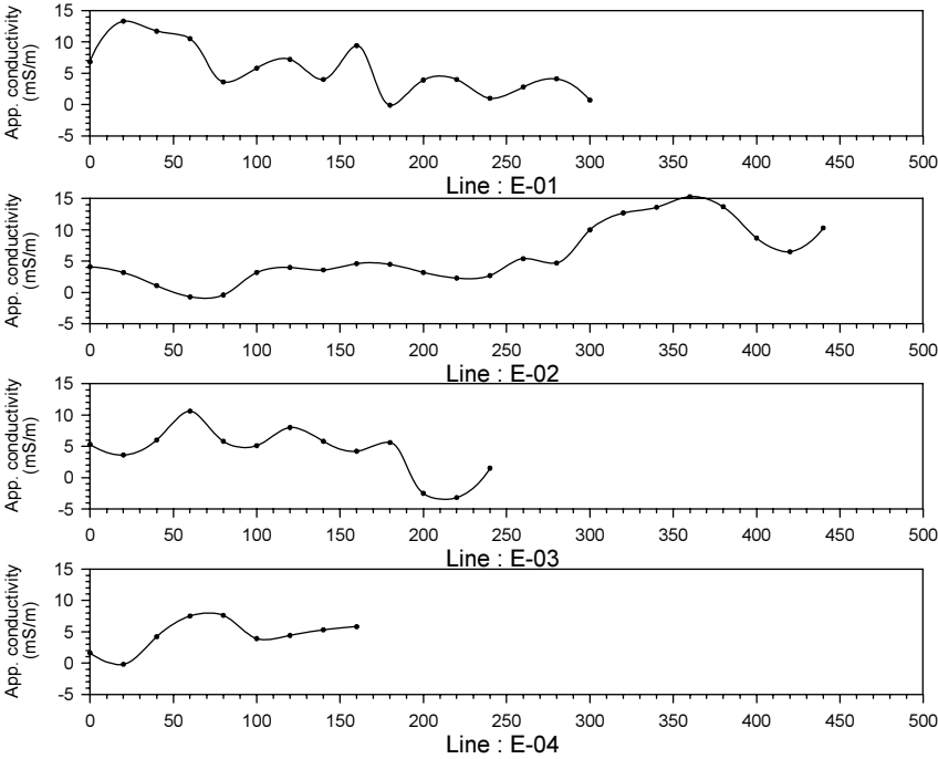
Figure.2.4.33 Geophysical survey results at Mandelo sub-village in Uyui village
