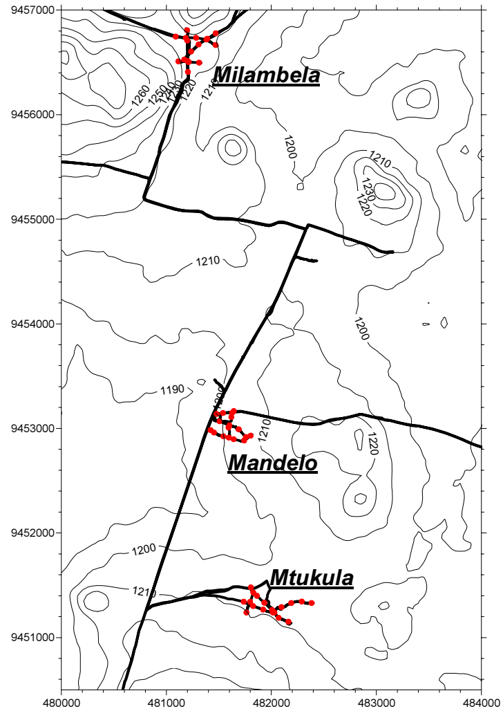
Figure.2.4.29 Geophysical survey location at Uyui village in Tabora Municipality
