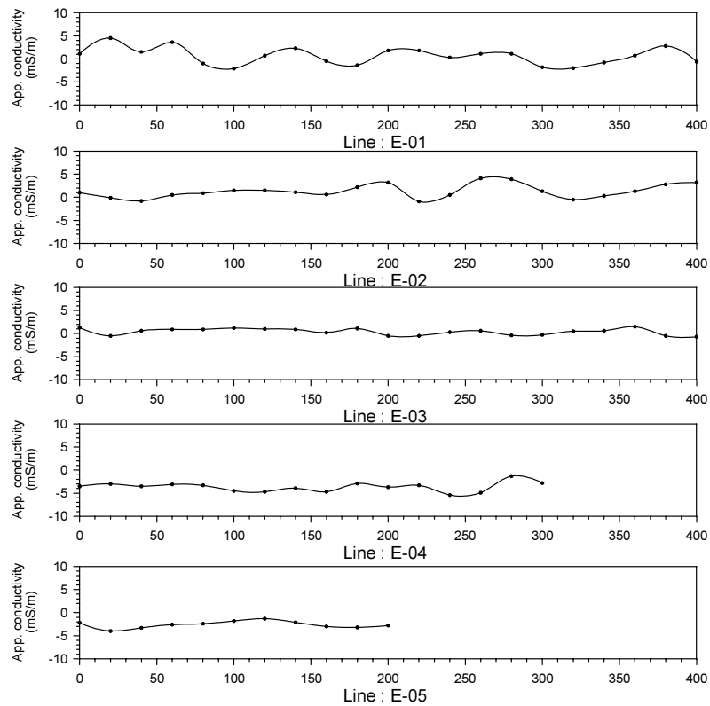
Figure.2.4.41 Geophysical survey results at Imalamakoye-B sub-village in Imalamakoye village
