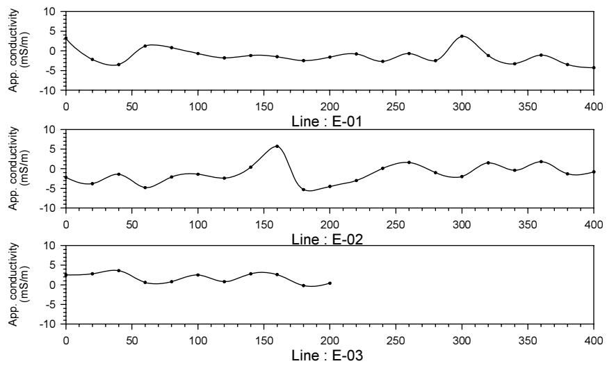
Figure.2.4.42 Geophysical survey results at Imalamakoye-D sub-village in Imalamakoye village
