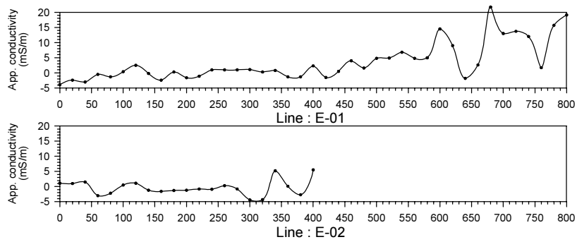
Figure.2.4.22 Geophysical survey results at Ujungu sub-village in Kasandalala village
