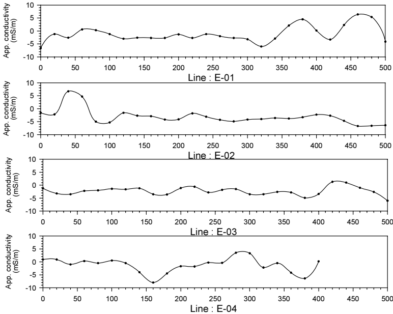
Figure.2.4.47 Geophysical survey results at Kiloleni-A sub-village in Kiloleni village
