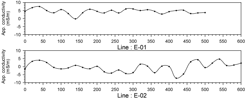
Figure.2.4.49 Geophysical survey results at Nsungwa No.7 sub-village in Nsungwa village
