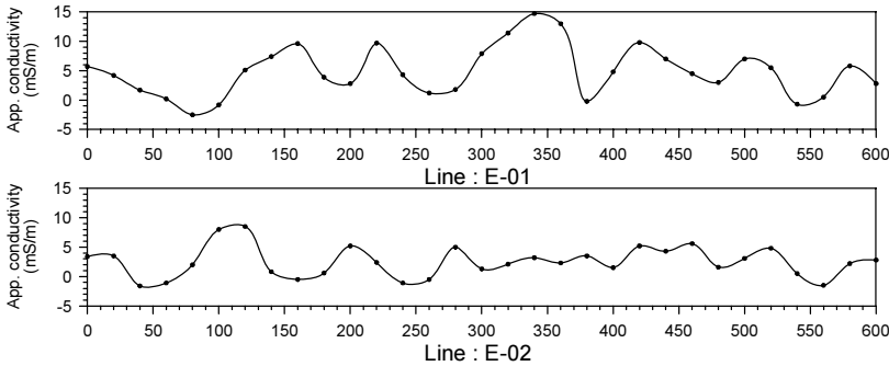
Figure.2.4.51 Geophysical survey results at Usonga sub-village in Nsungwa village
