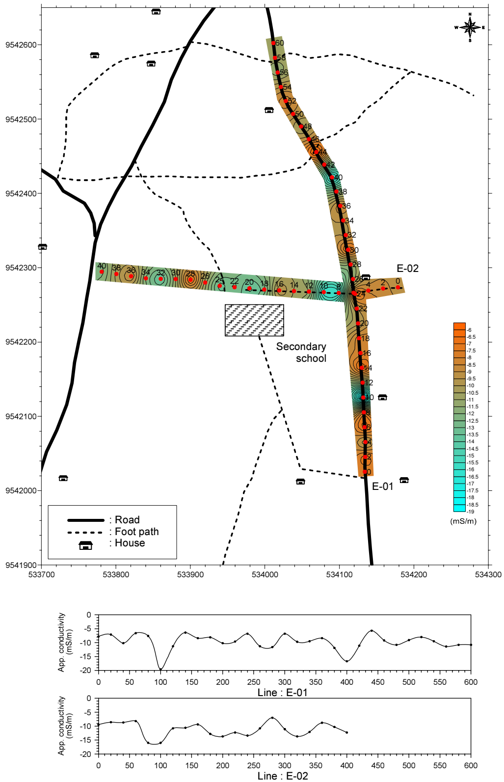
Figure.2.4.17 Geophysical survey results at Kityelo sub-village in Wela village
