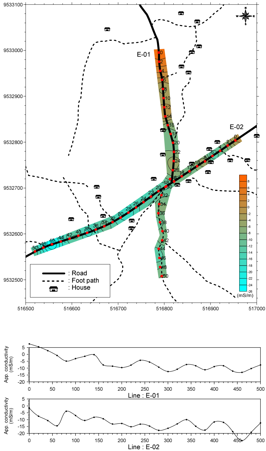
Figure.2.4.15 Geophysical survey results at Kalangale sub-village in Makomelo village
