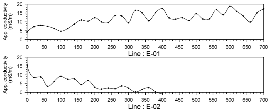
Fig.2.4.27 Geophysical survey results at Ufuluma Senta sub-village in Ufuluma village
