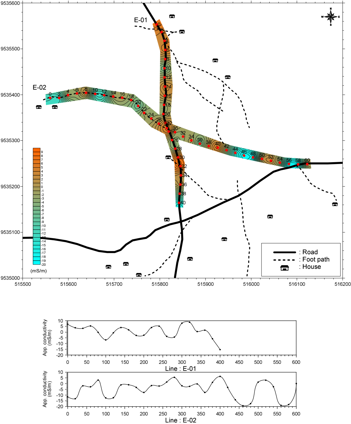
Figure.2.4.14 Geophysical survey results at Idubula sub-village in Makomelo village
