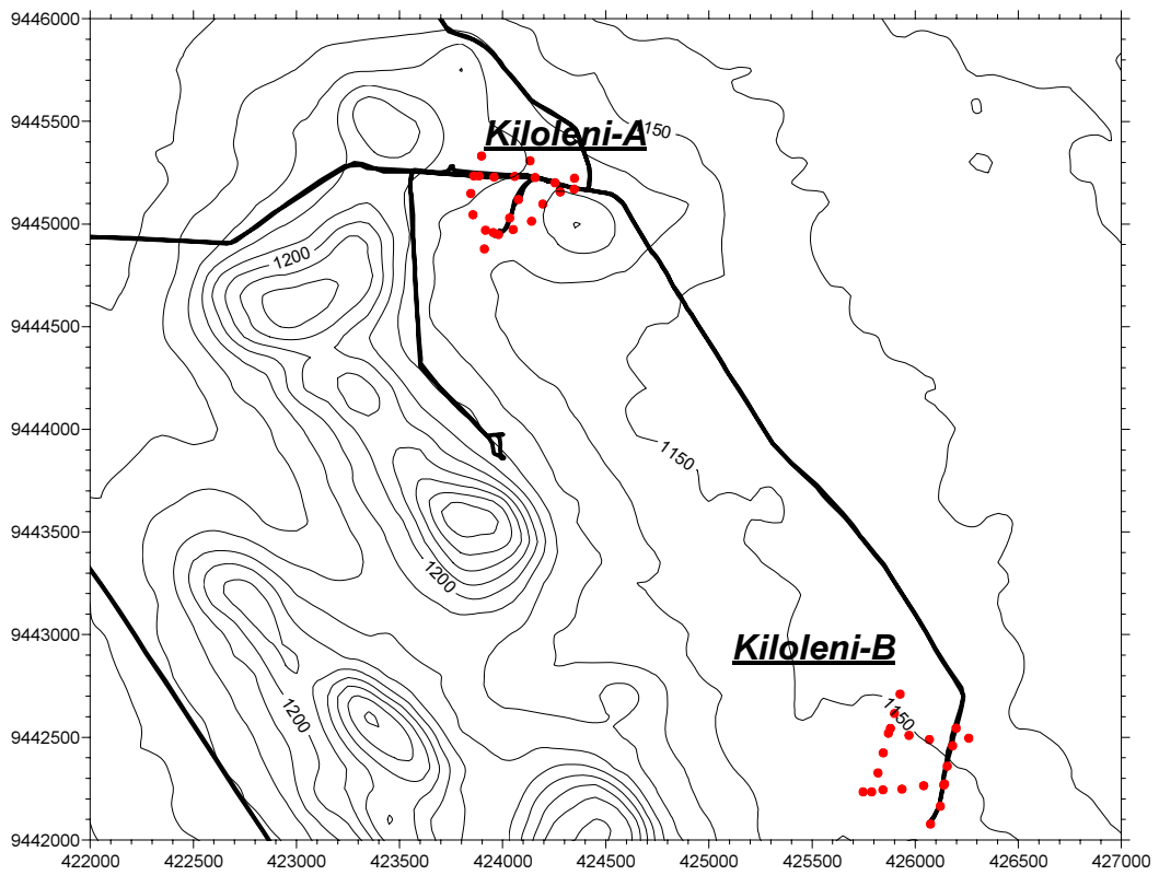
Figure.2.4.39 Geophysical survey location at Kiloleni village in Urambo district
