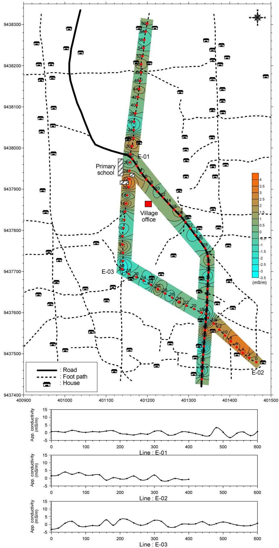
Figure.2.4.46 Geophysical survey results at Mlimani sub-village in Kapilula village
