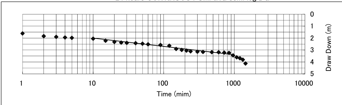
24 hours CONTINUOUS PUMPING semi log DG
