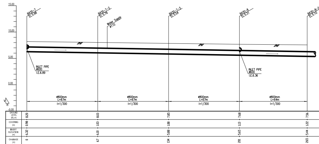
PROFILE (Manhole No. fr. B430-7 to B430-8-2)
