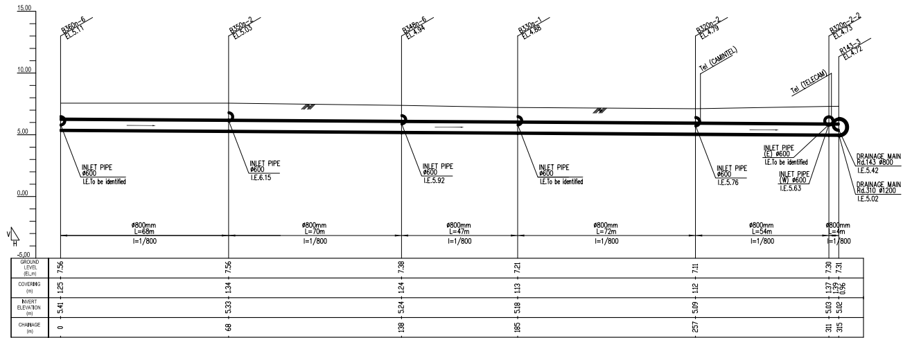
PROFILE (Manhole No. fr. B360n-6 to R143-3) H: SCALE A V: SCALE B
