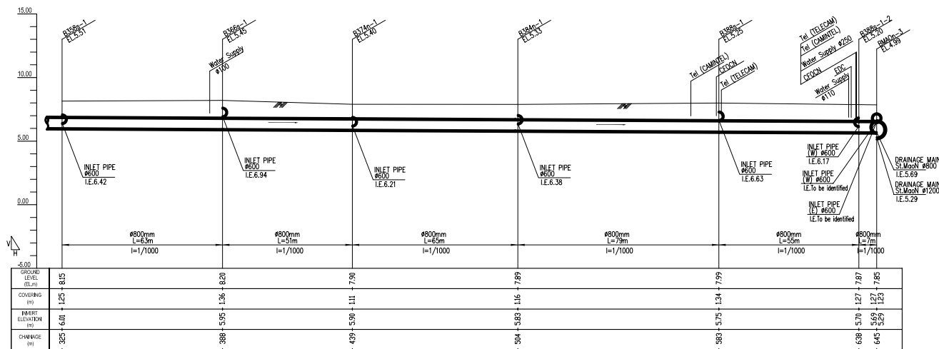
PROFILE (Manhole No. fr. B358s-1 to BMAOn-3)
