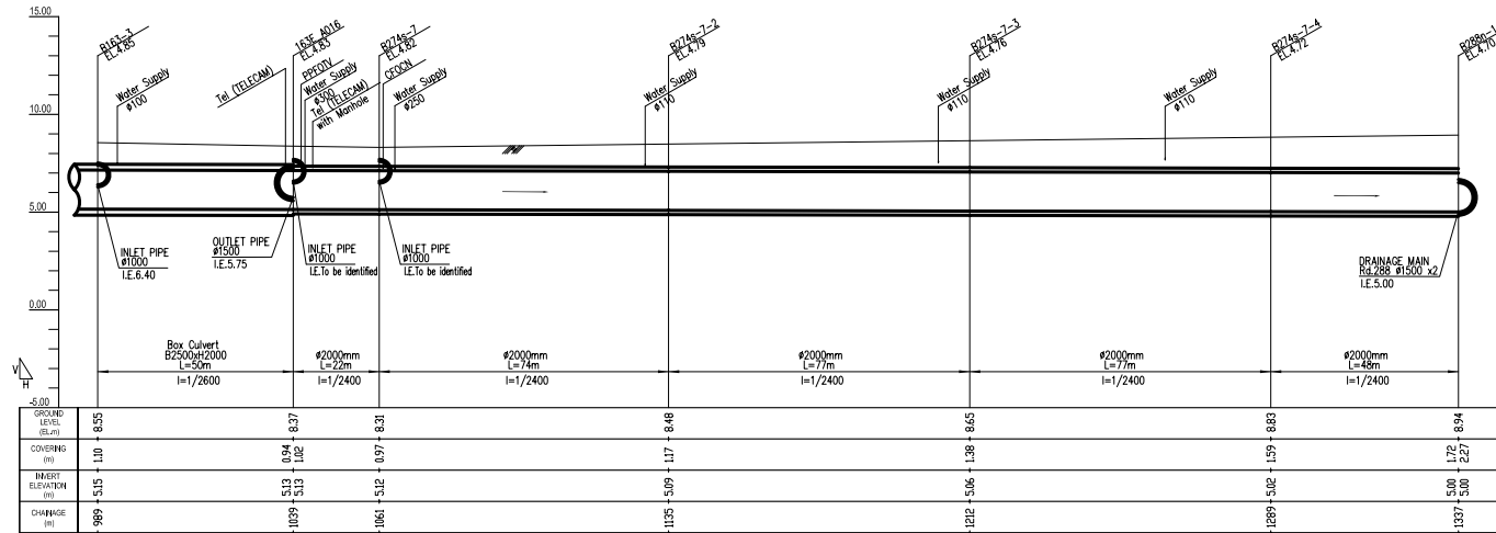
PROFILE (Manhole No. fr. B163-3 to B288n-1)
