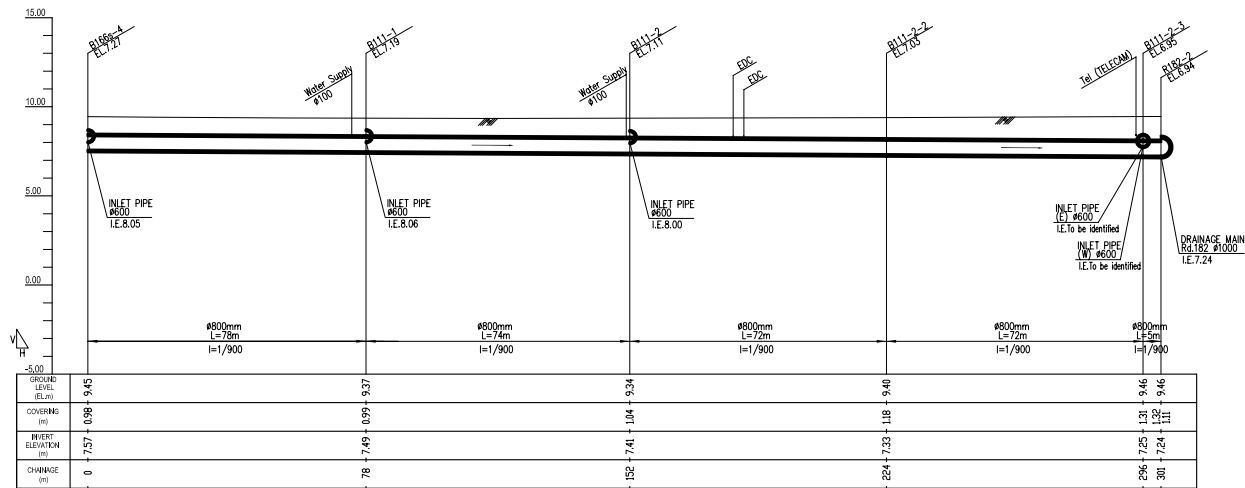
PROFILE (Manhole No. fr. B166s-4 to 182-2) H: SCALE A V: SCALE B
