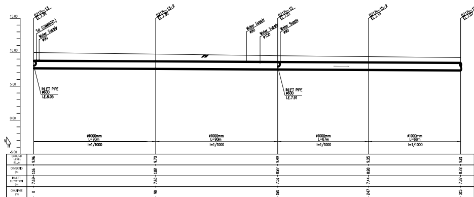
PROFILE (Manhole No. fr. B217n-13 to B217n-15-3)
