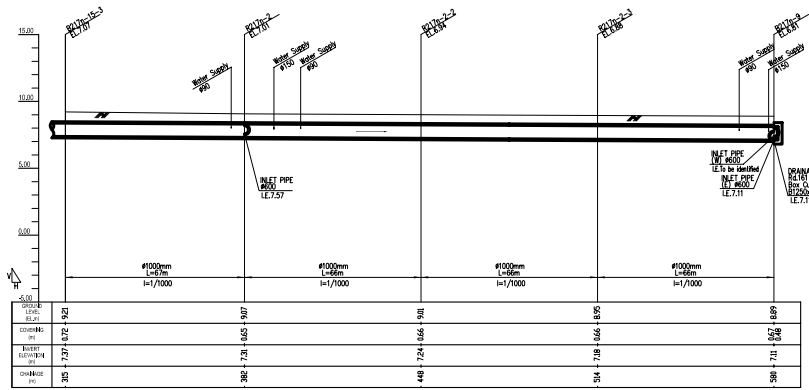
PROFILE (Manhole No. fr. B217n-15-3 to B217n-19) H: SCALE B V: SCALE C
