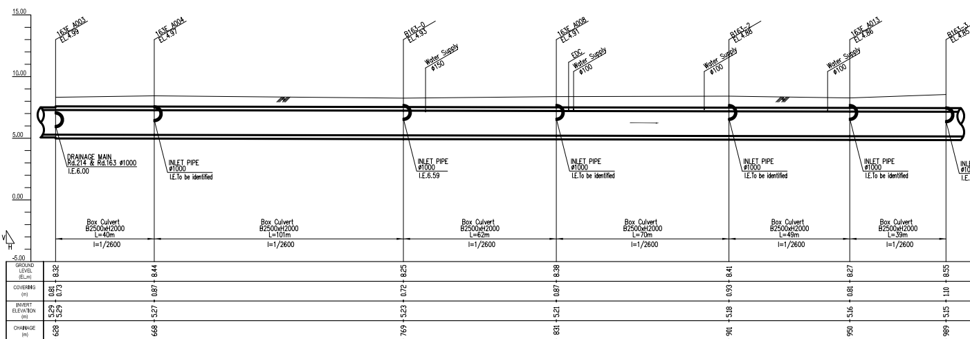
PROFILE (Manhole No. fr. 163E_A003 to B163-3)
