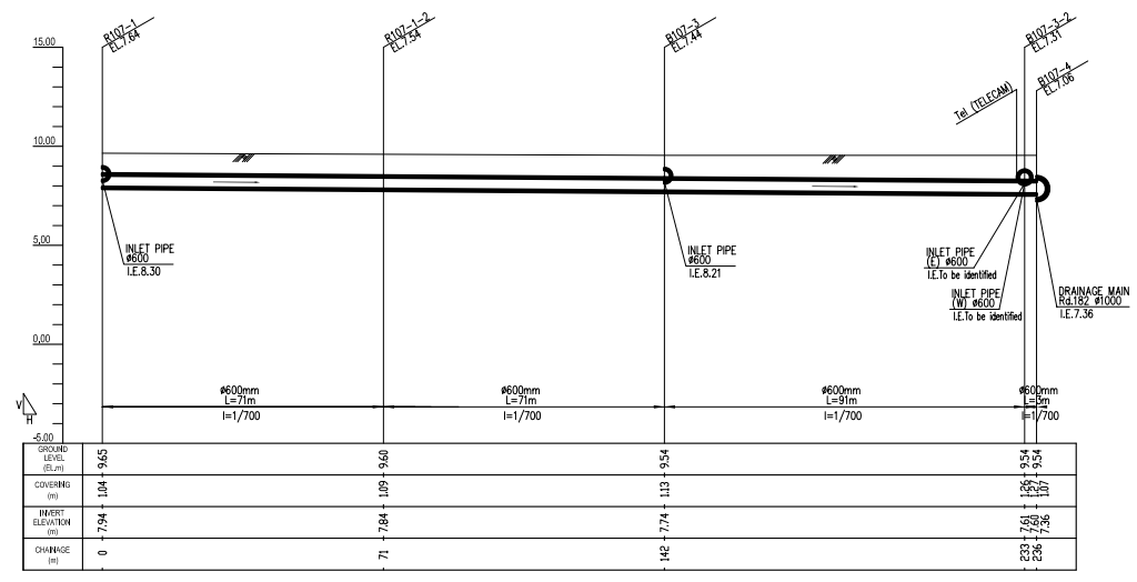
PROFILE (Manhole No. fr. R107-1 to R107-4) H: SCALE A V: SCALE B
