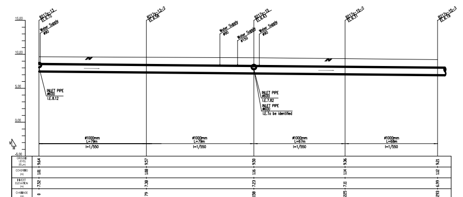
PROFILE (Manhole No. fr. B217s-13 to B217s-15-3)
