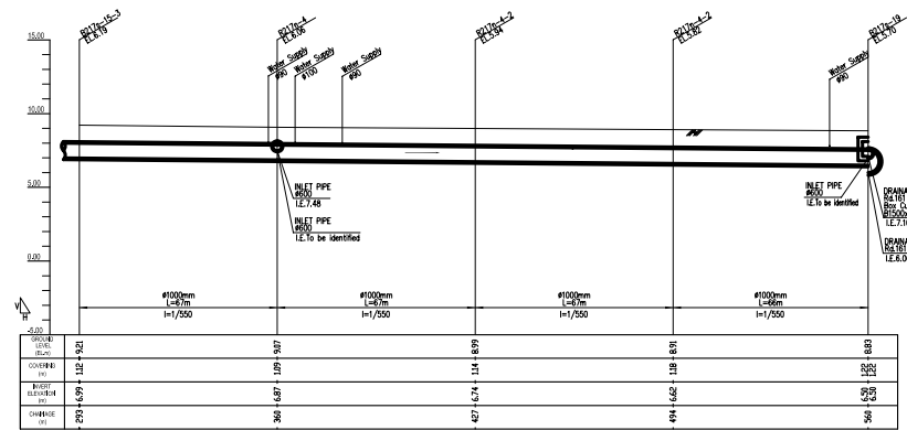
PROFILE (Manhole No. fr. B217s-15-3 to B217s-19) H: SCALE B V: SCALE C
