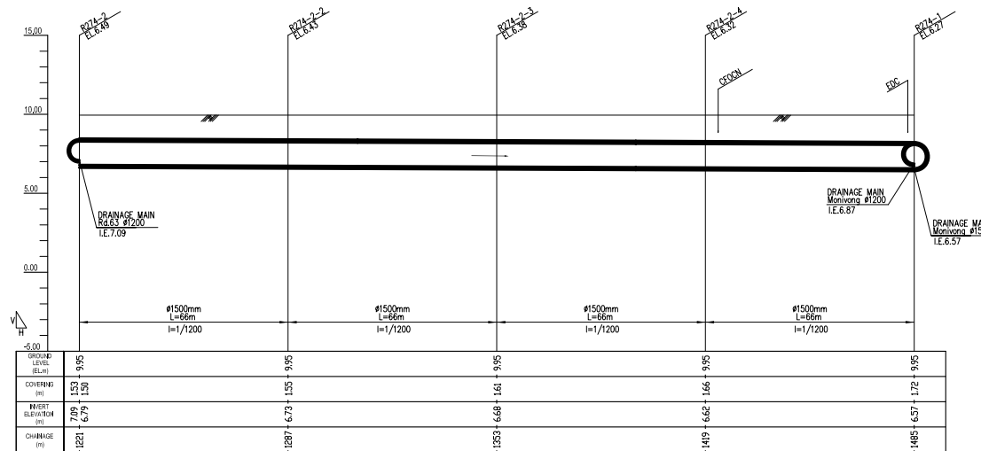
PROFILE (Manhole No. fr. R274-2 to R274-1) H: SCALE A V: SCALE B
