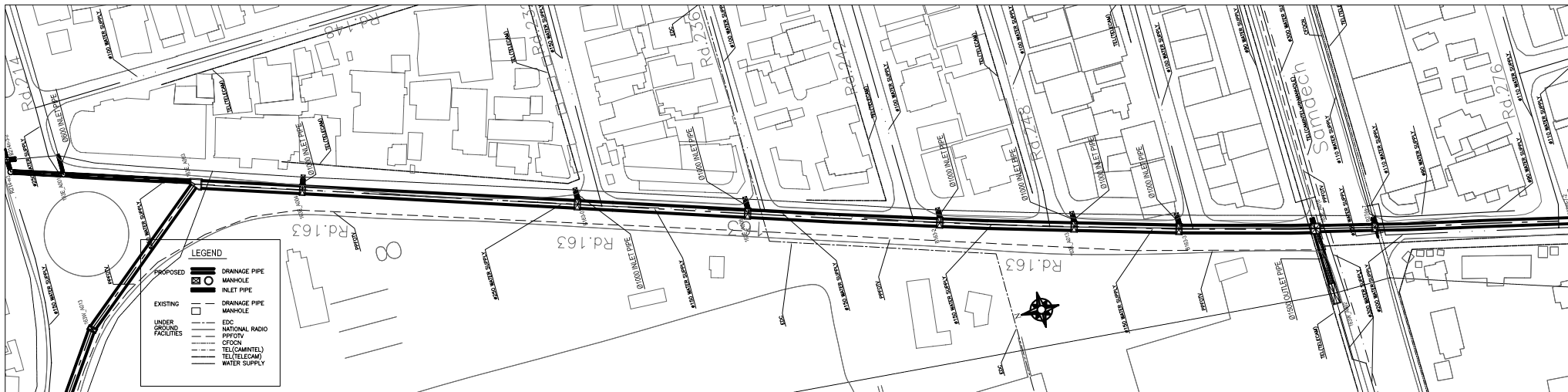
PLAN (Manhole No. fr. 163E_A003 to B163-3)
