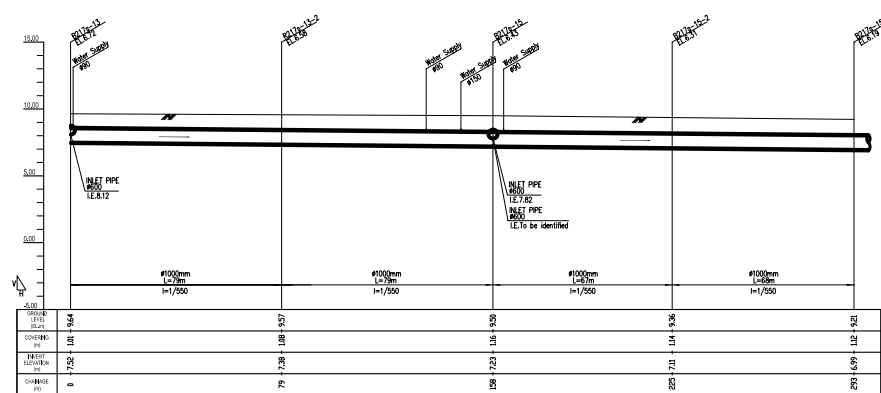
PROFILE (Manhole No. fr. B217s-13 to B217s-15-3)
