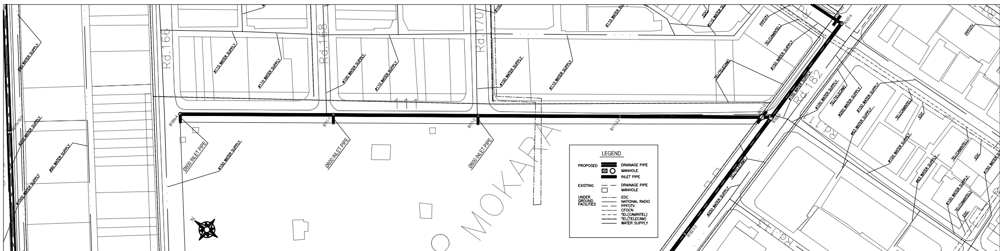
PLAN (Manhole No. fr. B1166s-4 to R182-2)
