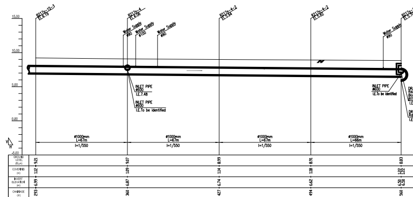
PROFILE (Manhole No. fr. B217s-15-3 to B217s-19)
