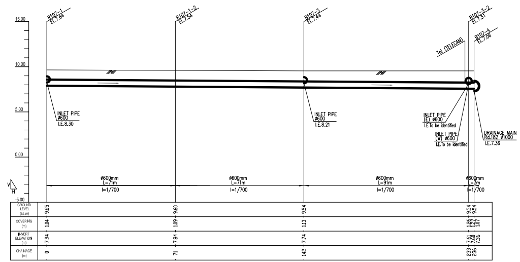
PROFILE (Manhole No. fr. R107-1 to R107-4) H: SCALE A V: SCALE B
