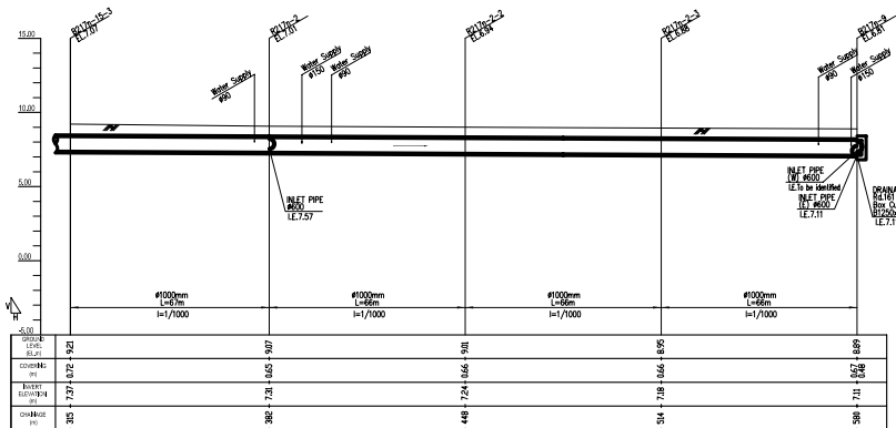
PROFILE (Manhole No. fr. B217n-15-3 to B217n-19)
