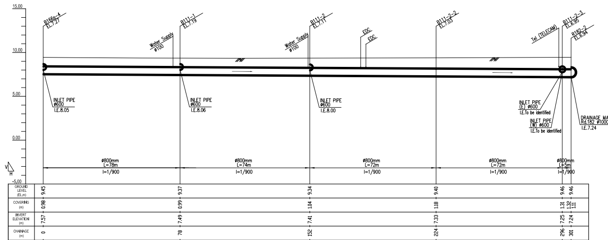
PROFILE (Manhole No. fr. B1166s-4 to 182-2)
