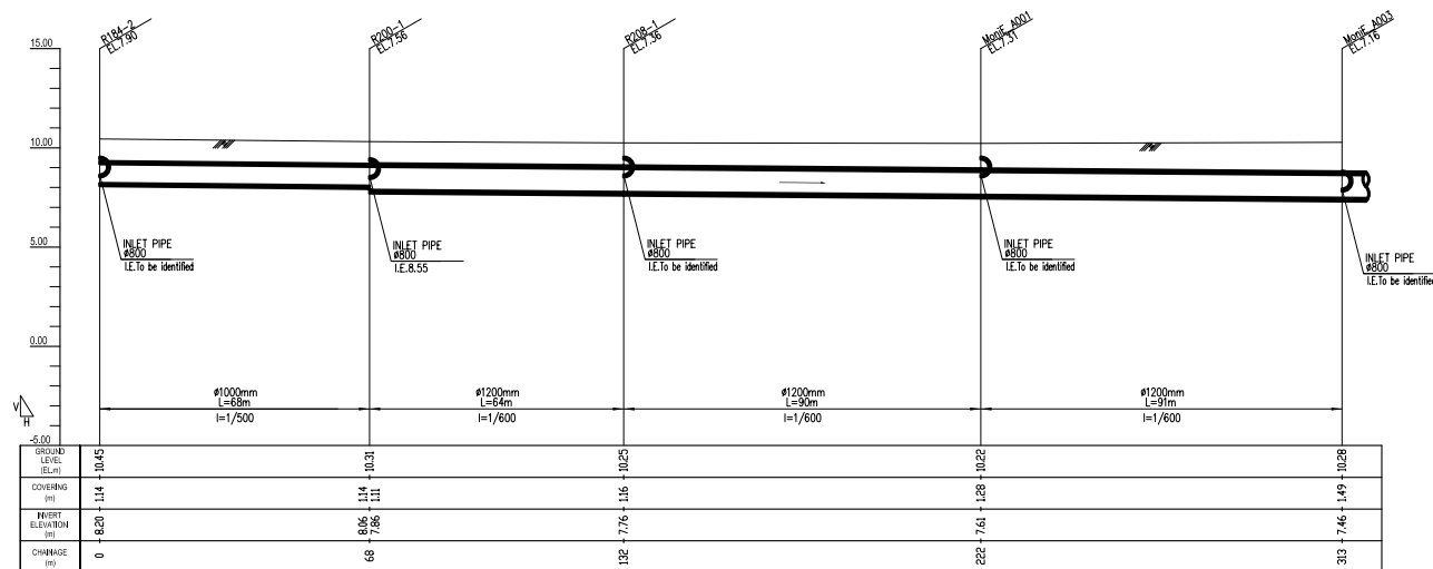
PROFILE (Manhole No. fr. R184-2 to MoniE_A003)
