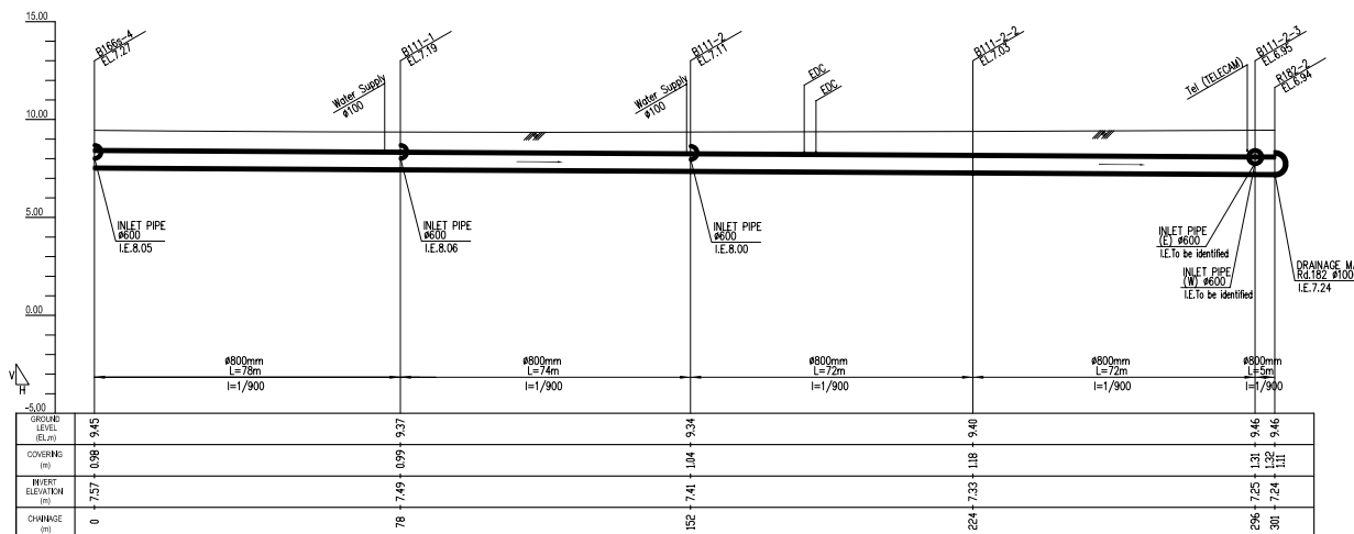
PROFILE (Manhole No. fr. B166s-4 to 182-2)
