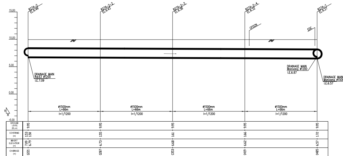
PROFILE (Manhole No. fr. R274-2 to R274-1)
