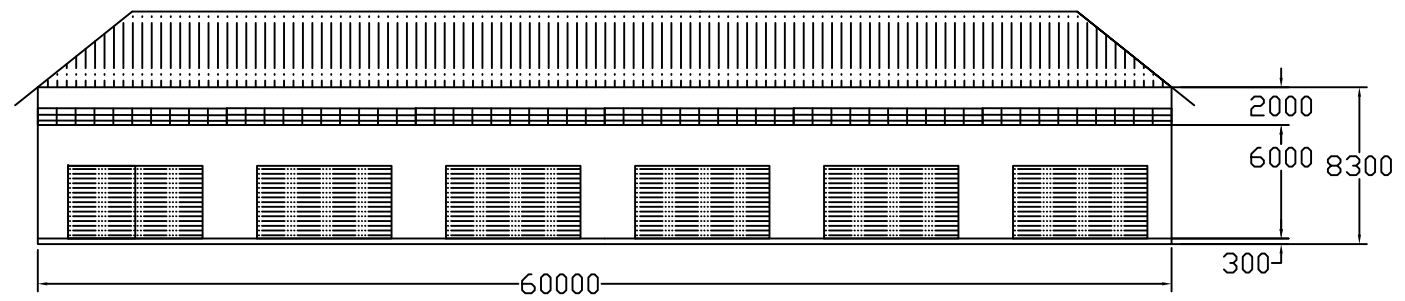
① Front View ECH 1: 400
