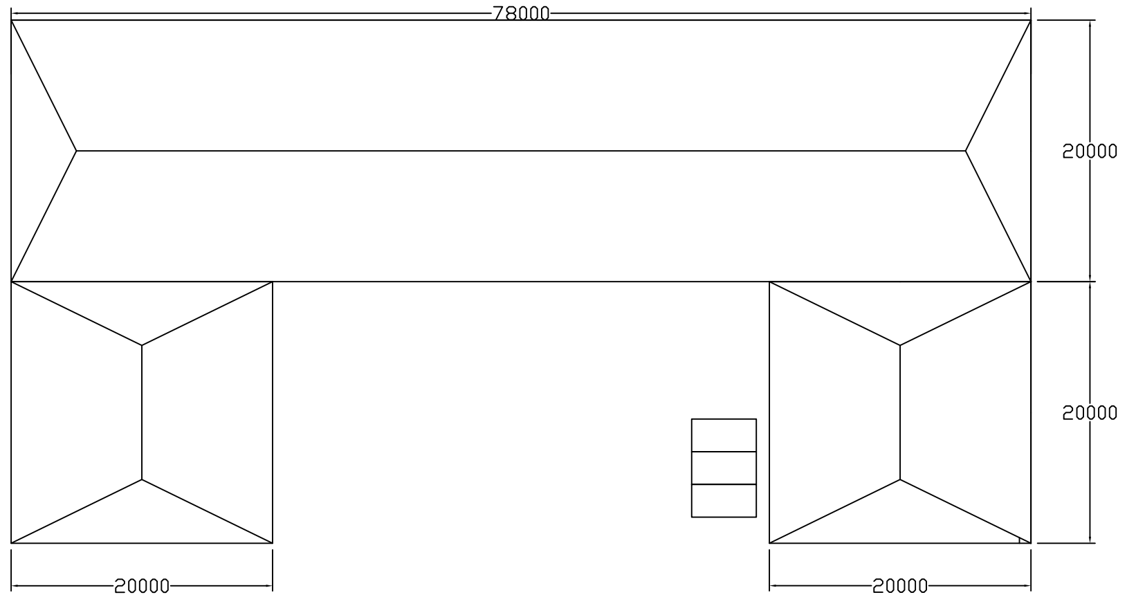
○ Top View ECH 1: 400
