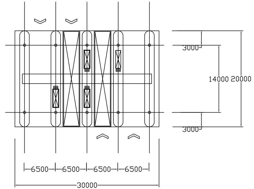
① Top View ECH 1: 400
