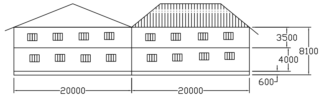
② Side View ECH 1: 400
