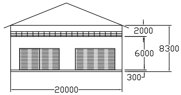
② Side View ECH 1: 400
