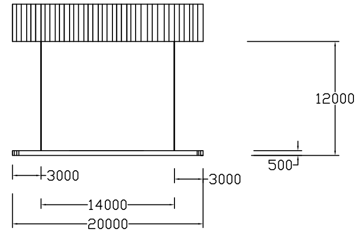
② Side View ECH 1: 400
