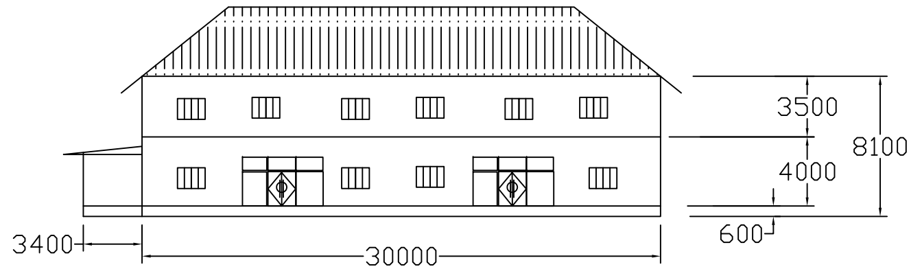
① Front View ECH 1: 300
