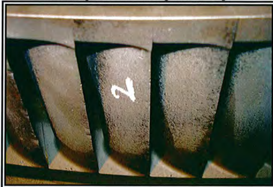
Photo 2 IP Rotating Blade – Surface Roughness of 2 nd Stage
