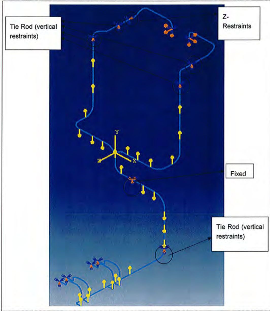
Figure 11.4: Restraints in the model
