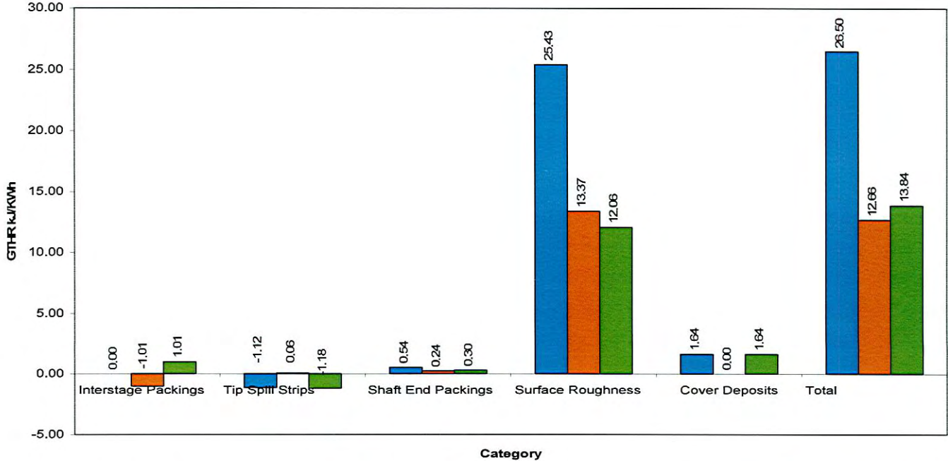
Figure 4 Changes in Heat Rate – IP Turbine
