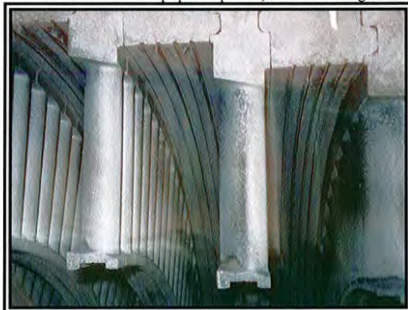
Photo 18 IP –Condition of Tip spill strip fins in 3 rd , 4 th , 5 th stage
