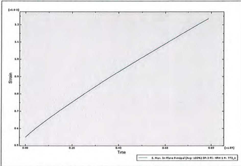
Figure 11.10: Creep strain accumulated over a period of 25 years (point A indicated in figure 11.9)
