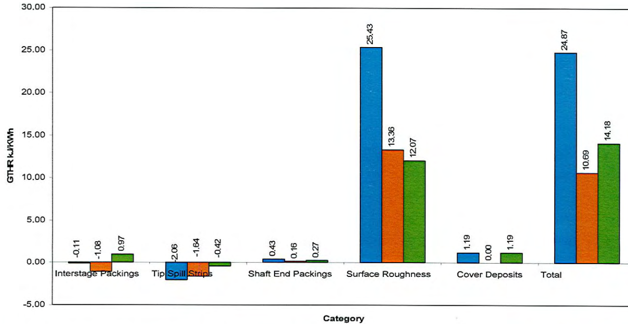
Figure 6 Changes in Heat Rate – IP Generator
