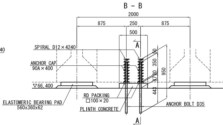
DETAILS SCALE 1:20
