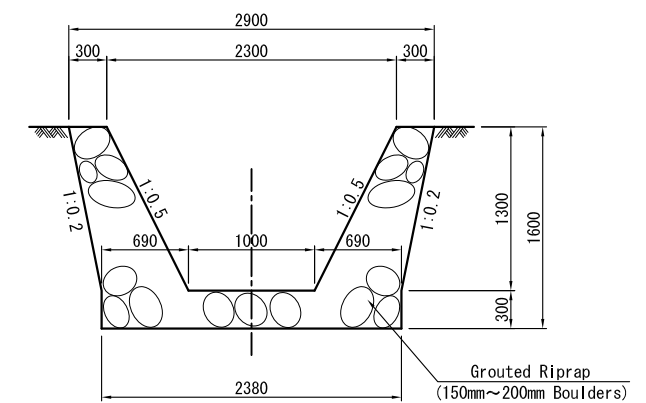
2-2 SECTION
