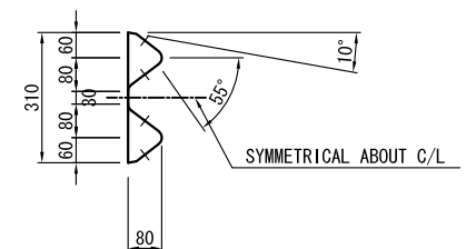
SECTION THROUGH W-BEAM S=1:10
