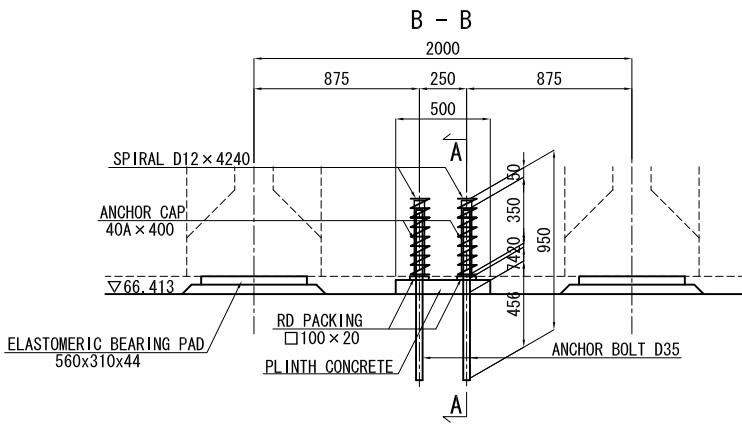
DETAILS SCALE 1:20
