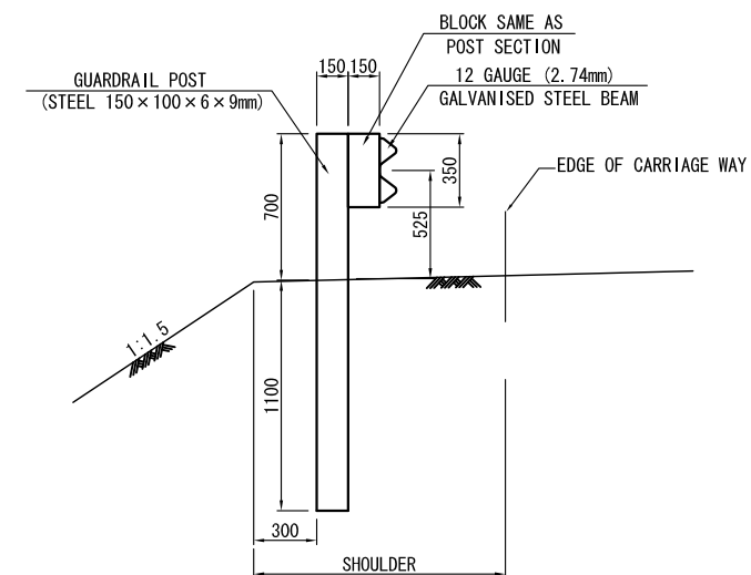
TYPICAL POST
