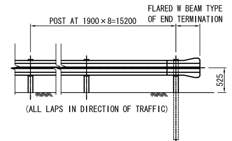
FRONT VIEW S=1:40
