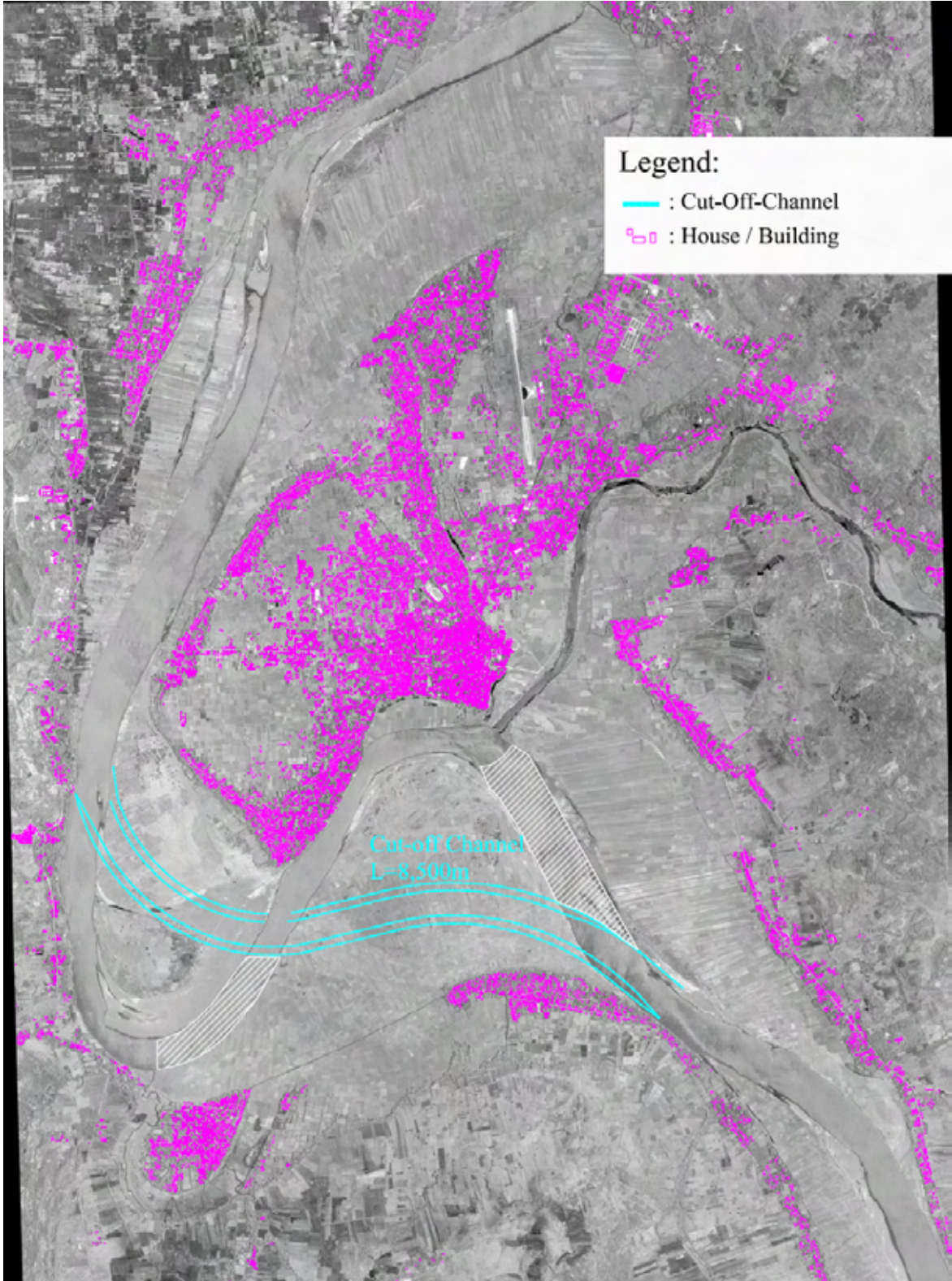
Figure7.3 Cagayan River Improvement Plan (Alternative C-3: Cut-Off Channel)
