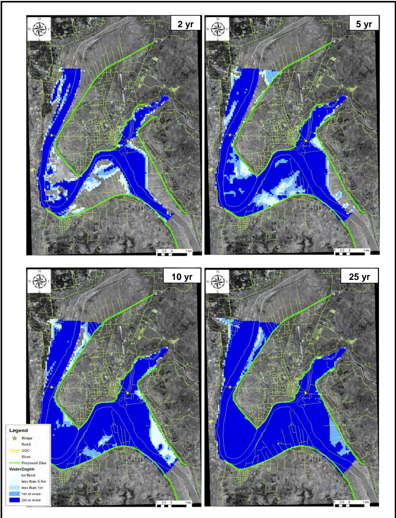
Figure 7.6 Result of Flood Inundation Analysis (With Alt-C2)
