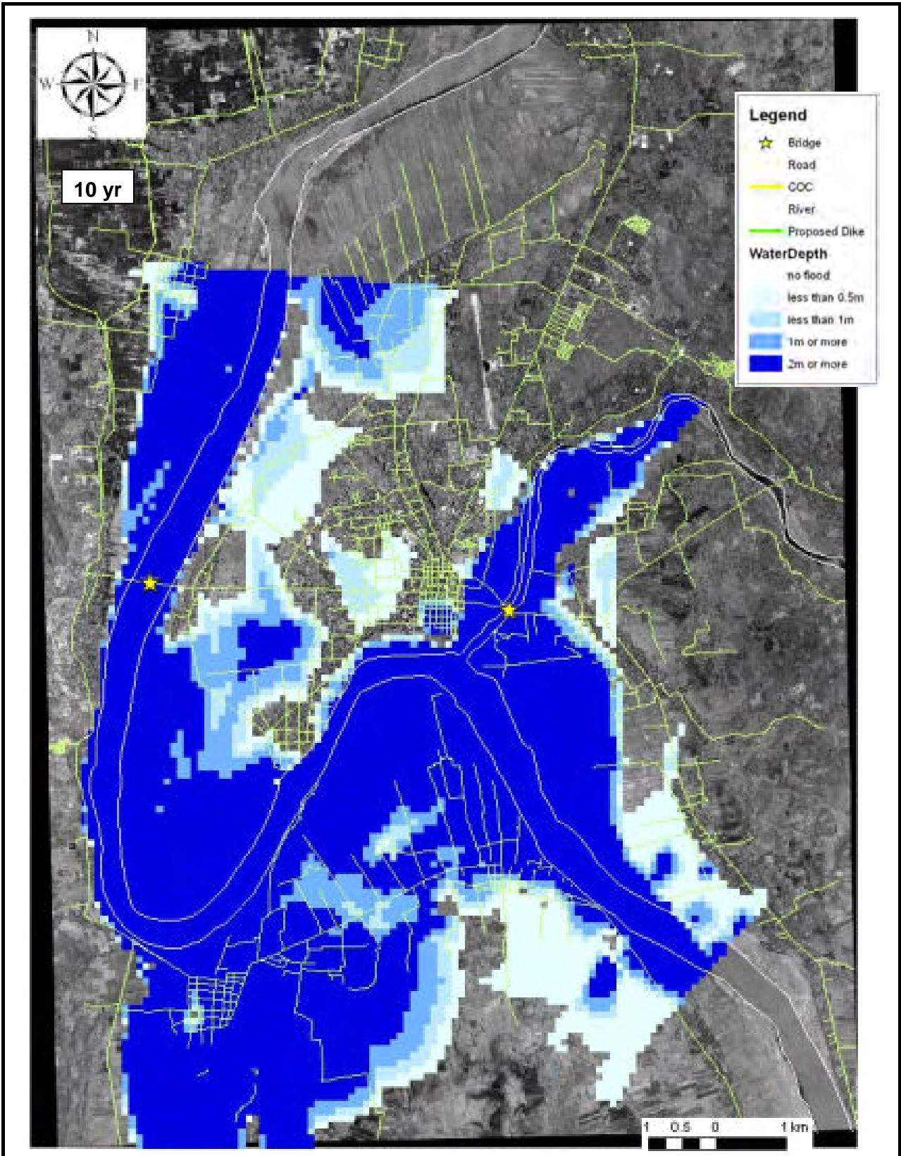
Figure 7.4 (3/6) Result of Flood Inundation Analysis (Without Project)
