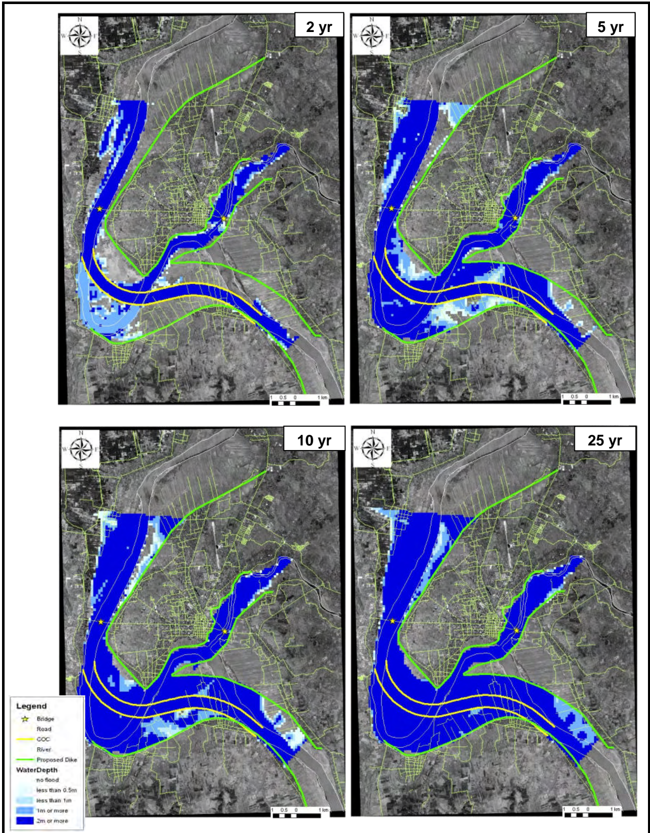
Figure 7.5 Result of Flood Inundation Analysis (With Alt-C1)
