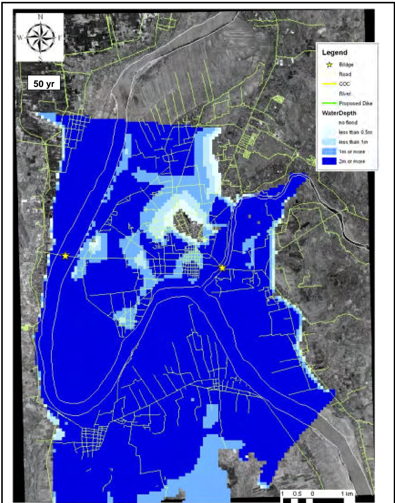
Figure 7.4 (5/6) Result of Flood Inundation Analysis (Without Project)
