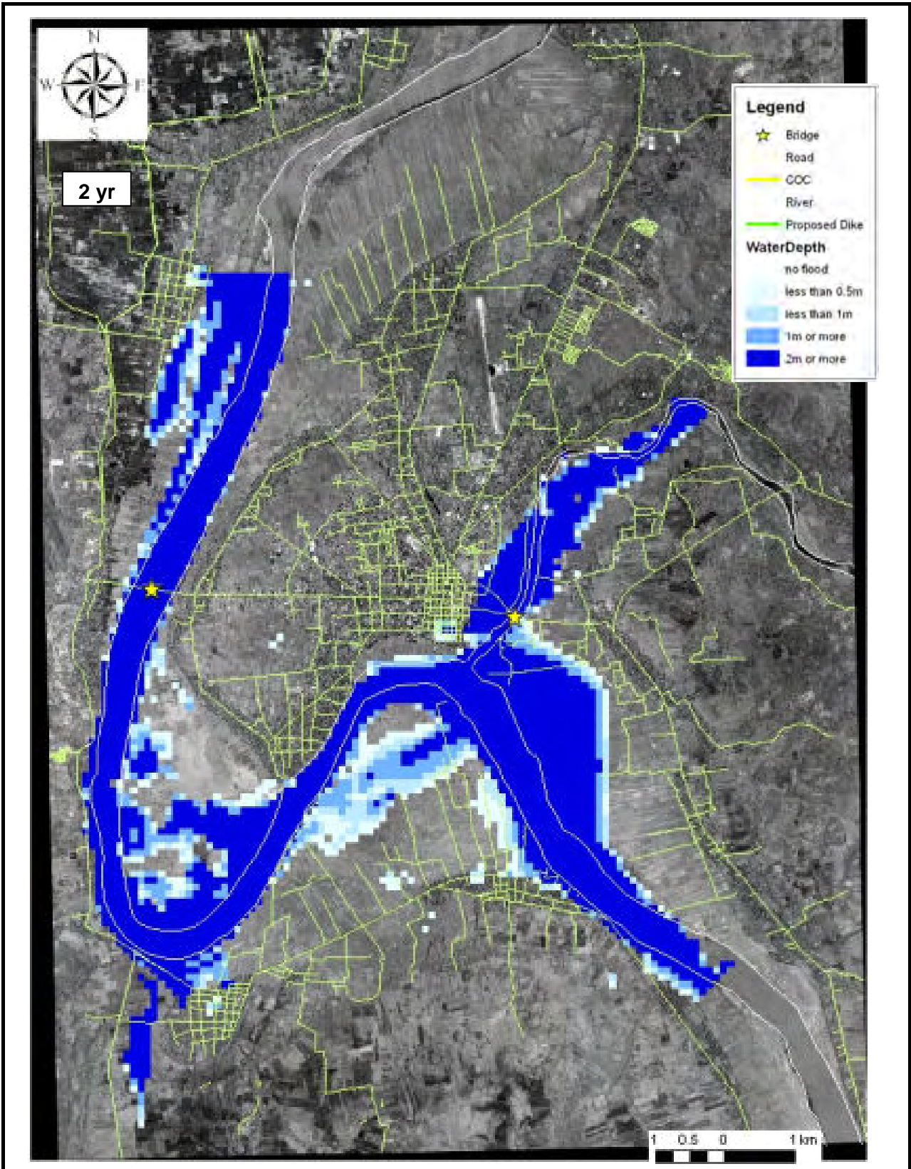
Figure 7.4 (1/6) Result of Flood Inundation Analysis (Without Project)
