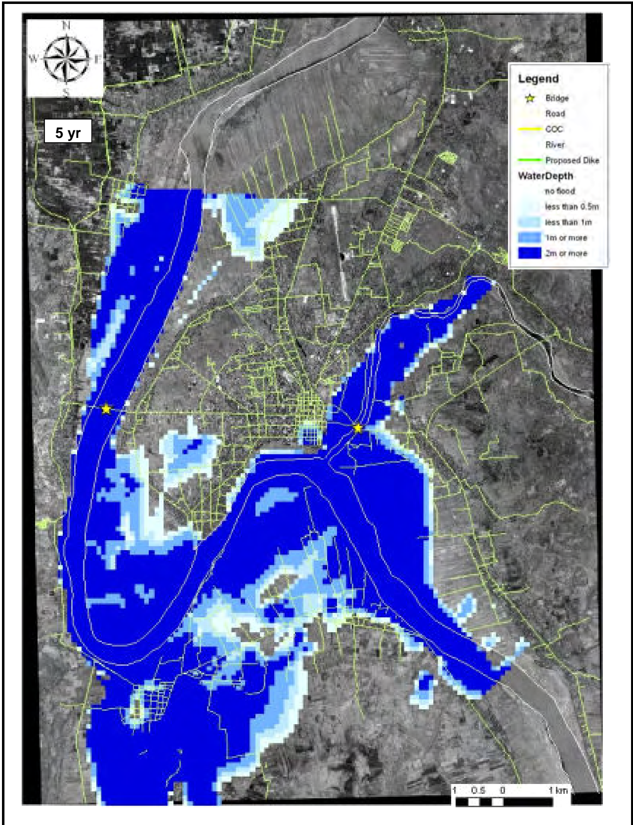
Figure 7.4 (2/6) Result of Flood Inundation Analysis (Without Project)
