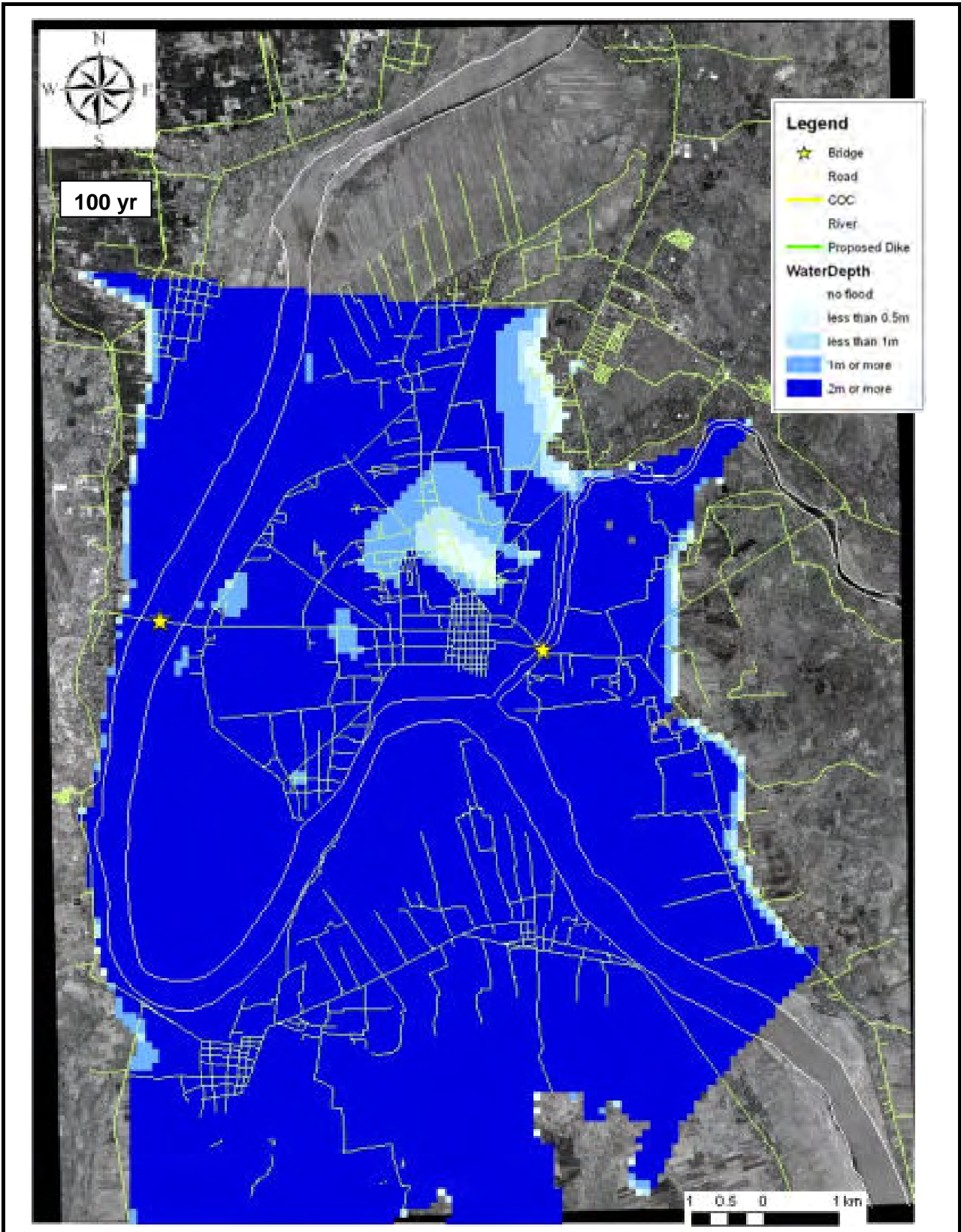
Figure 7.4 (6/6) Result of Flood Inundation Analysis (Without Project)
