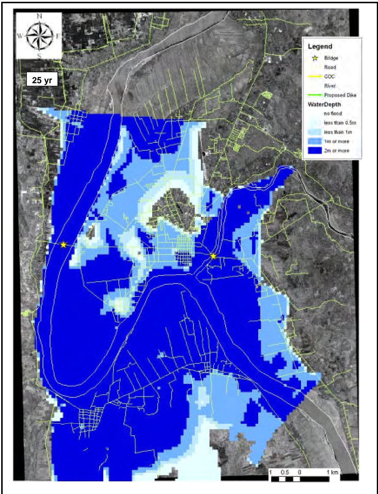
Figure 7.4 (4/6) Result of Flood Inundation Analysis (Without Project)
