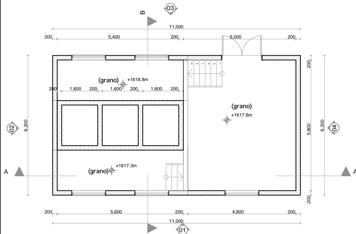
FLOOR PLAN
