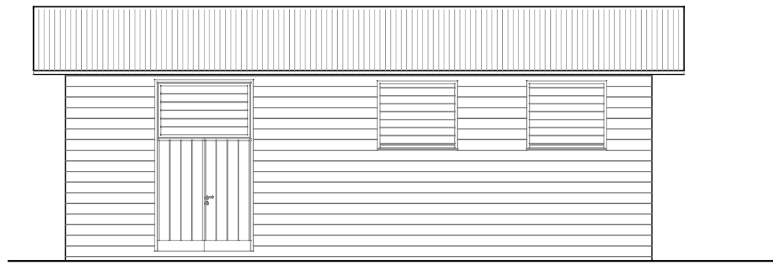
ELEVATION 03
