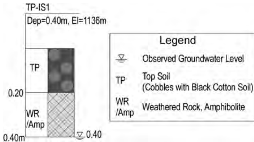
Figure 5.4.16 Columnar Section of TP-IS1
