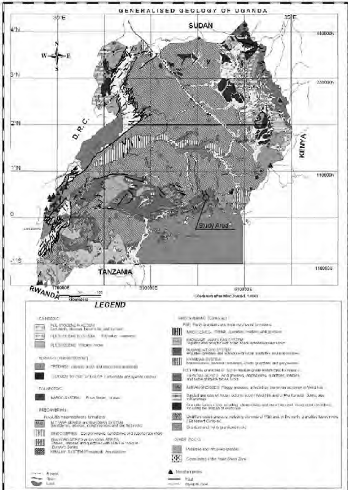
Figure 5.4.2 Geological Map of Uganda
