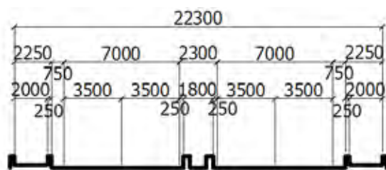
Figure 6.4 Cross Section for Segment-3
