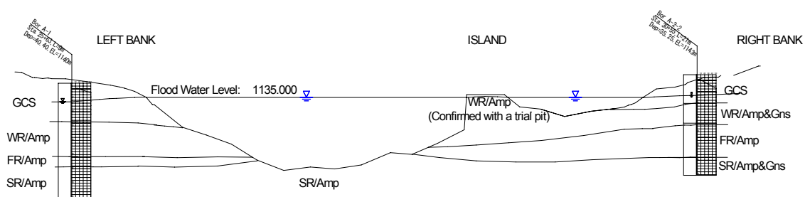
Figure 6.12 Assumed Geological Profiles
