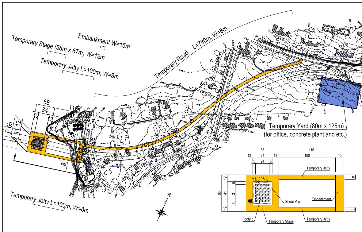
Figure 7.3 Location of Temporary Road and Yard at Njeru side
