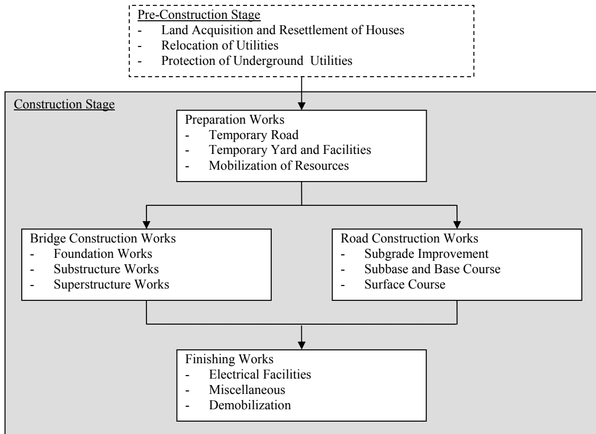
Figure 7.1 Construction Method of the Proposed Nile Bridge
