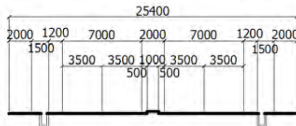
Figure 6.3 Cross Section for Segment-1
