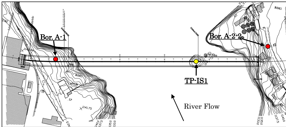
Figure 6.10 Location of Drilling and Trial Pit
