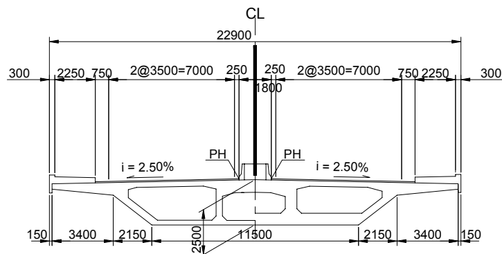
Figure 6.16 Typical Cross Section of the New Nile Bridge
