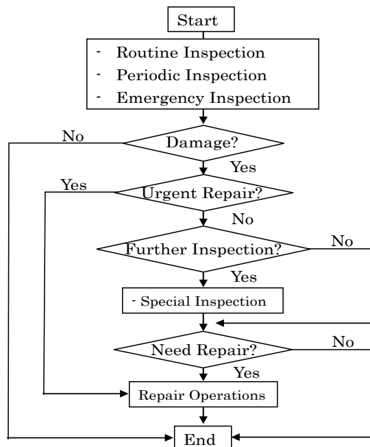
Figure 8.1 Procedure of Maintenance (Repairs) Operations
