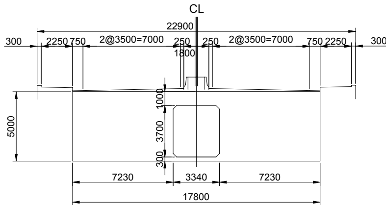
Figure 6.19 Typical Cross Section of the Semi-Underground Beam
