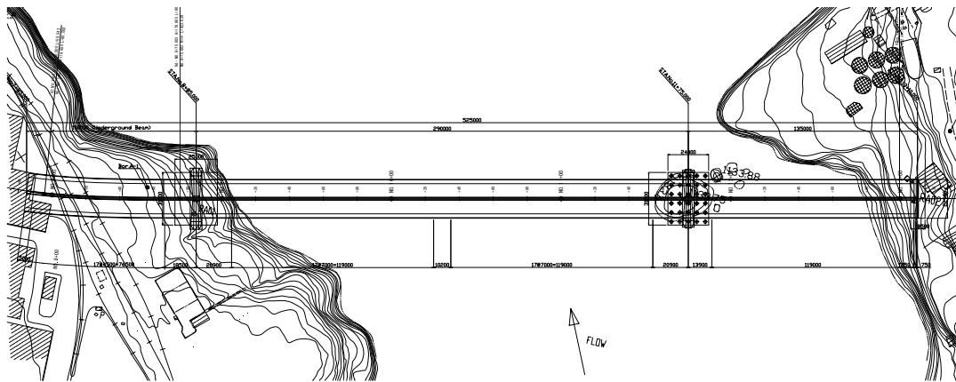
Figure 6.15 Plan of the New Nile Bridge
