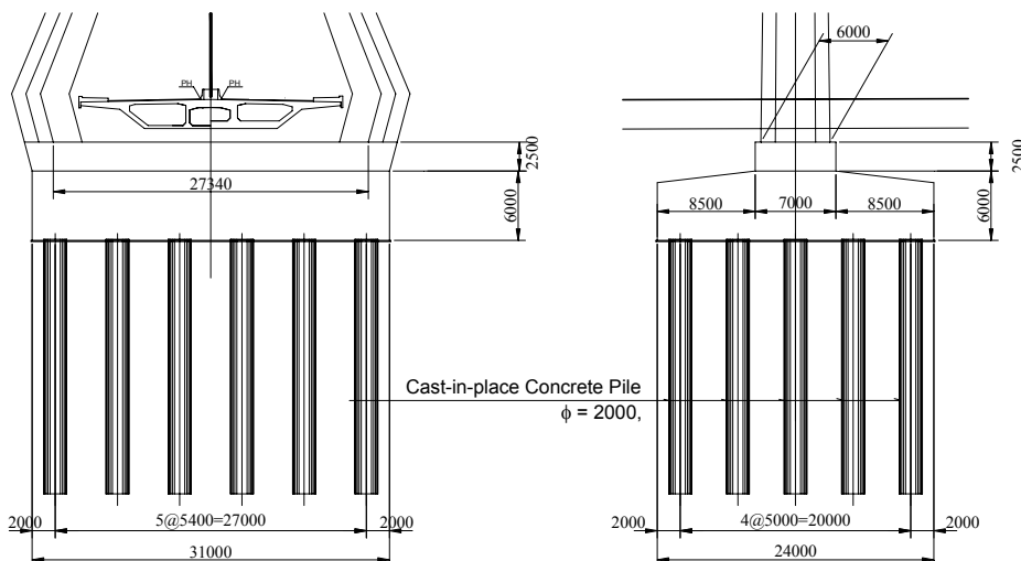
Figure 6.18 Arrangement of Pile for P2
