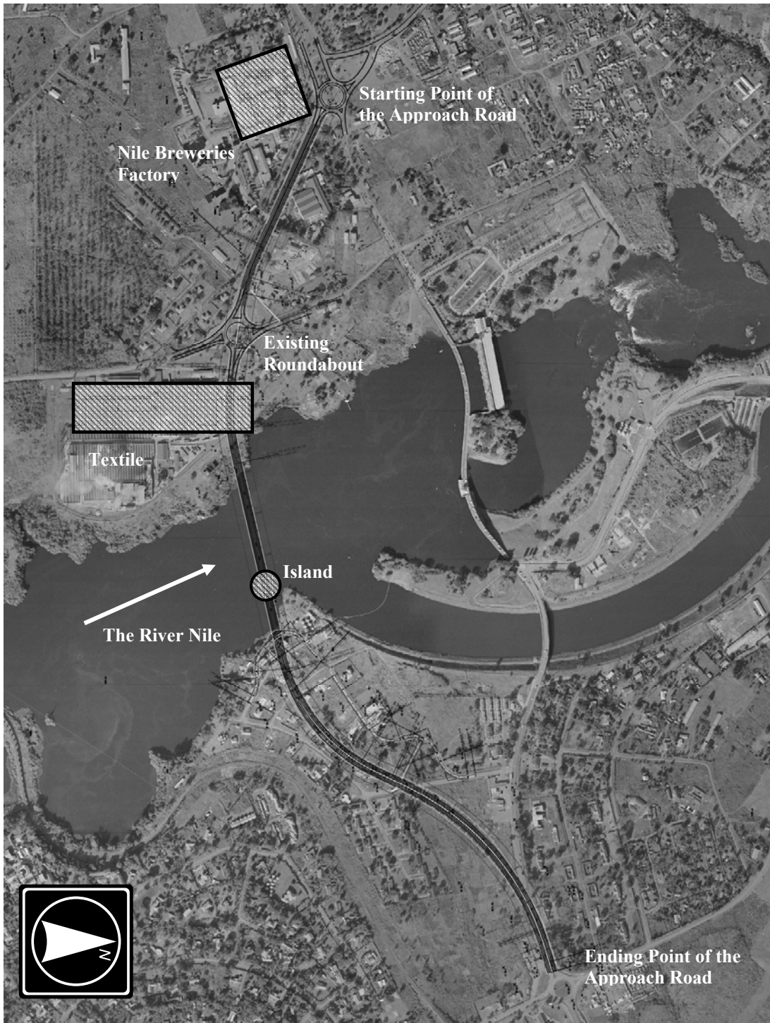
Figure 6.1 Outline of Horizontal Alignment Design
