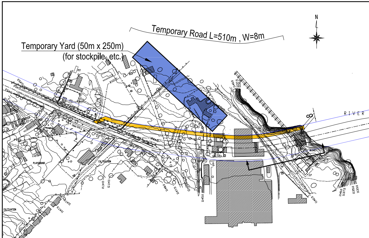
Figure 7.2 Location of Temporary Road and Yard at Njeru side
