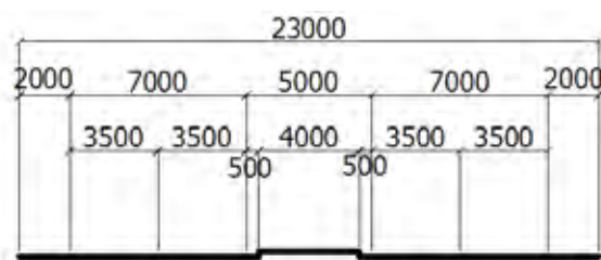
Figure 6.5 Cross Section for Segment-5
