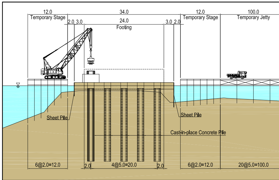
Figure 7.4 Methodology for the Construction of the Foundation for the Jinja Side
