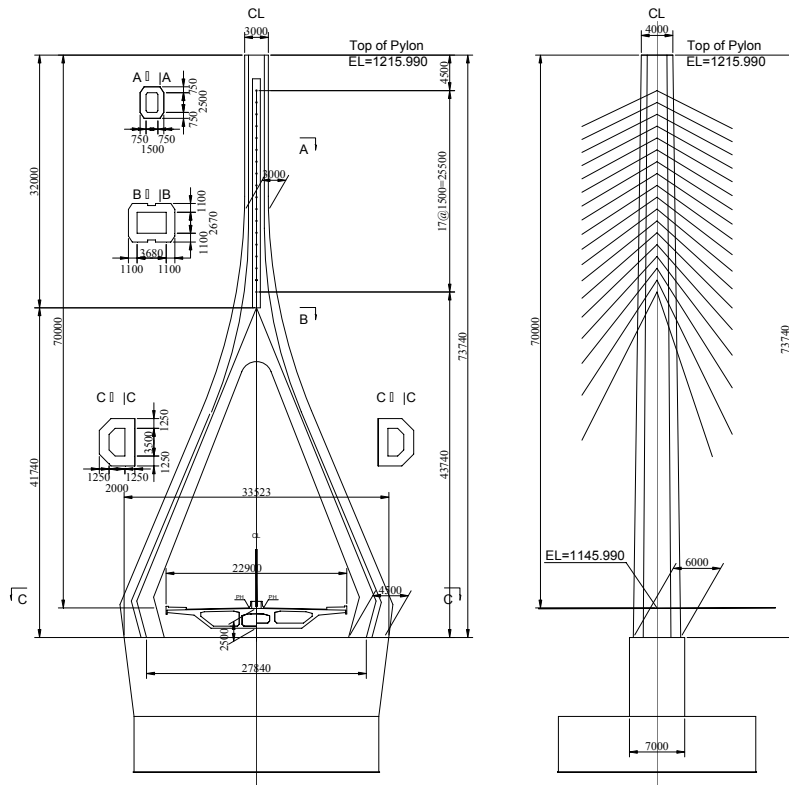
Figure 6.17 General View of the Pylon (P1)
