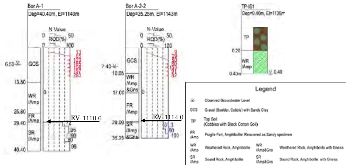
Figure 6.10 Location of Drilling and Trial Pit
