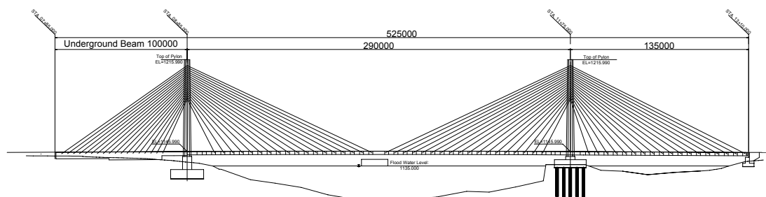
Figure 6.14 Profile of the New Nile Bridge
