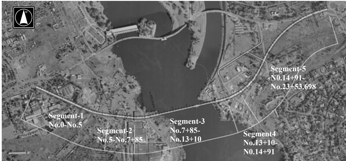
Figure 6.2 Segments for Cross Section
