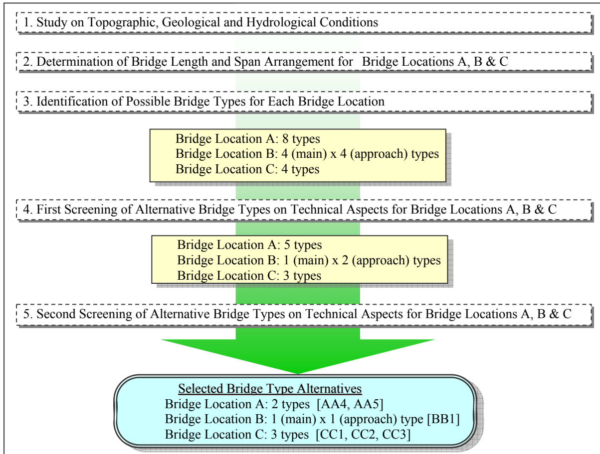
Figure 3.7 Flow Chart for Selecting Optimum Bridge Types for Bridge Locations A, B & C
