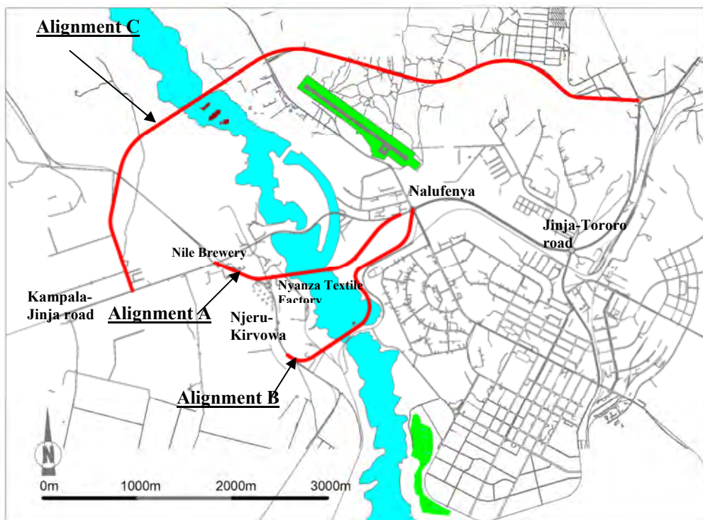
Figure 3.1 Base Alignment Alternatives
