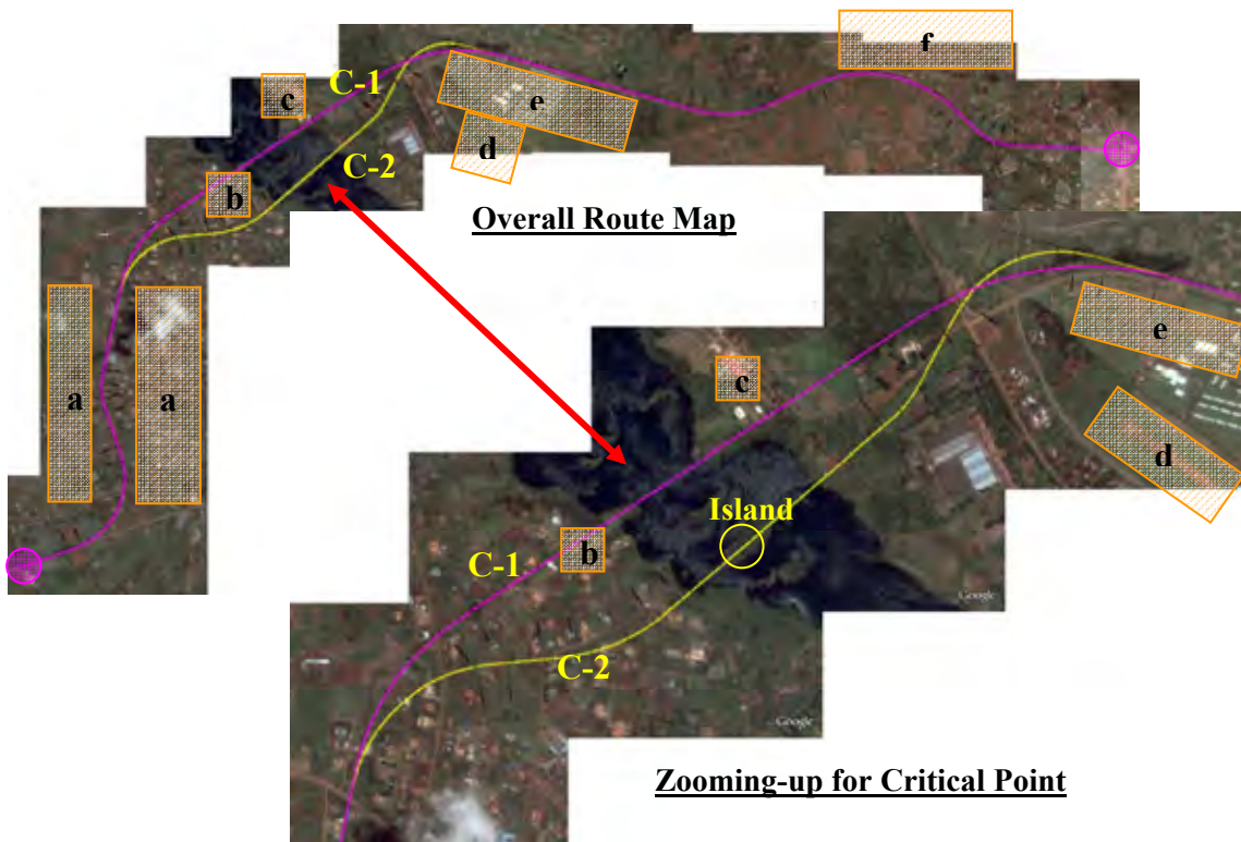
Figure 3.5 Alignment and Bridge Location of Alternatives C-1 and C-2
