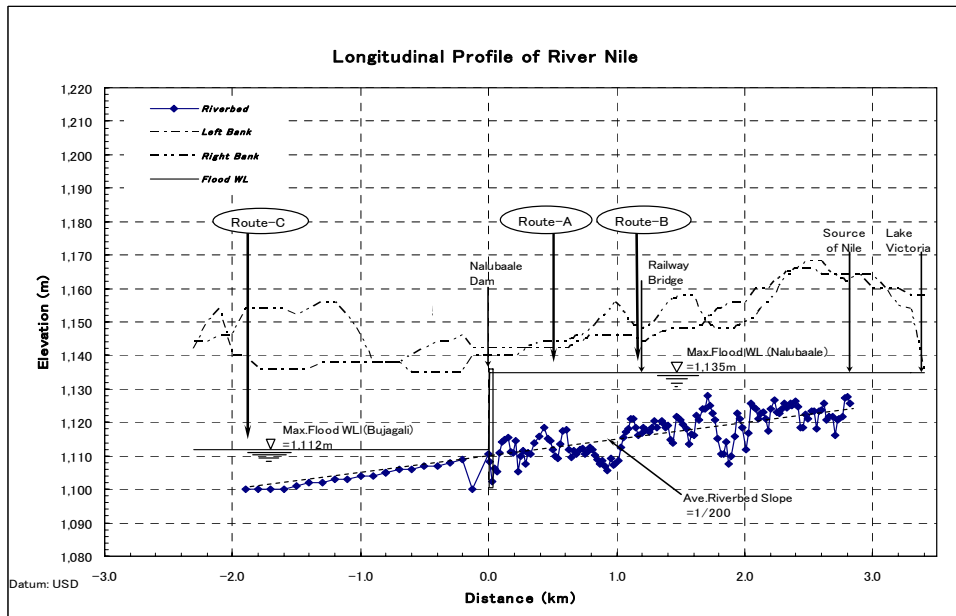
Figure 5.2 Longitudinal Profile
