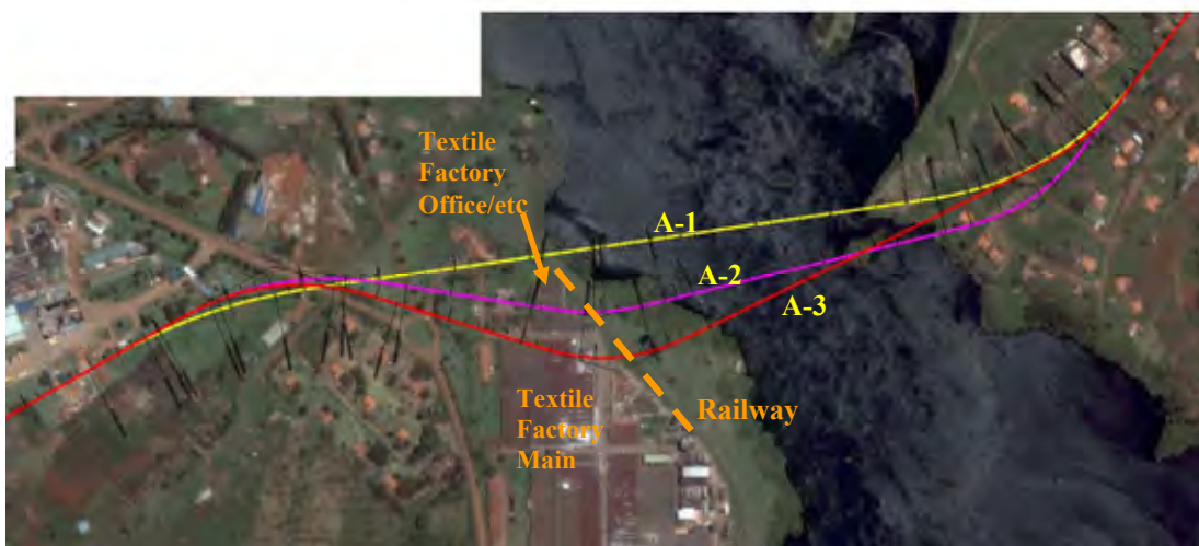
Figure 3.3 Alignment and Bridge Location Alternatives A-1, A-2 and A-3
