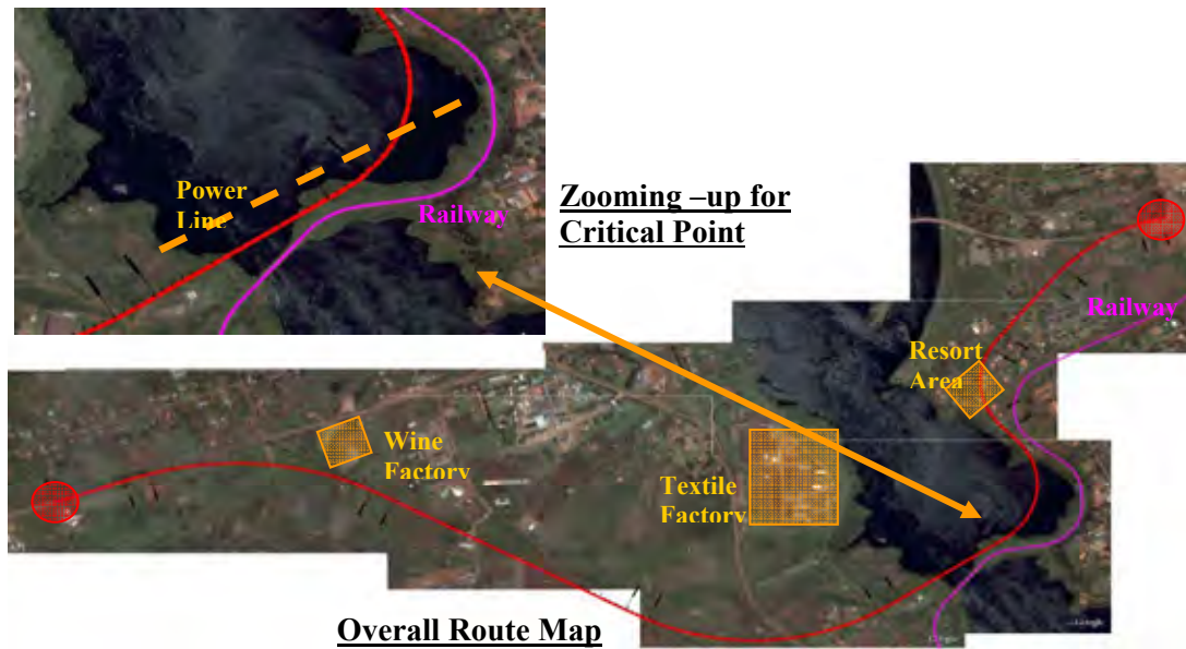
Figure 3.4 Alignment and Bridge Location Alternative B
