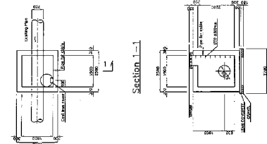
No.3 Plan
