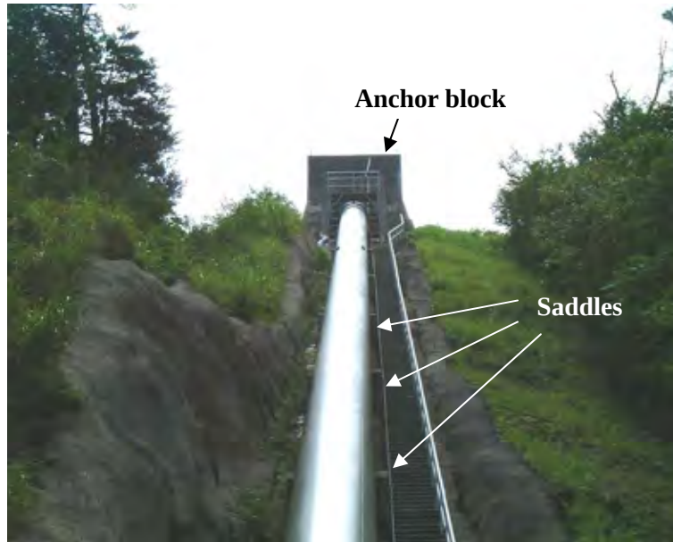
Photograph 48-3 Penstock, Anchor Block and Saddles
