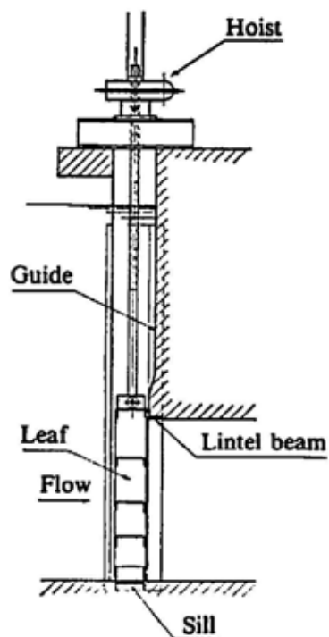
Fig. 50-7 Slide Gate
