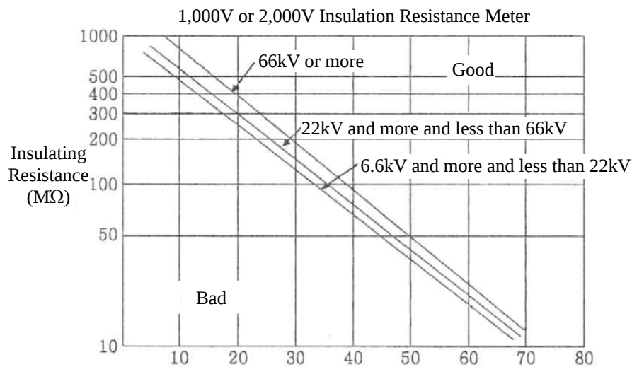
Fig. 183-1 Allowable Insulating Resistance for Transformer
