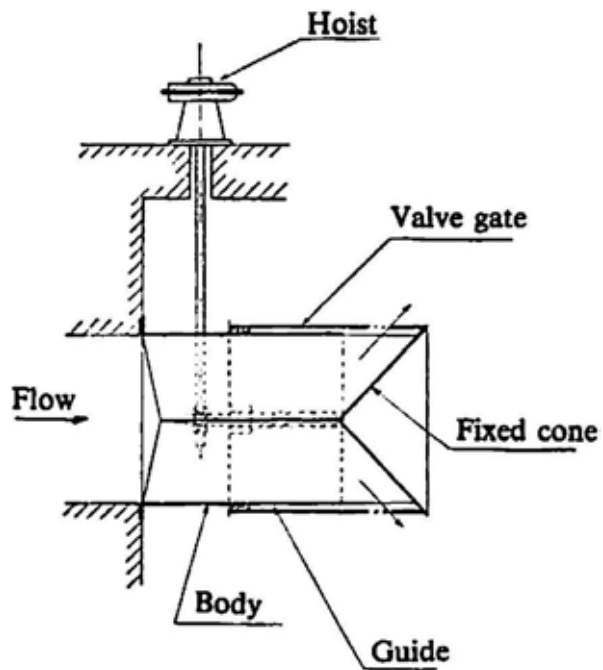
Fig. 50-13 Cone Valve
