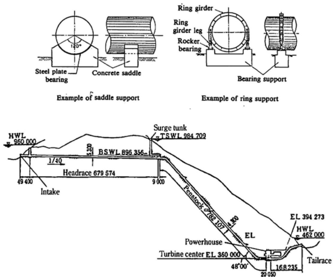
Fig. 48-4 Embedded Type Penstock
