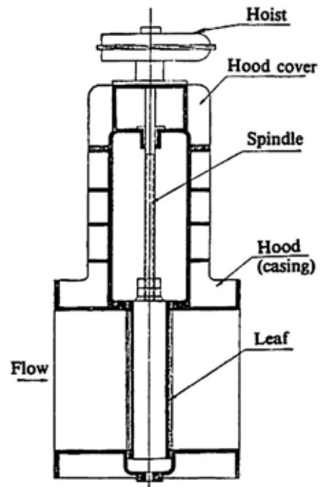
Fig. 50-14 Gate Valve
