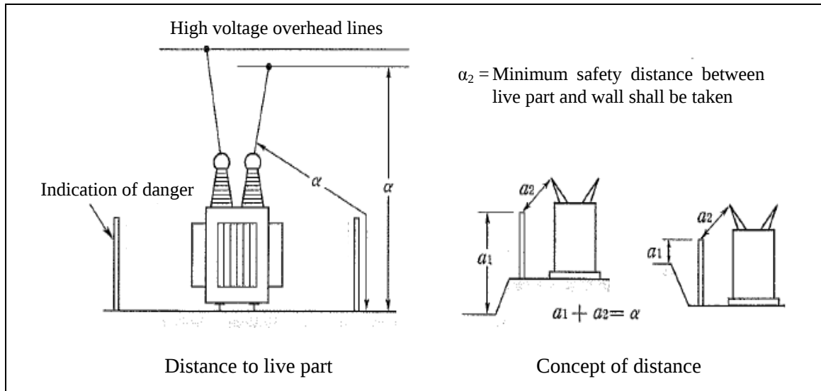
Fig. 64-2 Installation of High Voltage
