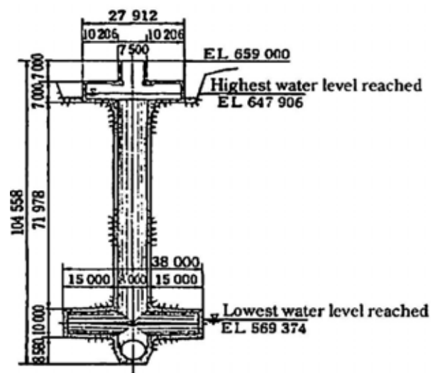
Fig. 47-4 4. Chamber Type
