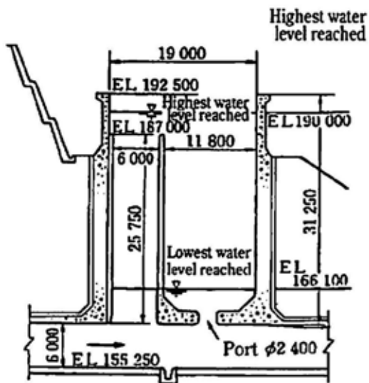
Fig. 47-3 3. Differential Type
