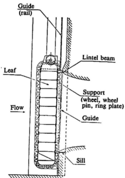
Fig. 50-5 Caterpillar Gate
