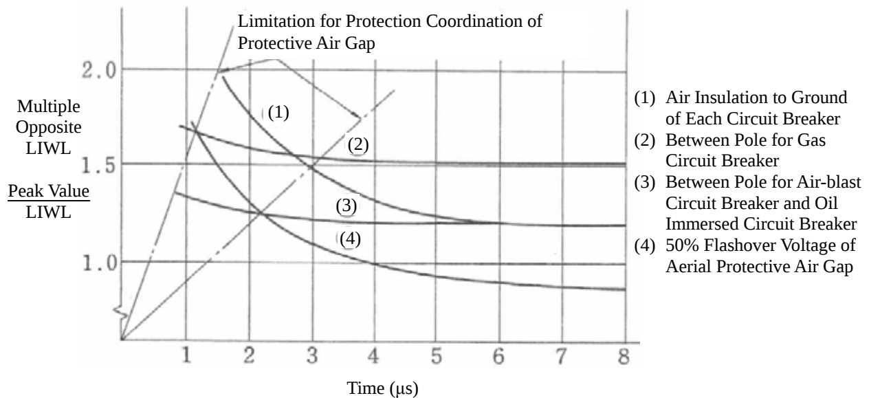
Fig. 95-1 Comparison of V-t Characteristics for Circuit Breaker
