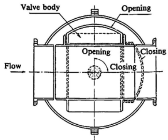
Fig. 50-16 Rotary Valve
