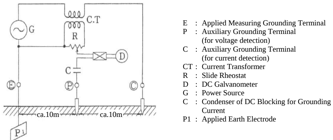
Fig. 181-1 Measuring Circuit for Direct Reading Earth Resistance Meter
