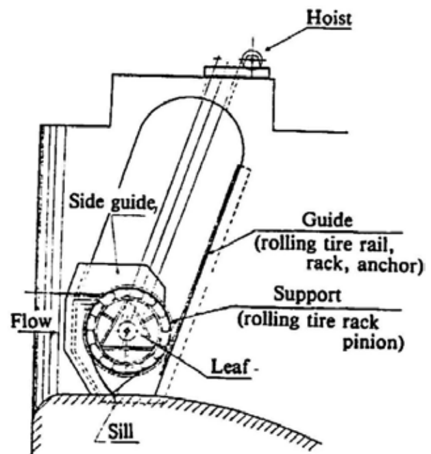
Fig. 50-6 Rolling Gate
