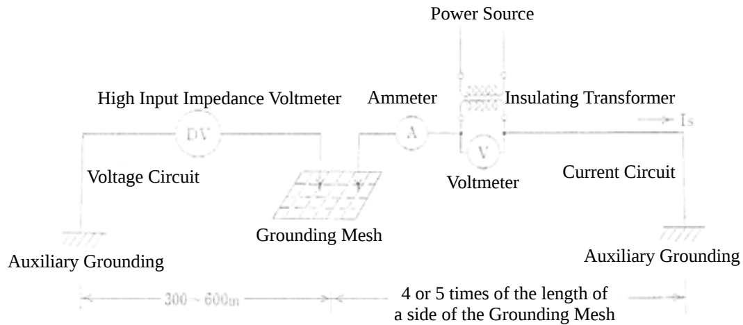
Fig. 181-2 Measuring Circuit for the Fall of Potential Method
