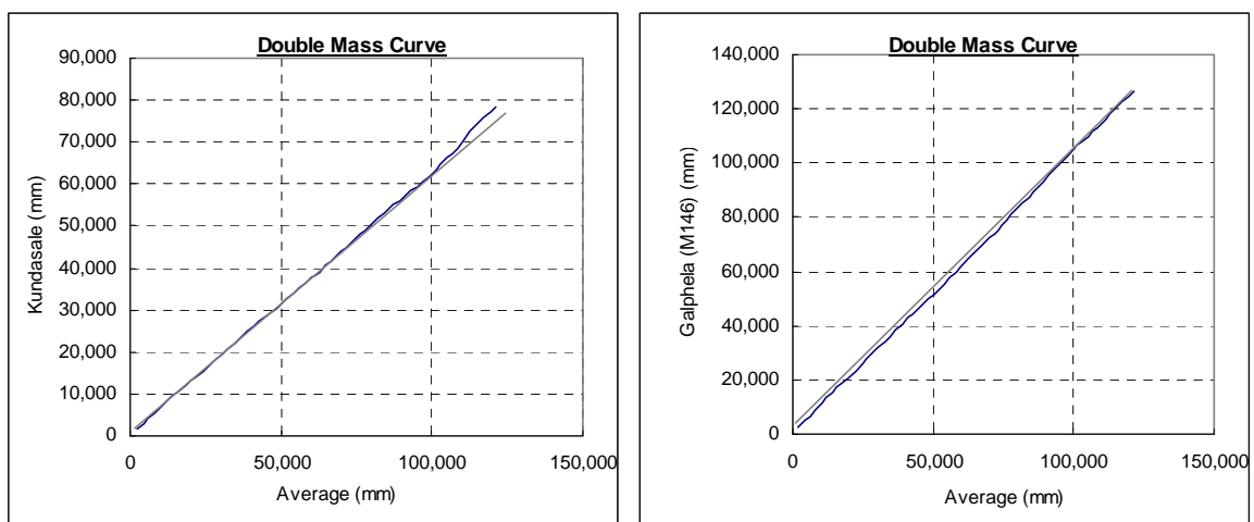
Figure 3 Double Mass Curve Analysis of Kundasale and Galphela after Corrected
