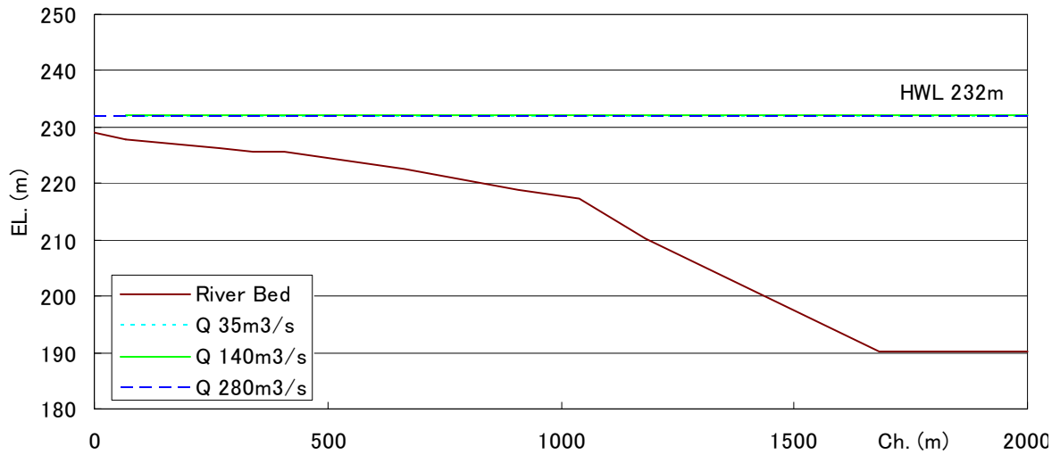
Figure 5 Difference of water level (HWL)
