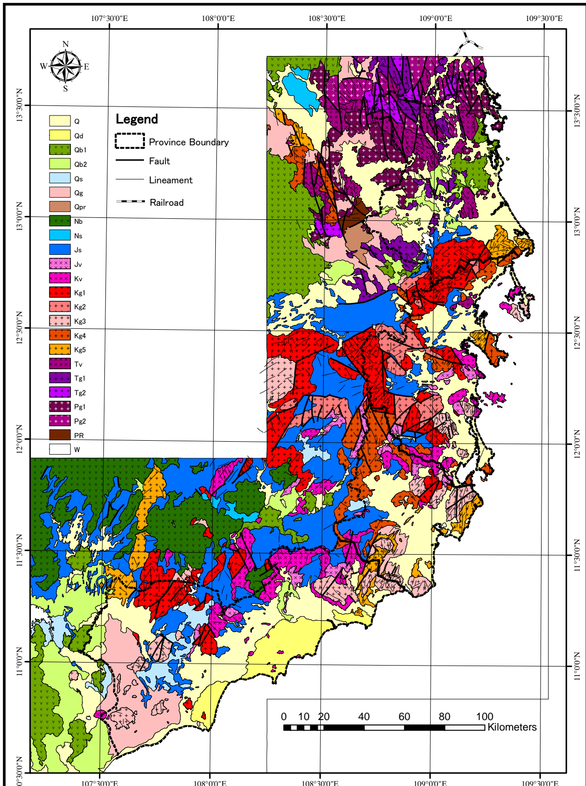
Figure 2.1.12 Geological Map in the Study Area
