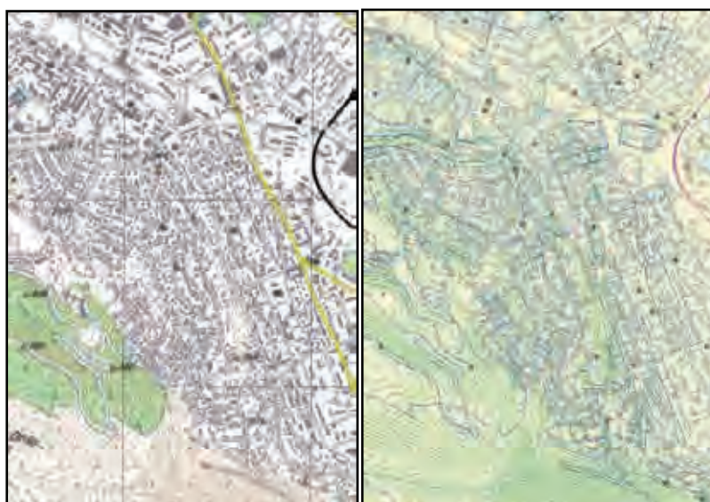
Fig 42 : Comparison of topographic map (left) and GIS database
