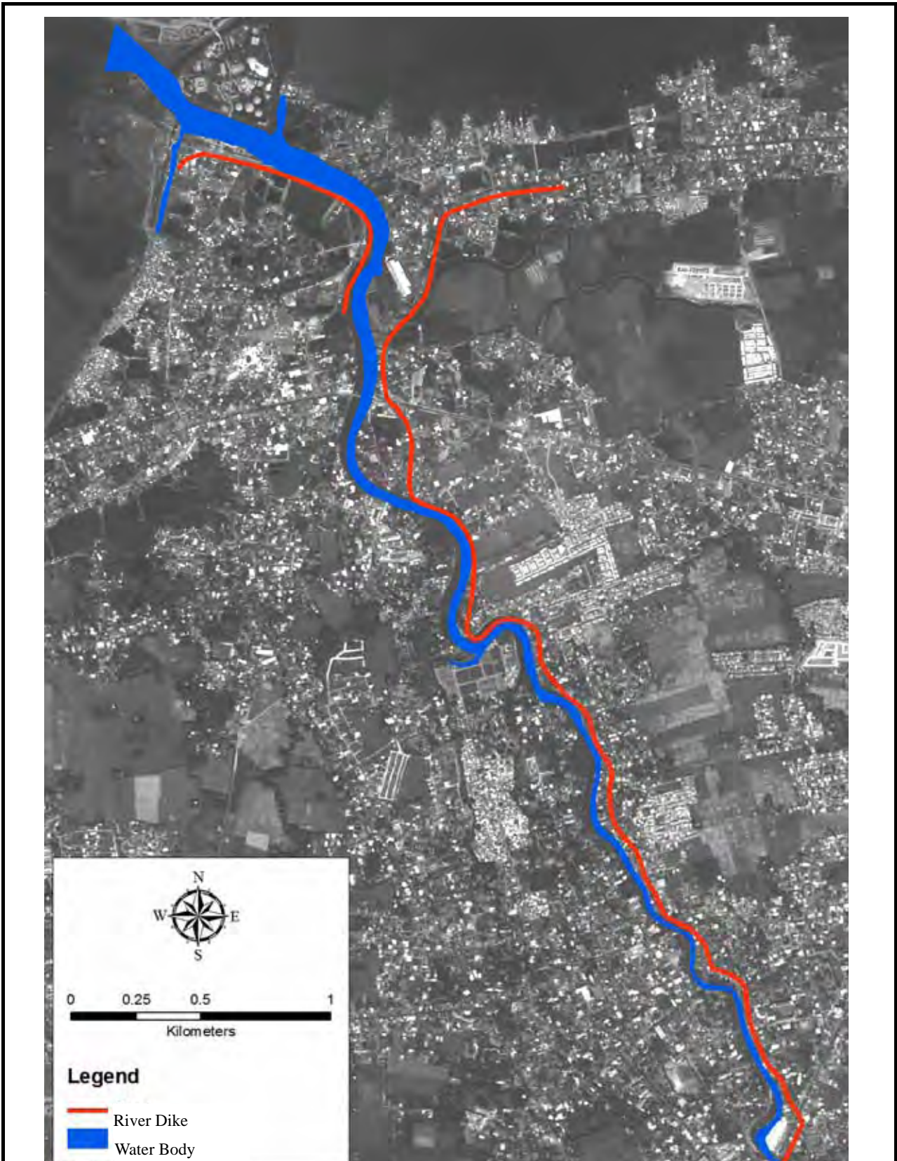
Fig. 5.1 Layout of Existing River Dike along Imus River
