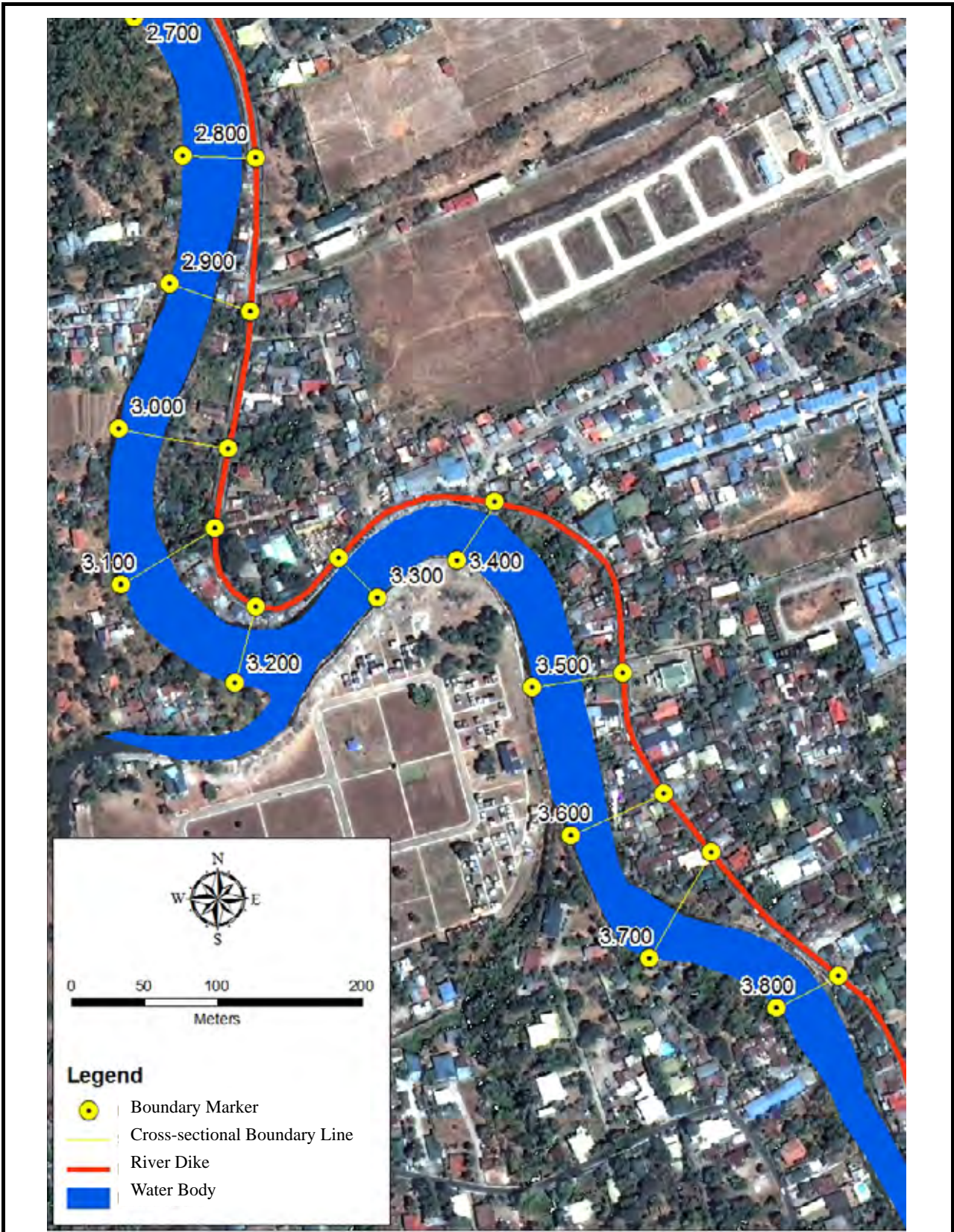
Fig. 5.2 (4/7) Division of River Area for Imus
