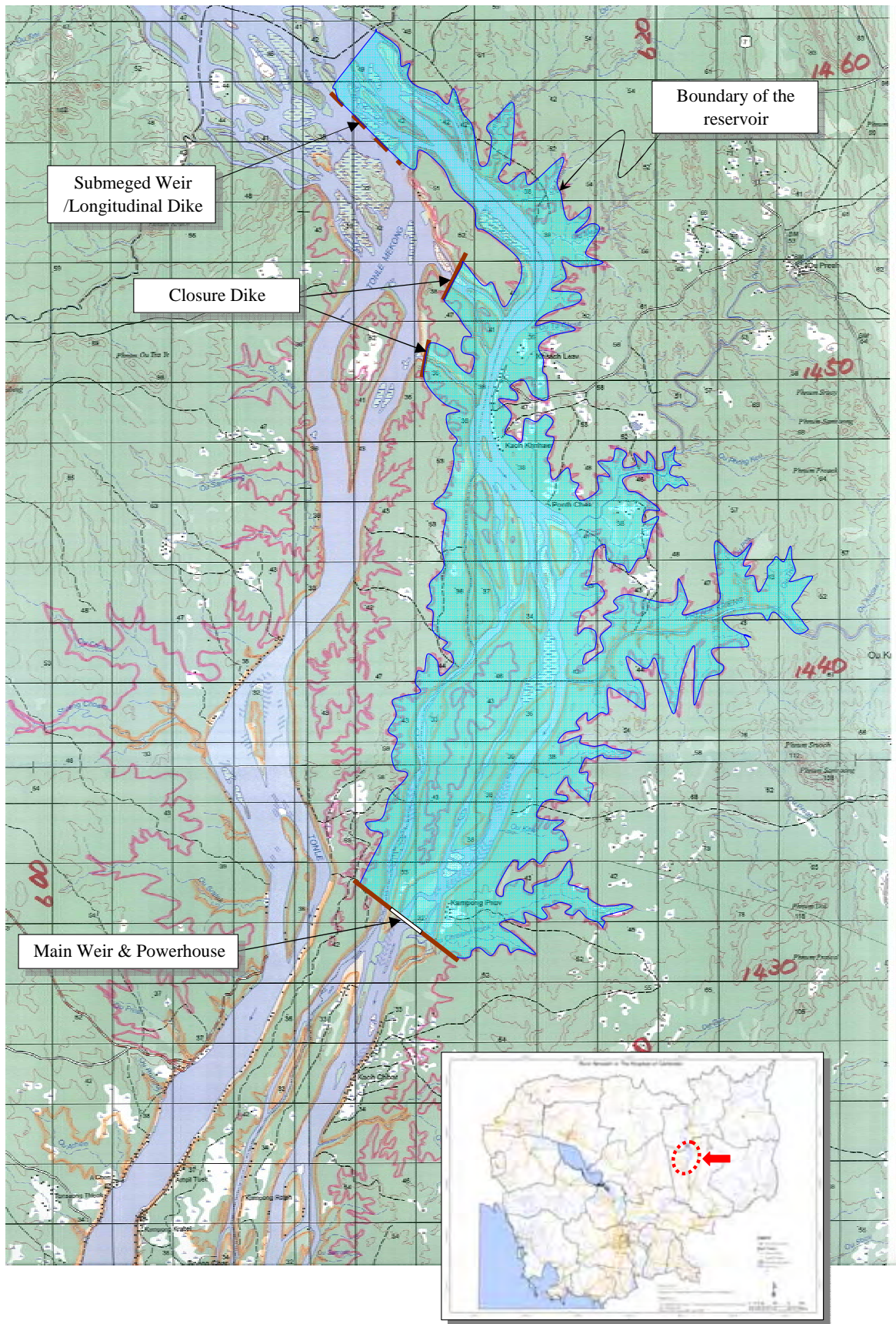
D-3: An example of using a part of river course for power generation in the Mekong Mainstream
