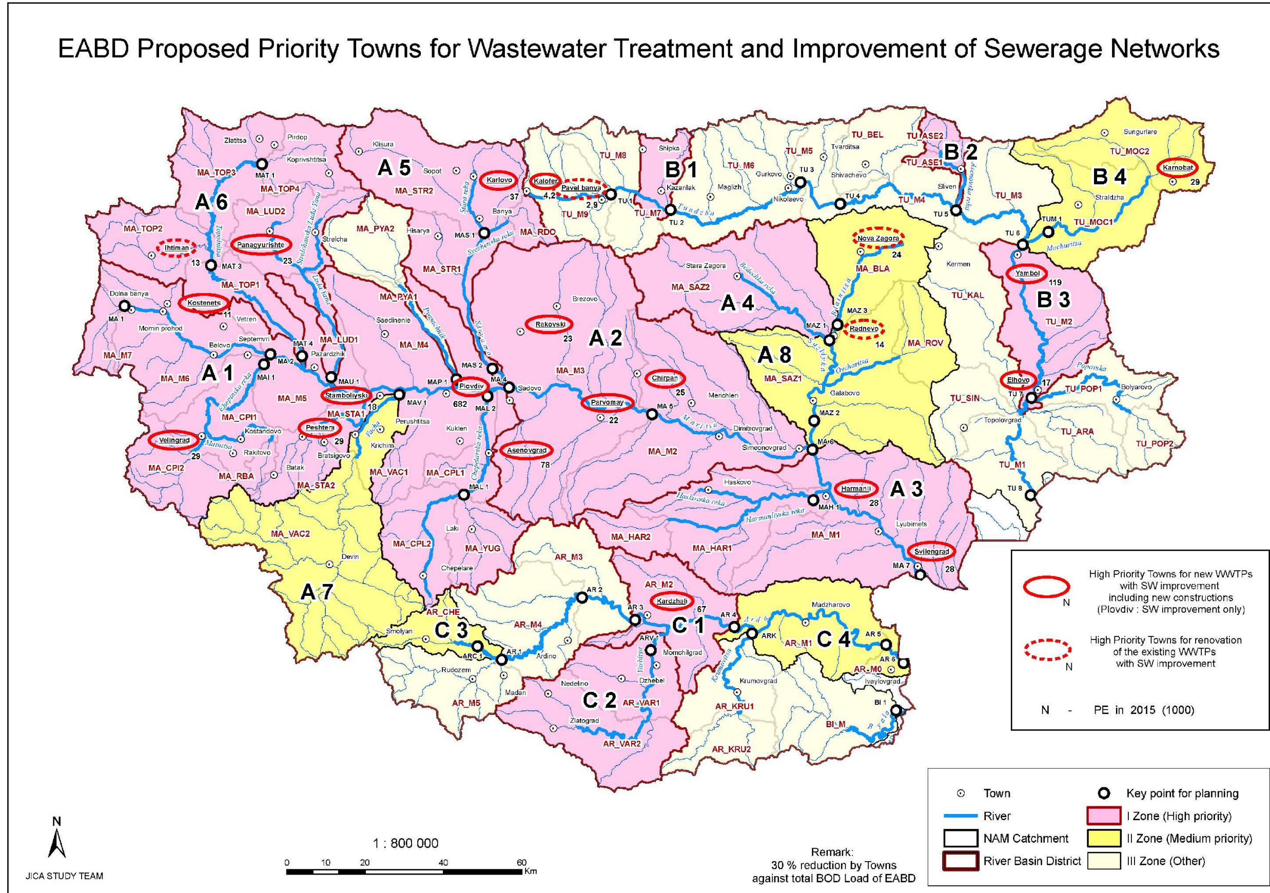
Figure 8 EABD Proposed High Priority Towns for Wastewater Treatment and Improvement of Sewerage Networks
