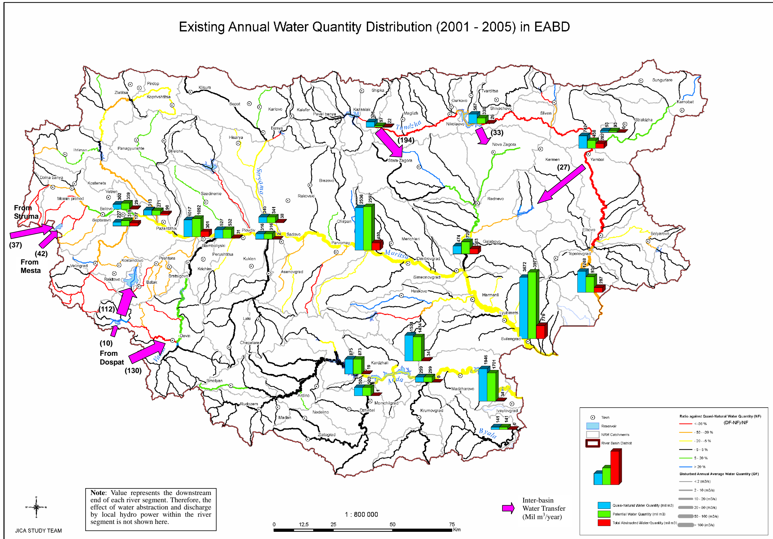
Figure 1 Water Balance including Inter-Basin Water Transfer in EABD (Average in 2001 – 2005)
