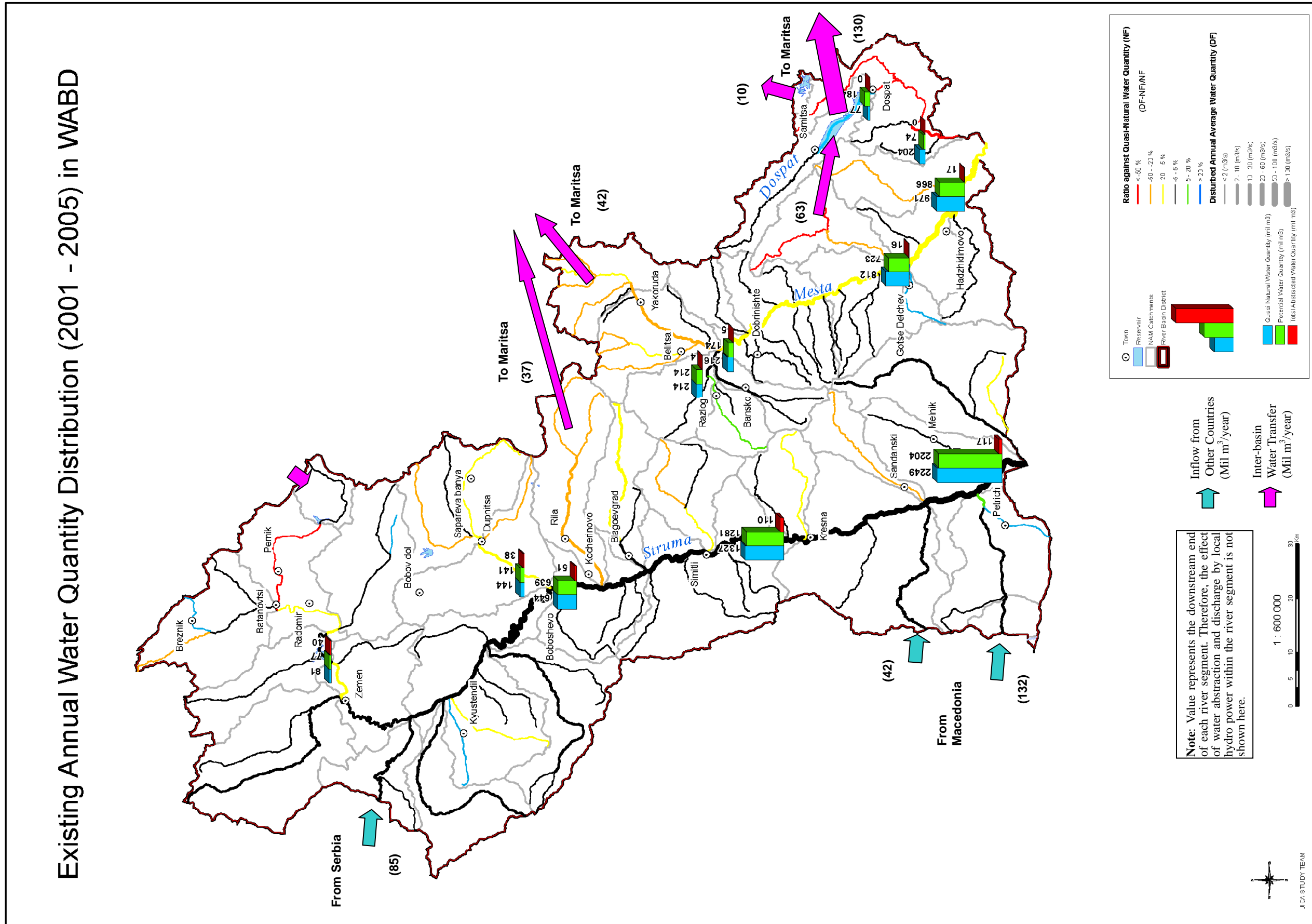
Figure 2 Water Balance including Inter-Basin Water Transfer in WABD (Average in 2001 – 2005)
