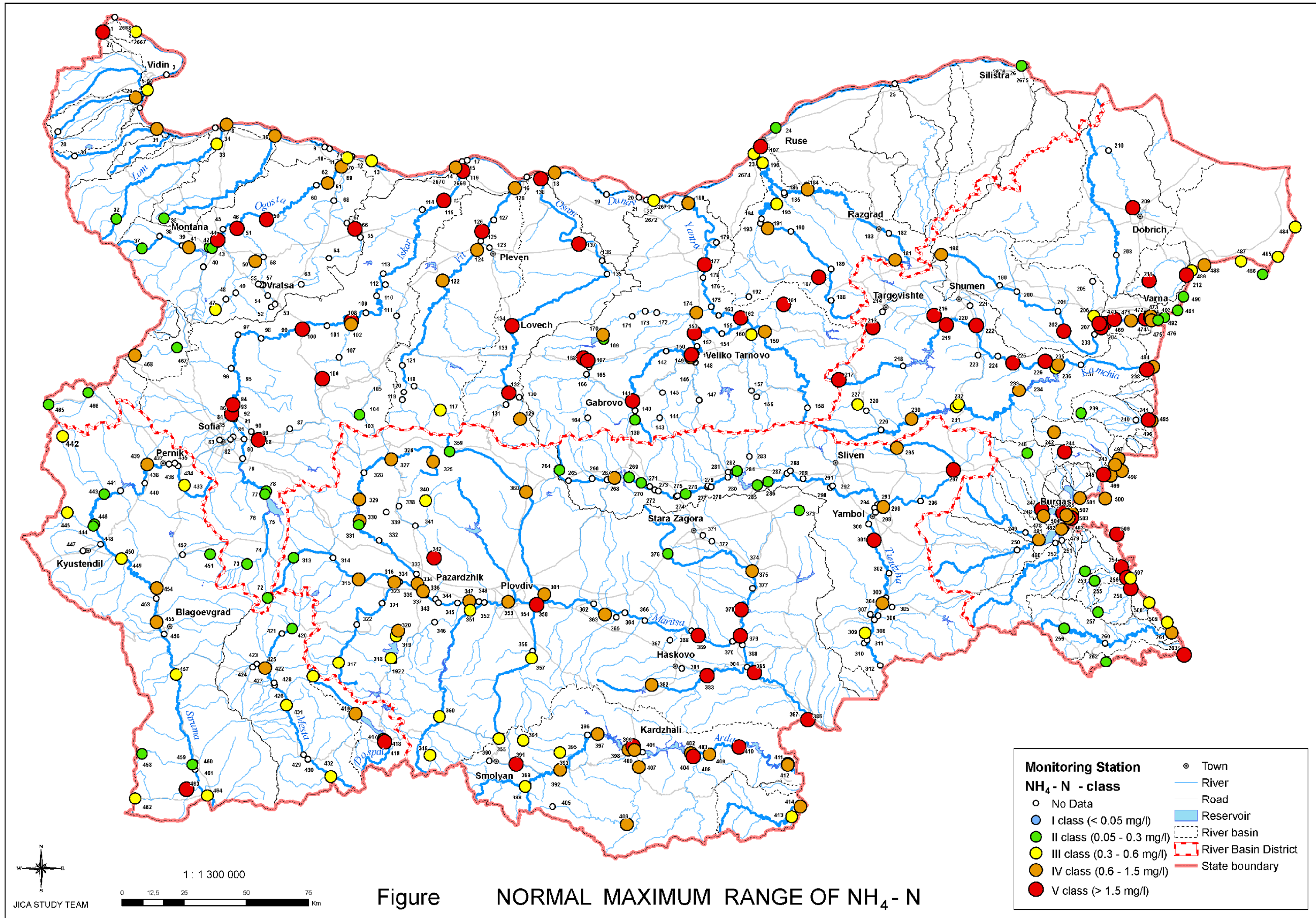
Figure 4 Normal Maximum Range of NH 4 -N
