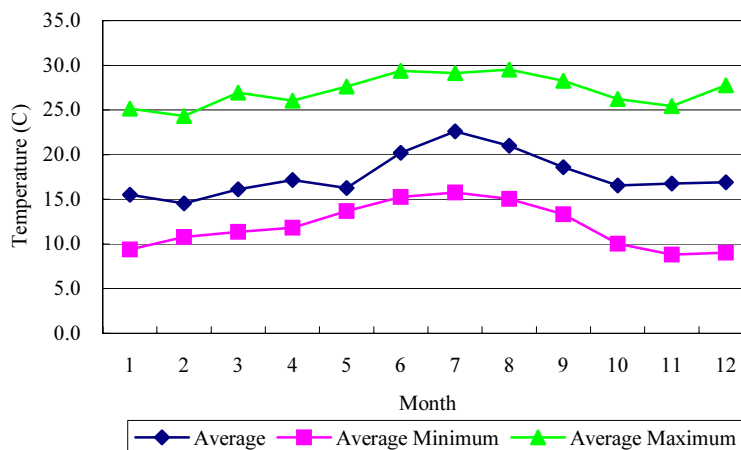
Figure 3.4 Monthly Temperature (NWRA-A, 1989-1997)
