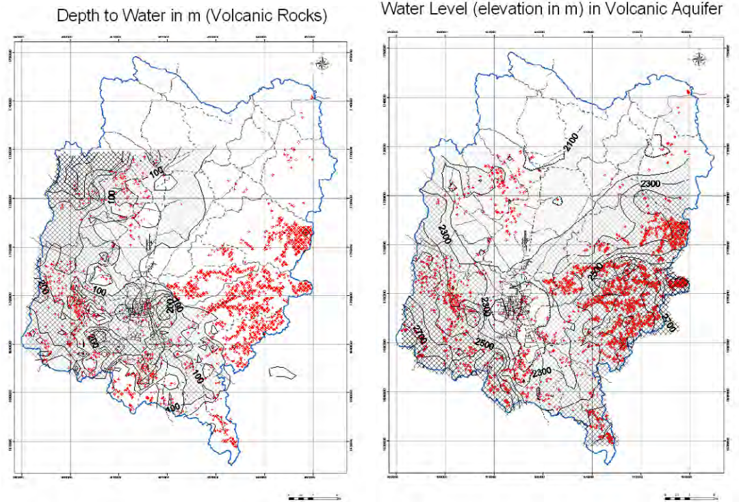
Figure 3.19 Water Level (Volcanic Rocks)
