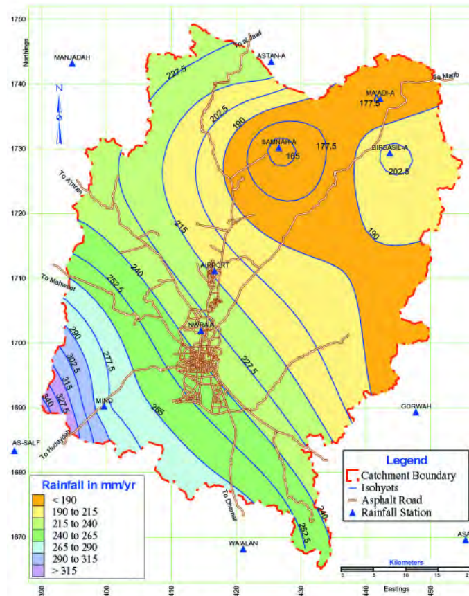
Figure 3.6 Isohyet Map of the Sana'a Basin
