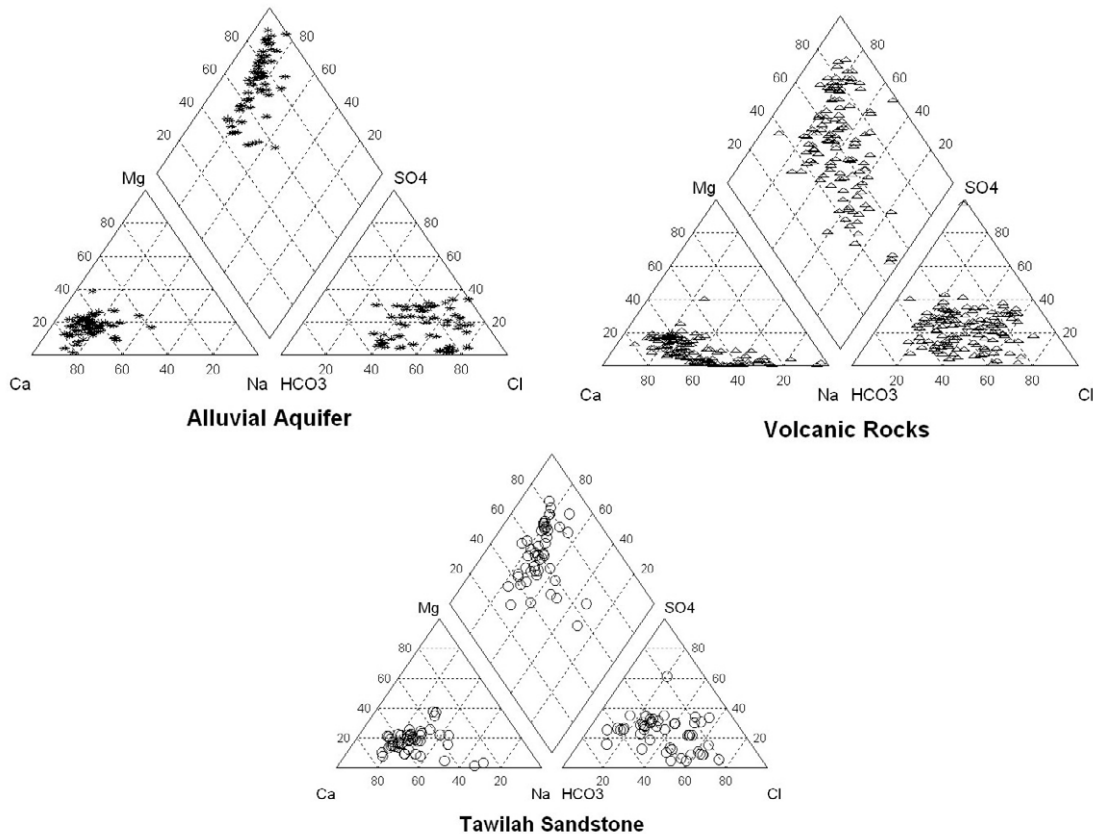
Figure 3.26 Piper Diagrams of Groundwater in the Sana'a Basin
