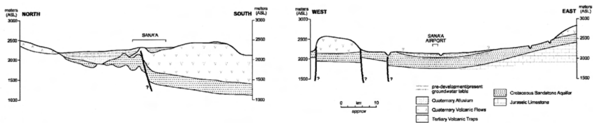
Figure 3.1 Geology in the Sana'a Basin
